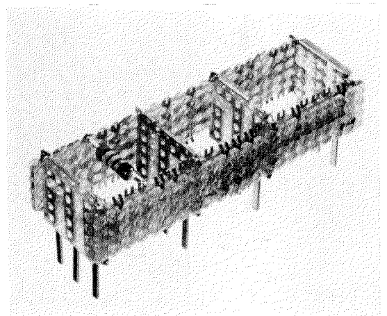
Figure 7—Two side-plate assemblies together with terminal plates make a frame for mounting components.
