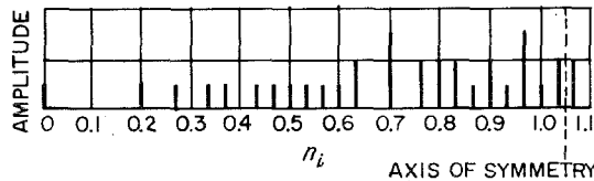
Figure 13—Space positions of elements and their excitation amplitudes for code 6. K = 1, 15/13, 15/11, 3/2, 15/8, \text{ and } 5/2 . D = 15 . A mirror image of the figure exists to the right of the axis of symmetry.
