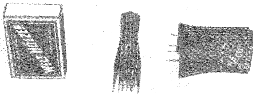
Figure 19—Bridge-connected selenium rectifiers for mounting on printed-circuit boards. The rectifiers are intended for power supplies of television receivers using transistors.
