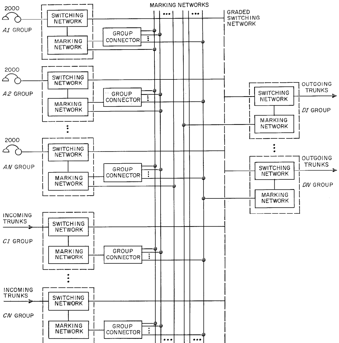
Figure 1—System grouping.
