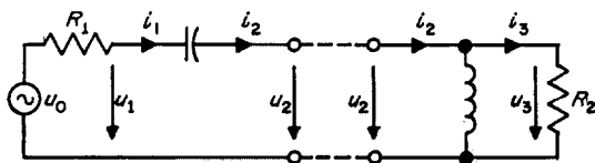
Figure 1—Cascade of 2 time-varying four-poles.
