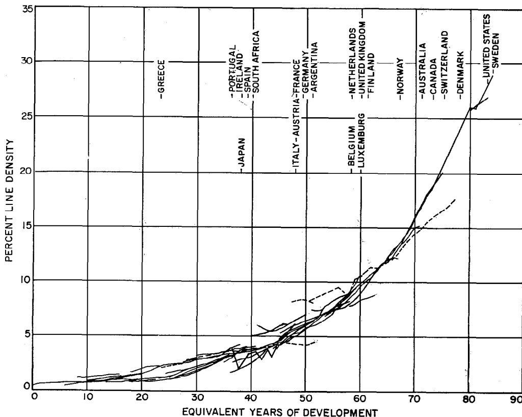
Figure 4—Composite line-density curves for various countries as a function of time in years t and a constant c of relative lag or lead with respect to all others. The development of each country is indicated as of 1 January 1961 [3].
