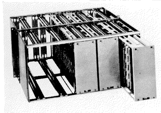
Figure 8—Double-depth subrack.
