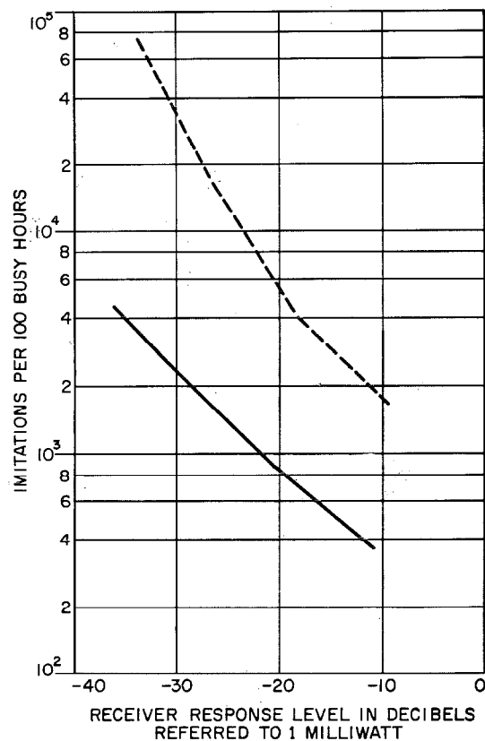
Figure 8—Number of signal imitations as a function of receiver sensitivity. The solid curve was derived by Flowers and Weir [7] and the broken curve by the authors. Refer to Table 2.
