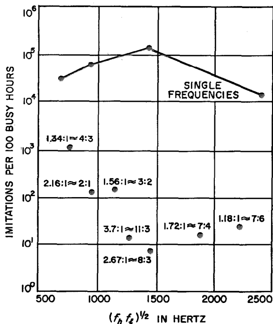
Figure 7—Comparison of protection afforded by single-frequency and 2-frequency tones. The indicated ratios represent f_h/f_l , and are plotted at their geometric means (f_h f_l)^{1/2} in hertz. Receiver ratings were: bandwidth, 150 hertz; sensitivity, -26 decibels referred to 1 milliwatt; and response time, 25 milliseconds. No speech-guard circuit was used.
