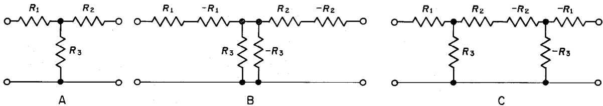
Figure 1—The attenuation of the nonsymmetrical T network at A may be compensated for by the insertion of corresponding negative impedances at B, which may also be accomplished at C by converting to an equivalent \pi network.
