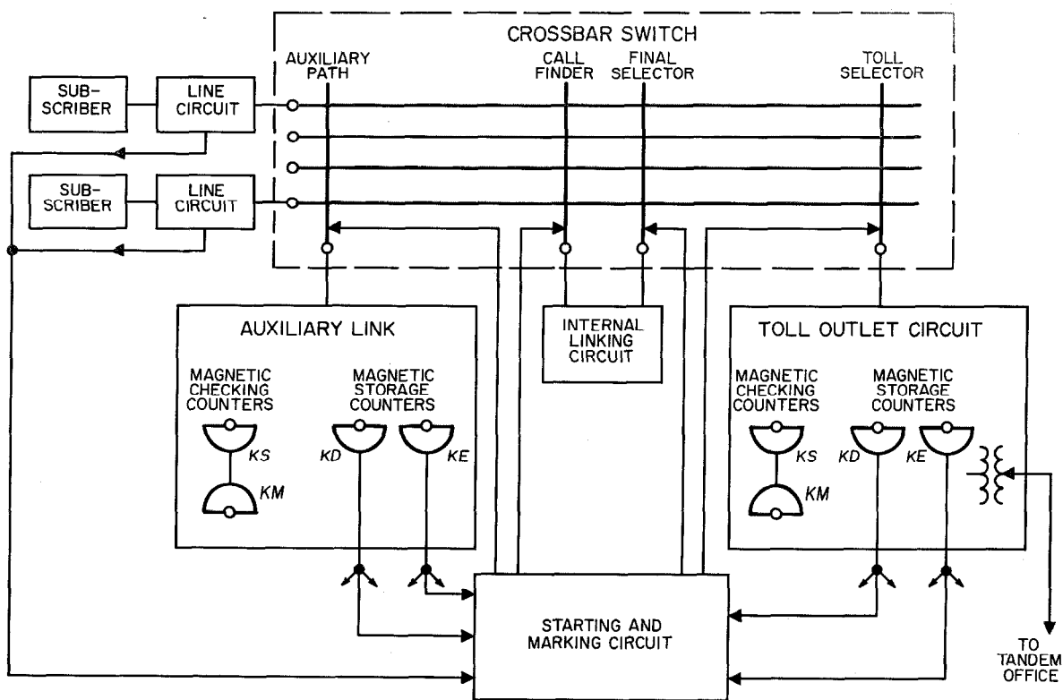
Figure 2—Starting and marking of junctions in a crossbar exchange.
