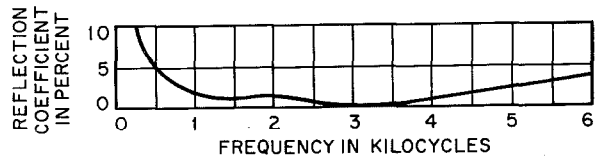
Figure 24—Reflection coefficient of the repeater as derived from Figure 23.
