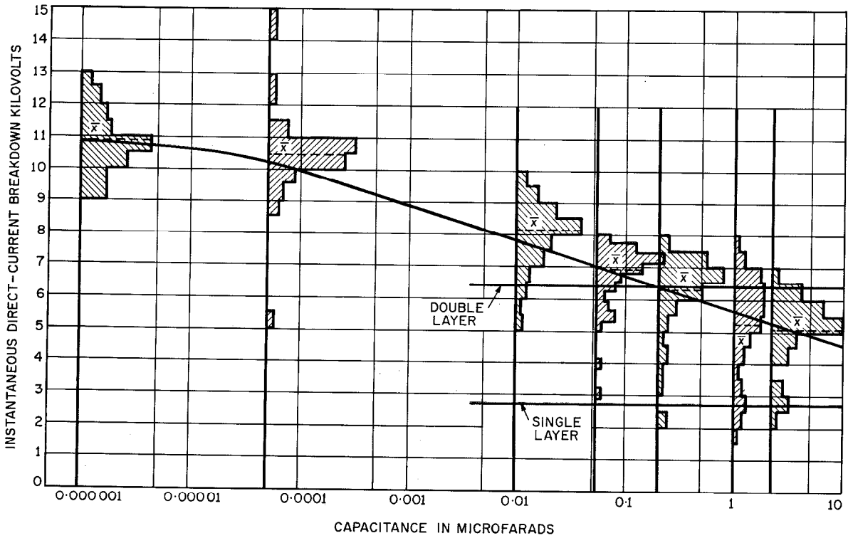
Figure 6—Instantaneous-breakdown-voltage histograms as a function of capacitance (area). Values of capacitance tested were 0.000001 (sphere gap), 0.0001, 0.01, 0.05, 0.2, 1, and 3 microfarads. All had 3 layers of 8-micron rag-based tissue impregnated with mineral oil. Each histogram is based on 100 results.
