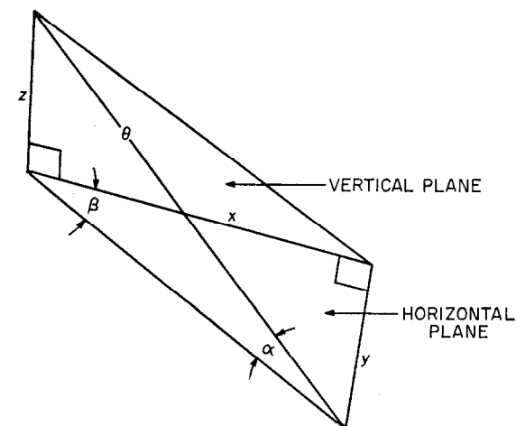
Figure 7—Vector diagram.
