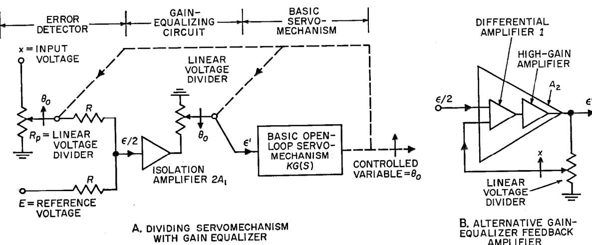
Figure 2—Gain-equalized servomechanism for determination of reciprocals.
