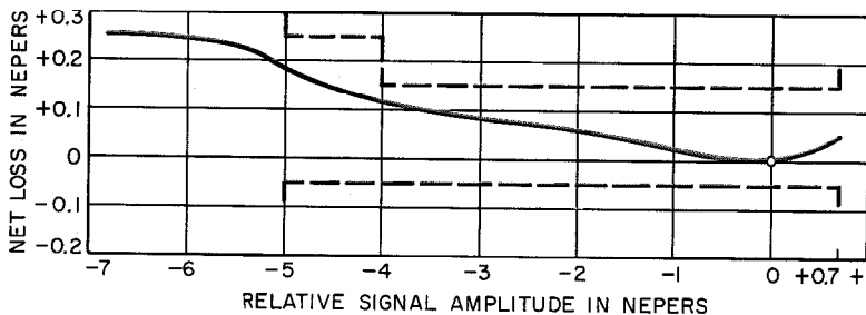
Figure 8—Compressor amplitude dependence. Dashed lines give the tolerance.
