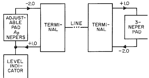
Figure 9—Loop loss as a function of noise level. Input and output levels in nepers are shown on the block diagram: Loop loss, A_i = 3 - A_p nepers.
