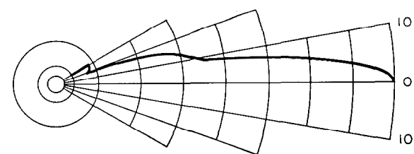
Figure 11—Vertical-plane radiation pattern of transmitting horn.
