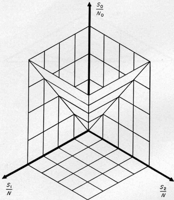
Figure 6—Three-dimensional characteristic of selector combiner.
