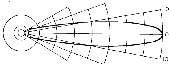
Figure 10—Horizontal-plane radiation pattern of transmitting horn.
