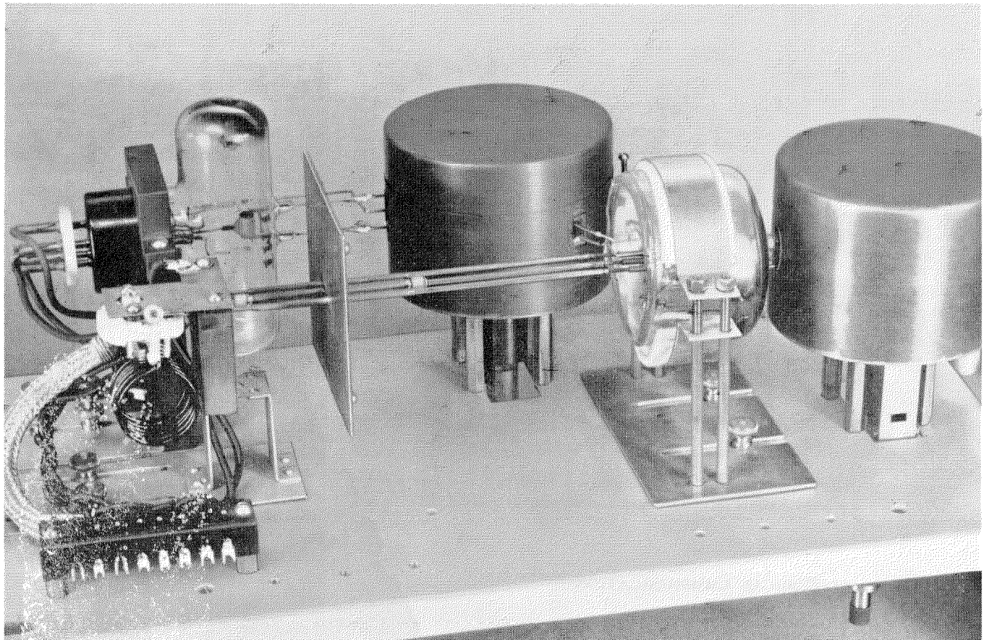
Figure 5—The frequency-converter portion of the receiver. The diode mixer is coupled to the input cavity at the right and to the local-oscillator cavity at the center.
