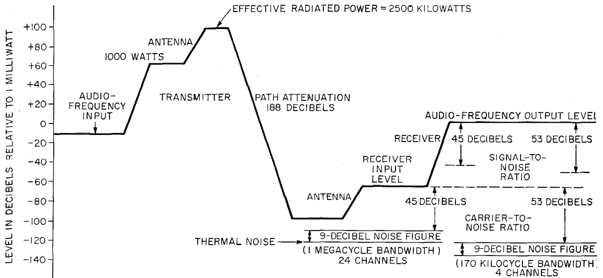
Figure 8—Power-level diagram.
