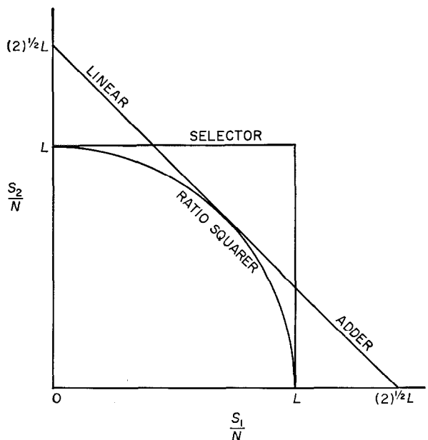
Figure 10—Characteristics of diversity combiners for an output signal-to-noise ratio of L .
