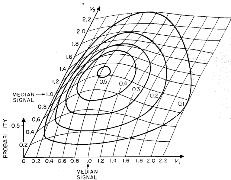
Figure 12—Two-dimensional Rayleigh distribution.
