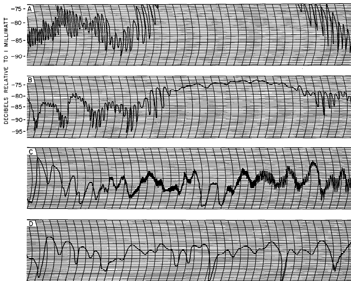
Figure 12—Recordings showing effect of airplane reflection when using, A and C = wide-beam 10-foot (3-meter) antenna, B and D = narrow-beam 28-foot (8.5-meter) antenna. Horizontal time scale = 2 divisions per second.
