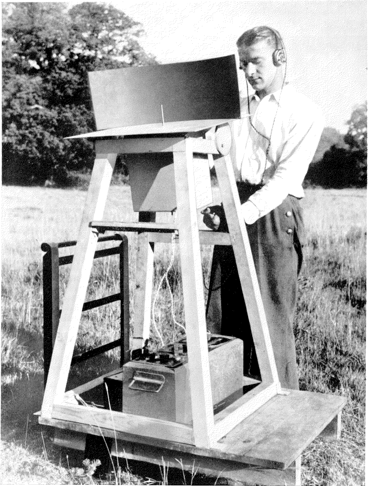
Figure 9—Receiver used for checking the transmitter and its radiating horn.
