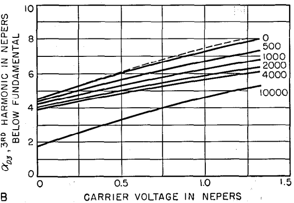
Figure 3—Measured distortion attenuation in a germanium modulator as a function of the carrier voltage level for the indicated values of R_s in ohms. The dashed curve is for 10 000 ohms in parallel with the rectifiers.
