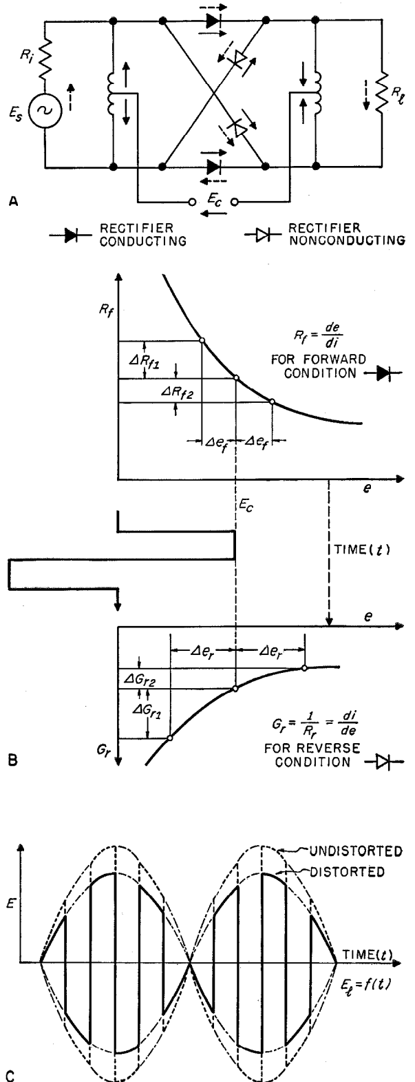
Figure 2—Generation of cubic distortion in conducting and blocking rectifier elements.
