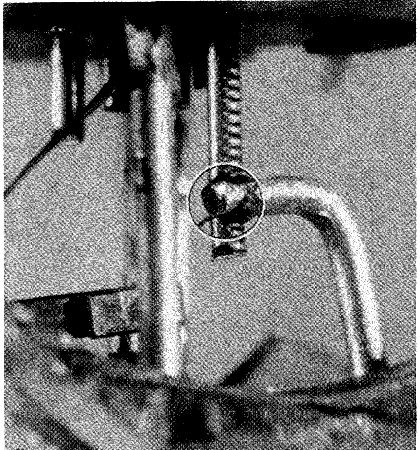
Figure 14—Piece of weld splash that may break away under vibration and cause noise. Also, the cathode ribbon is too tight.
