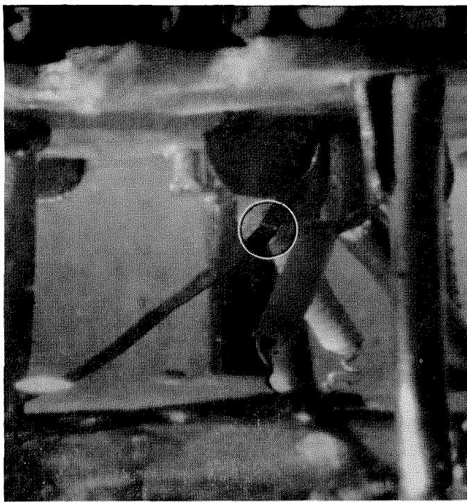
Figure 6—This overly tight cathode ribbon has broken after a few hours of testing.
