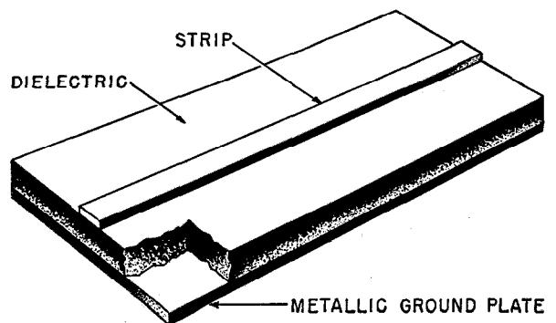
Figure 1—Microstrip line.
