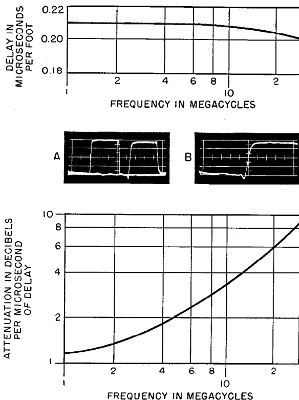
Figure 2—Type- A delay cable. The delay-frequency characteristic is shown at top and the attenuation-frequency relation at the bottom. Oscillograms are for a 1-microsecond pulse through 6 feet (1.8 meters) of cable with timing divisions of 0.3 microsecond at A and 0.1 microsecond at B . At A , the input pulse is at the left and its output form is at the right.
