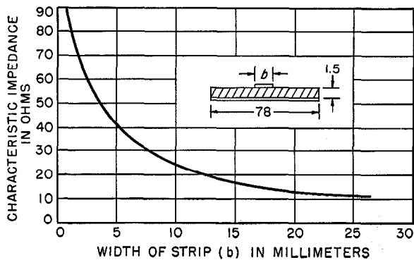
Figure 2—Characteristic impedance for microstrip as a function of the width of the strip. Fiberglass G-6 dielectric is used. Dimensions are in millimeters.
