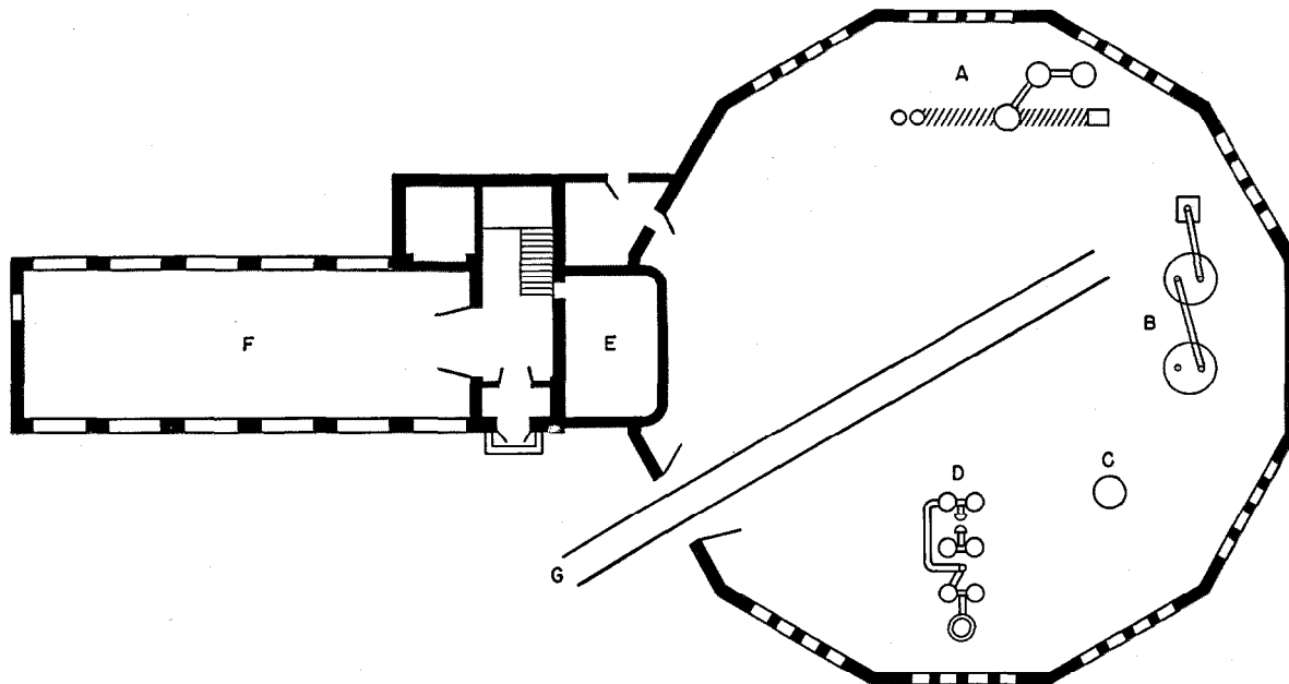
Figure 1—Plan of the laboratory. A—the 1 000 000-volt direct-current test set. B—600 000-volt alternating-current reactor set. C—1.5-meter-(4.9-foot-) diameter spark gap. D—2 100 000-volt impulse generator. E—the control room (on the second floor). F—physical laboratory, instrument shop, et cetera. G—railroad track.
