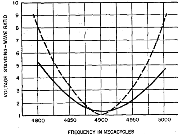
Figure 16—Input voltage standing-wave ratio plotted against frequency for a resonant section.
