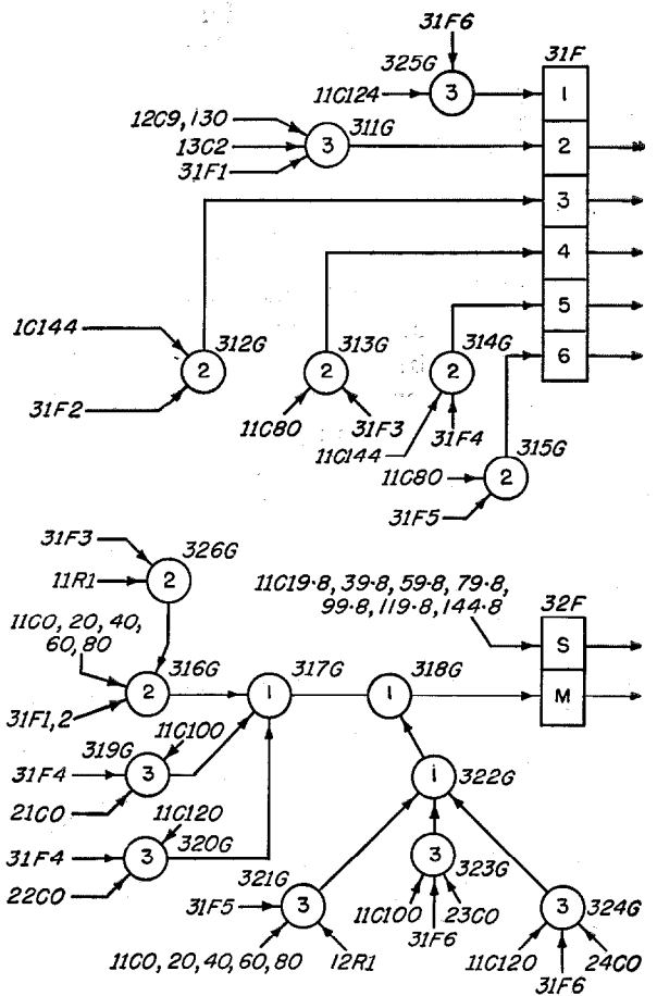
Figure 15—Error-correcting-system character emission, outgoing terminal.
