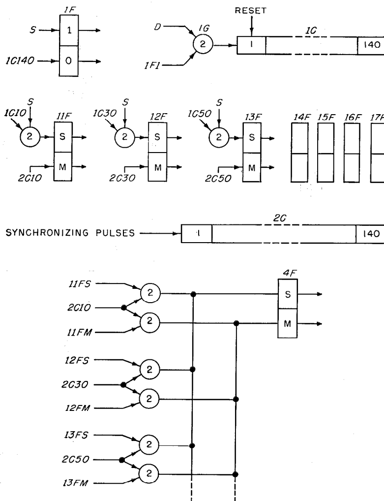
Figure 13—Receiving end for character synchronization.
