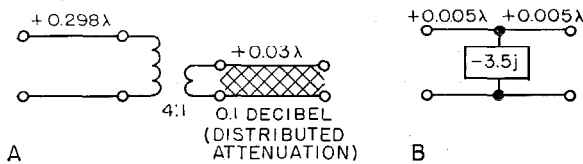
Figure 5—A is the exact equivalent circuit including losses deduced from Figure 4 and B is the approximate equivalent circuit neglecting the losses for a post transverse to a microstrip line.
