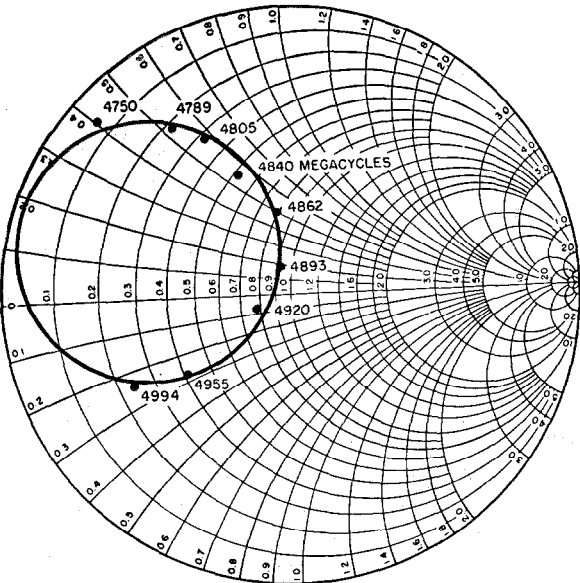
Figure 15—Frequency response and Q of a resonant section obtained experimentally.
