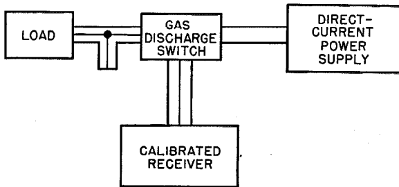
Figure 12—Equipment arrangement for noise measurement.
