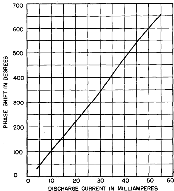
Figure 11—Phase shift plotted against discharge current for 18 inches (46 centimeters) of RG-52/U waveguide within which was a rectangular glass tube 1.9 by 0.8 centimeters (0.75 by 0.315 inch) filled with neon and argon at a pressure of 1.5 millimeters of mercury. The excitation frequency was 9450 megacycles.
