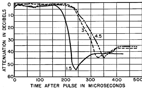
Figure 22—Attenuation plotted against time after a 1-microsecond discharge pulse in argon at the pressures indicated in millimeters of mercury. The pulse current was 1 ampere and the steady-state current was 25 milliamperes.
