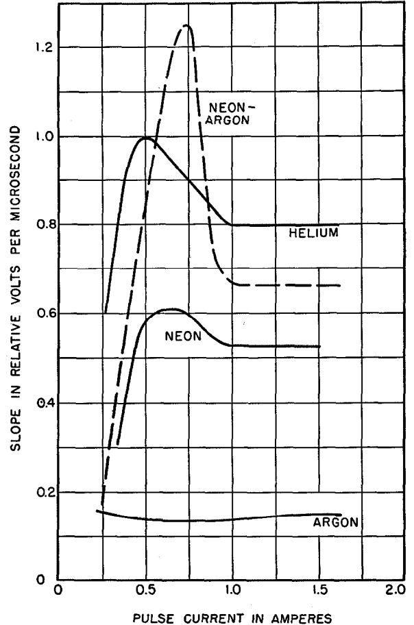
Figure 27—Rate of transmission decay as a function of the amplitude of 1-microsecond pulses starting from 20 milliamper steady-state conditions. The gases indicated (neon-argon being 1-percent argon) are at pressures of 2 millimeters of mercury.
