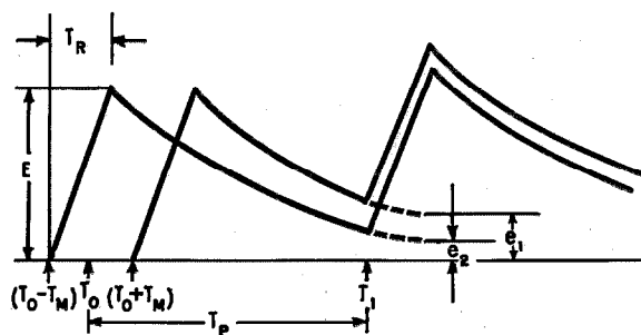
Figure 1—Effect of high-frequency response on cross talk in pulse-position modulation using a resistance-capacitance filter.
