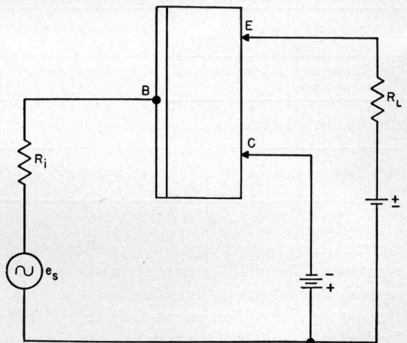
Figure 11—Emitter-output connection.
