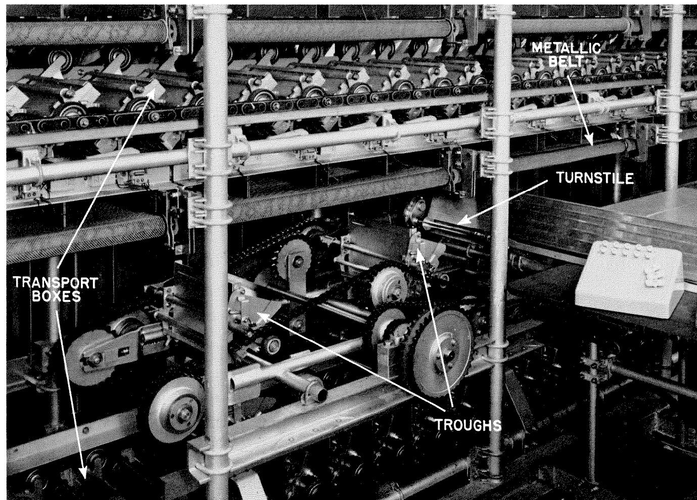
Figure 5—The troughs on the transfer device and some other parts of the machine are shown below.
