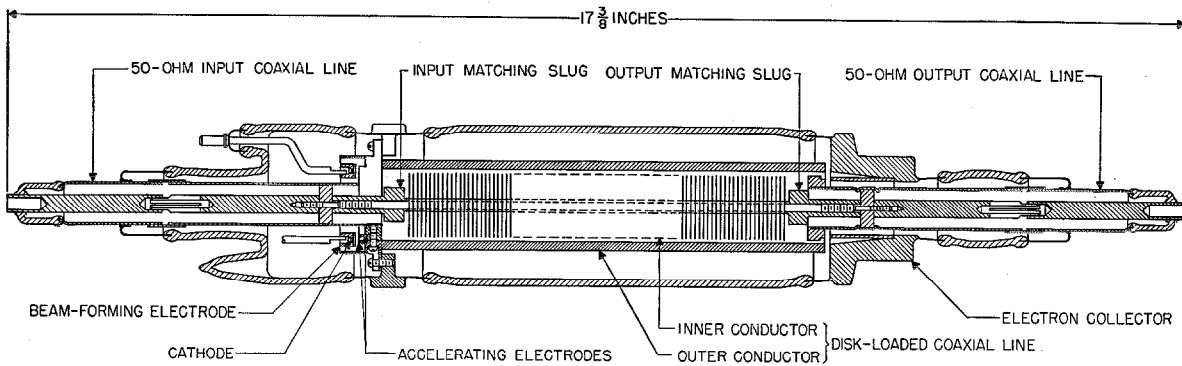
Figure 7—Experimental tube.
