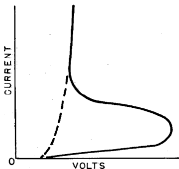
Figure 8—Electro-forming characteristics.
