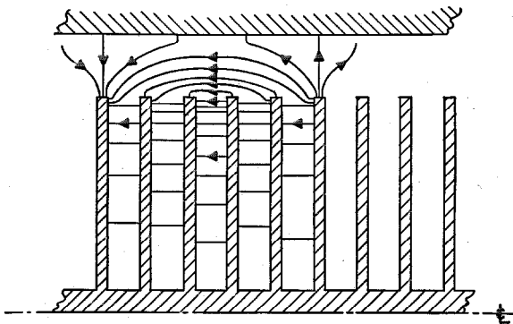
Figure 2—Qualitative picture of the electric field.
