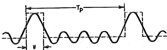
Figure 4—Effect of high-frequency response on cross talk in pulse-position modulation using a low-pass filter. For the \pi network C_0 R C_c = 78,900 , C = 2C_0 , C_0 L F_c^2 = 12,670 , in micromicrofarads, microhenries, ohms, and megacycles.
