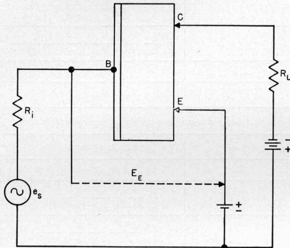
Figure 10—Base-input connection.
