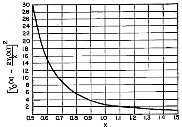
Figure 7—Plot of [Y_0(X) - \frac{2Y_1(X)}{X}]^2 against X .
