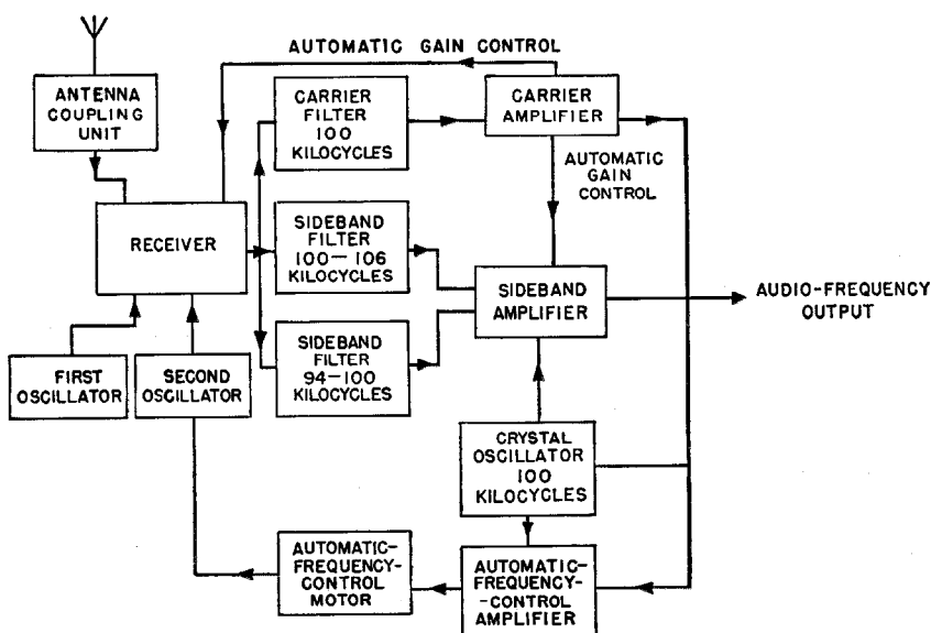
Figure 13—Block diagram of R.X.9. receiver.
