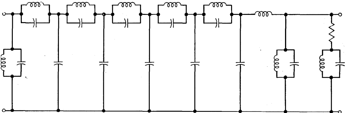
Figure 6—Filter for transition band from 106-184 kilocycles.
