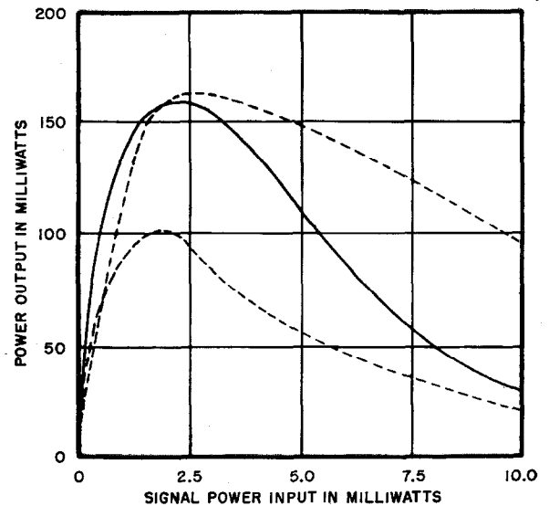
Figure 12—Relation between power output and signal power input. Solid line is for optimum helix voltage (1350 volts) for maximum gain. The upper broken line is for 50 volts above and the lower curve for 50 volts below optimum.
