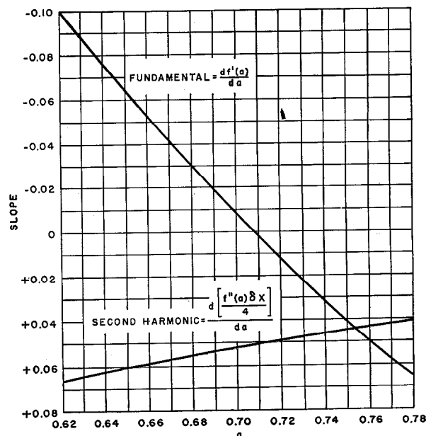
Figure 9—Slopes of the coefficients of fundamental and second harmonic plotted against a , where \delta X = 0.2 .
