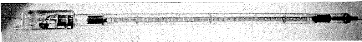
Figure 2—Travelling-wave tube for 10-centimetre work. Length approximates 24 inches.
