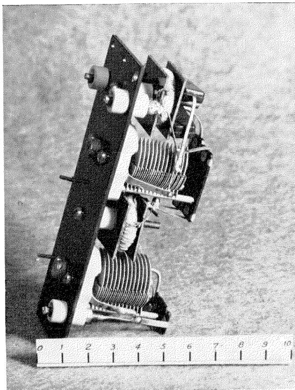
Figure 9—Constructional arrangement of one section of phase-shifting network.
