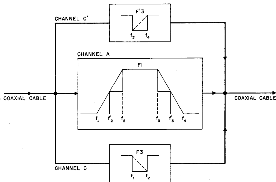
Figure 1—Arrangement of filters for removing a frequency band \Delta F from a coaxial cable. Distortion at band edges resulting from the characteristics of the main filter F1 is compensated by filters F3 and F'3 , which operate in the transitional-frequency bands.
