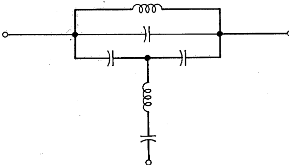
Figure 8—Type of phase-shifting network used.
