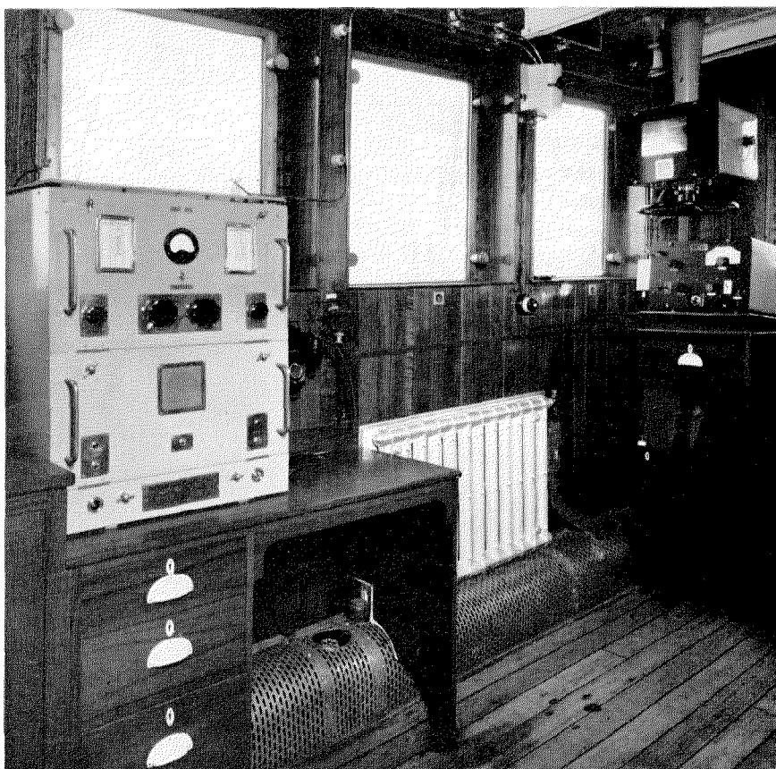
Figure 21—Corner of wheelhouse (port side) showing direction-finder and radiotelephone.
