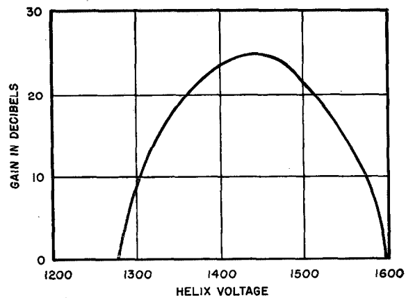
Figure 11—Variation of gain with helix voltage.
