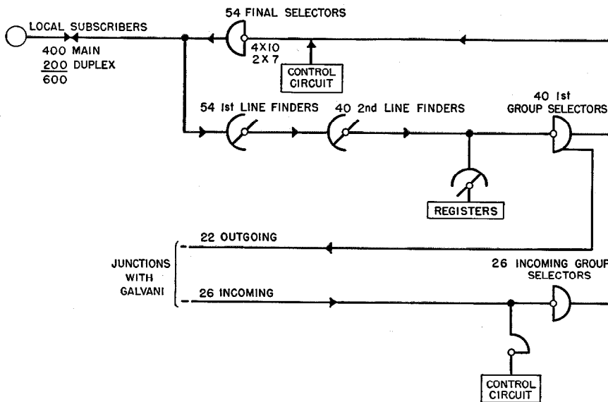
Figure 4—Rural-type exchange junction diagram for Galliera office.
