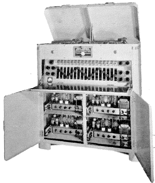
Figure 22—Public-address console with front panel and doors open.
