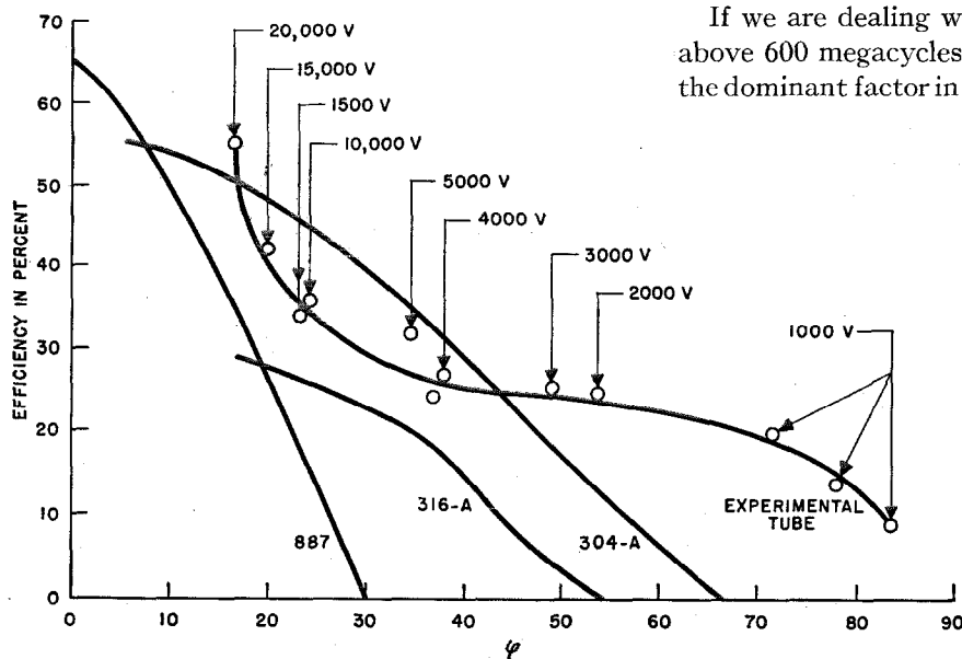
Fig. 6—Efficiency plotted against \phi for three prewar triodes and an experimental tube.
