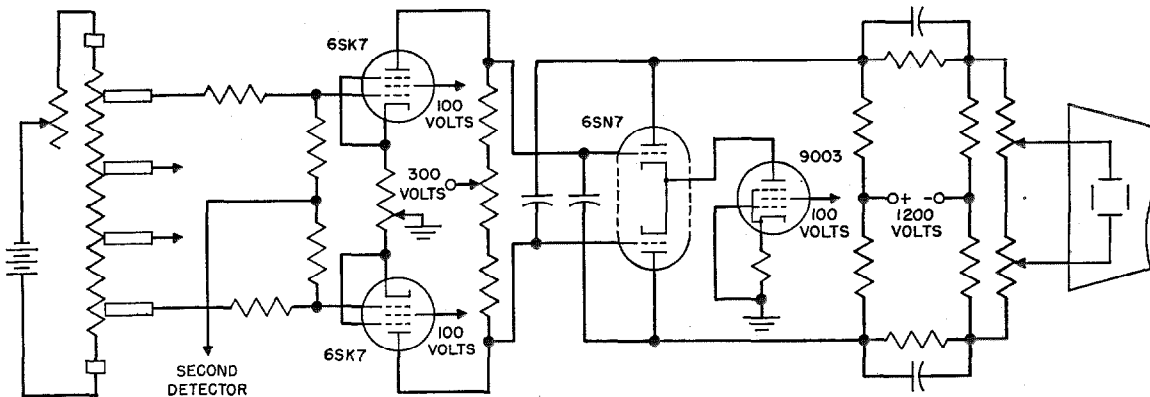
Fig. 6—The voltage from the distributor is amplified and applied to the deflecting plates of the cathode-ray tube. A similar amplifier operates on the quadrature phase from the other distributor probes, supplying voltage to the second pair of deflecting plates and producing a circular sweep. A 5-volt square-wave signal applied to both amplifiers from the second detector of a receiver will reduce the radial deflection to zero. The 9003 is used as a cathode bias resistor for the 6SN7.
