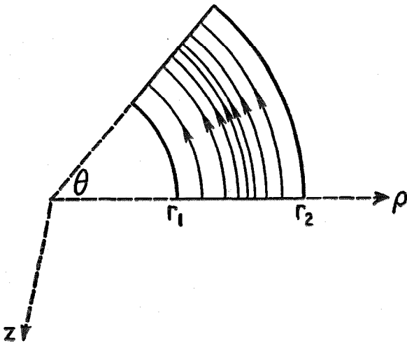
Fig. 11—Pattern representing the electric field of an H -wave, of zero order and principal mode, propagated through a guide composed of portions of two coaxial circular cylinders and two radial planes.
