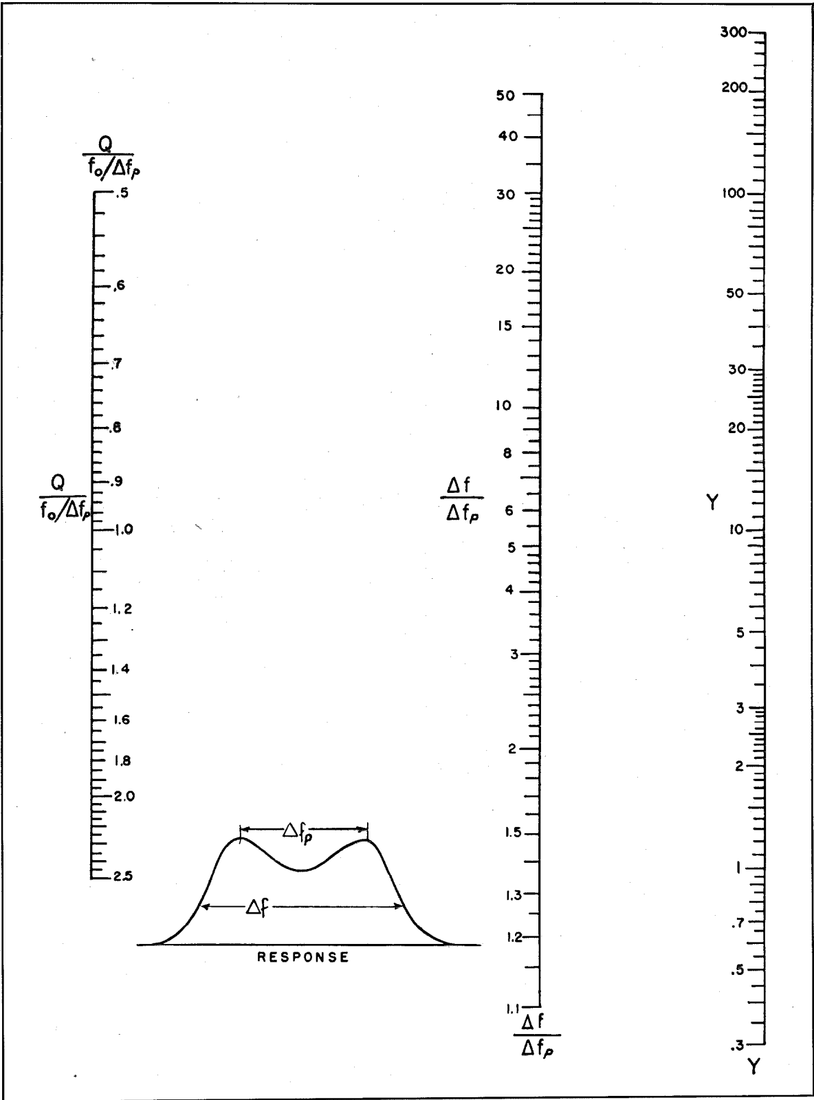
Chart C—Double-tuned band-pass circuit design.
