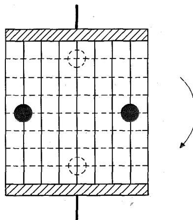
Fig. 3—Linear distributor. Uniform lines of current, indicated by solid lines, flow across a plane resistive sheet from copper connecting bars. Equipotential lines, shown dotted, are at right angles to the current flow. Probes are shown as large solid dots. Relative rotation of the probes about the central point on the sheet will develop a sine-wave voltage between the probes. For two-phase output, the additional pair of probes shown dotted may be used.
