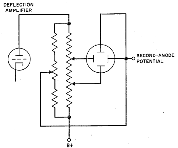
Fig. 8—Centering method used with simplified two-phase generator and tubes having two deflecting plates connected together internally.
