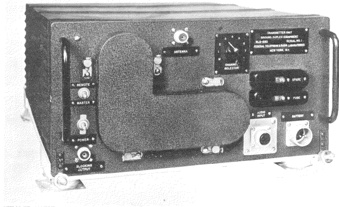
Fig. 3—Experimental pulse-time-modulation transmitter designed to operate with the U. S. Army EE-8 field telephone system.
