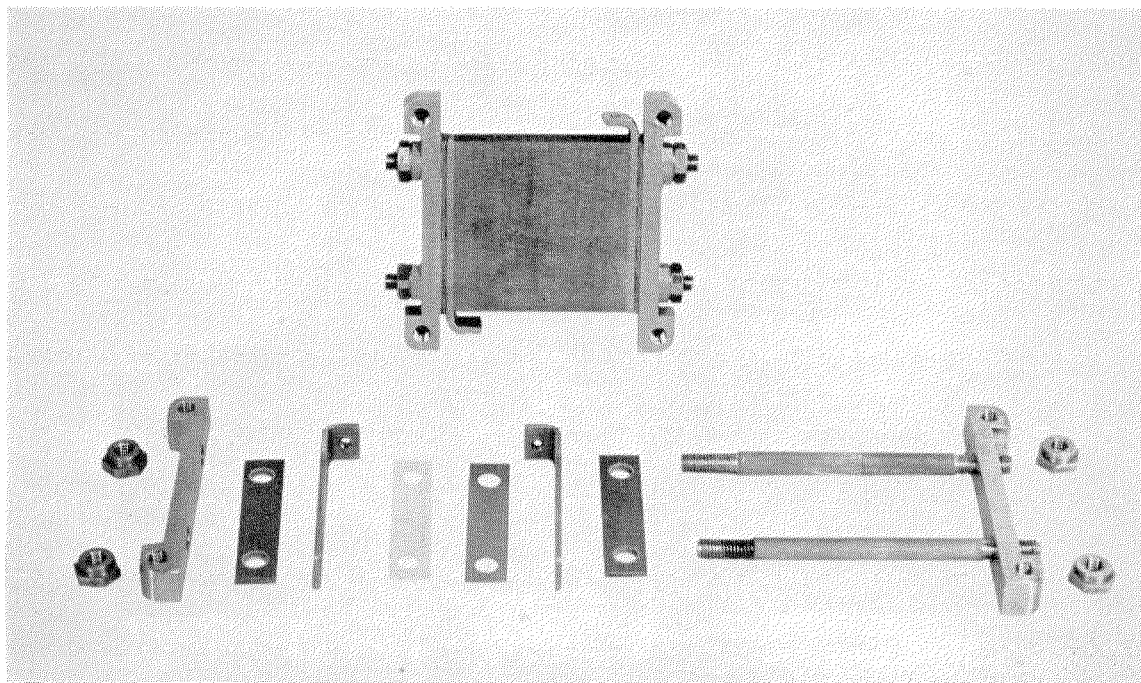
Fig. 10—Commutator assembly. Conducting and insulating laminations alternate. A resistive material makes contact with the conducting sheets on one side while the brushes bear on the other side.
