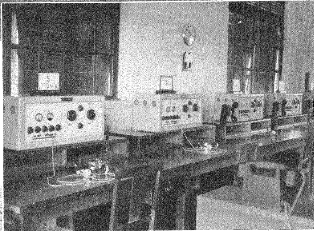
The high-frequency receiving room at Luanda.
