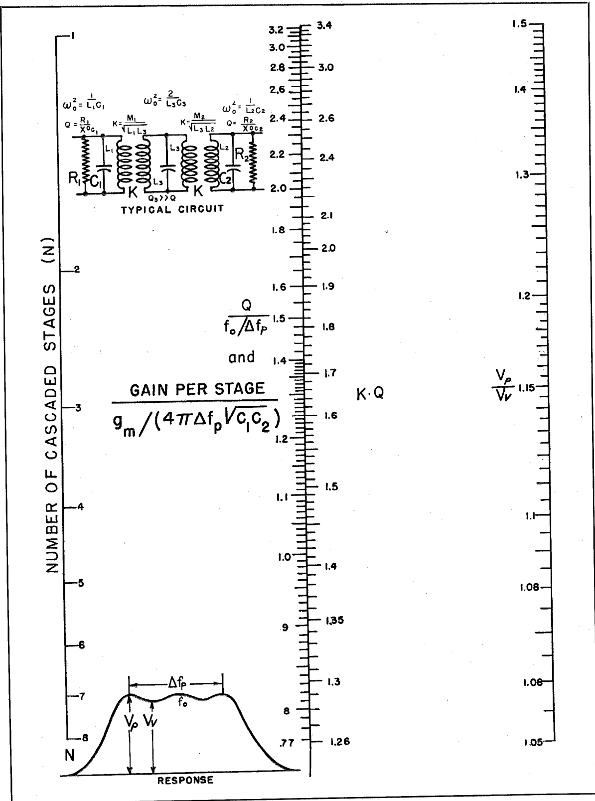
Chart I—Triple-tuned band-pass circuit design.
