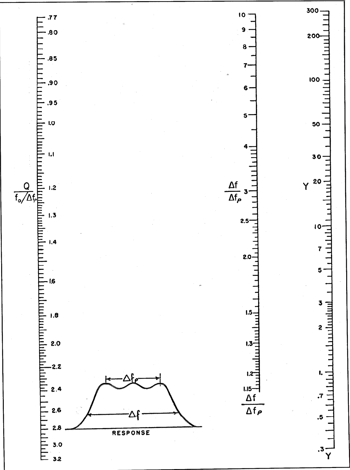
Chart III—Triple-tuned band-pass circuit design.
