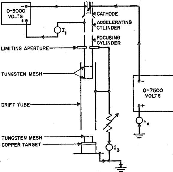
Fig. 12—Schematic diagram of apparatus.
