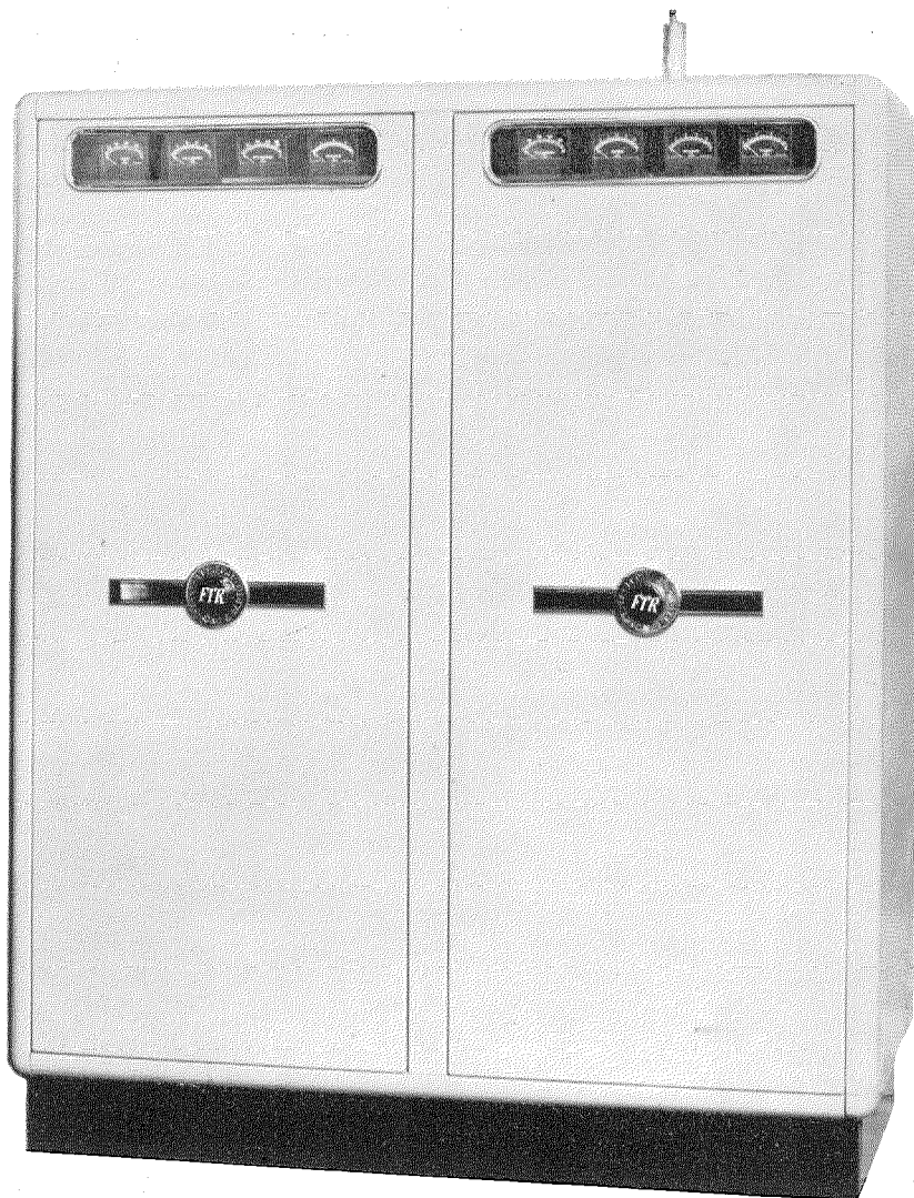
3-kilowatt frequency-modulated transmitter, front view, doors closed.
