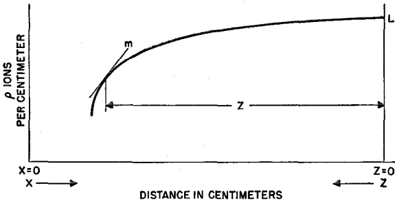
Fig. 3—Universal ion-density curve.
