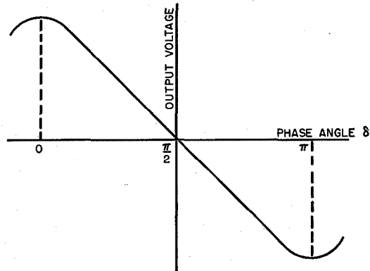
Fig. 4—Response curve of phase detector.
