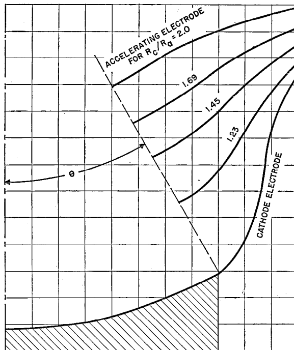
Fig. 6—Shape and placement of accelerating electrode for indicated values of R_c/R_a , where \theta=30 degrees.
