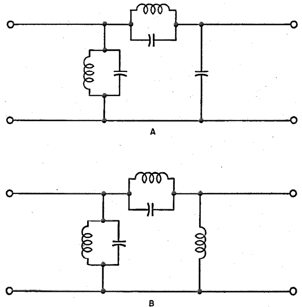
Fig. 3—Reduction of circuit of Fig. 2; A for cases where f_2 > f_3 , and B if f_2 < f_3 .
