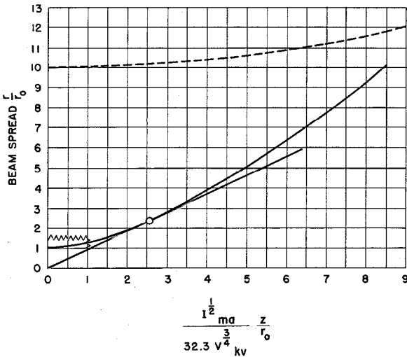
Fig. 7—Universal beam-spread curve (negative space-charge effect).
