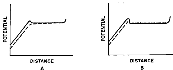
Fig. 14—Potentials at center and edge of beam during ion trapping.
