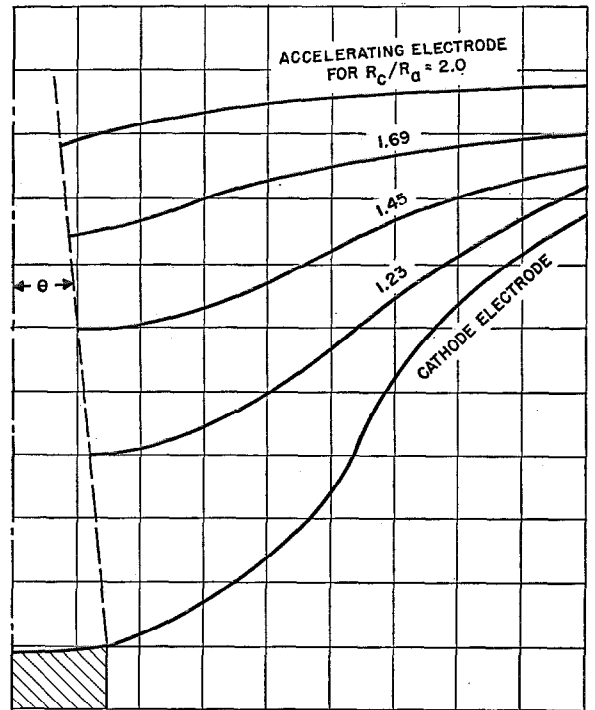
Fig. 3—Shape and placement of accelerating electrode for indicated values of R_c/R_a , where \theta = 5 degrees.
