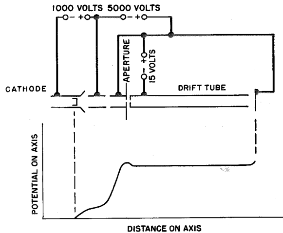
Fig. 13—Ion-trapping apparatus and potentials.
