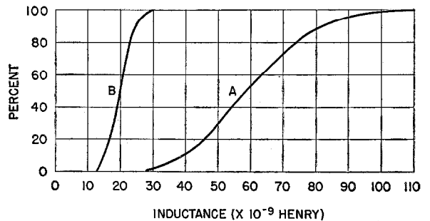
Fig. 14—Real-to-real mutual inductance of 12-channel star quads; A—between real circuits of one quad; B—between real circuits of different quads.
