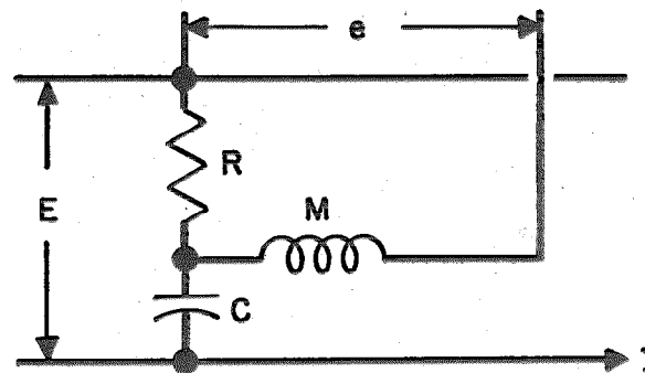
Fig. 4—Equivalent circuit of reflectometer.
