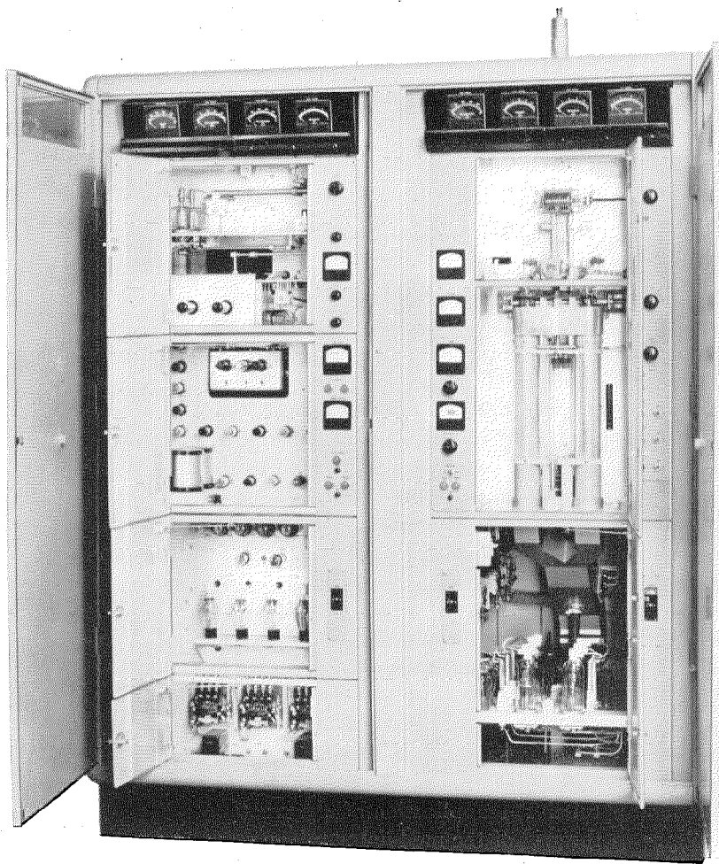
3-kilowatt frequency-modulated transmitter, front view, access doors open.
