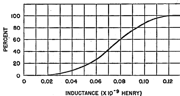
Fig. 18—Mutual inductance between 12-channel pairs and real circuit of star quads (12-channel).
