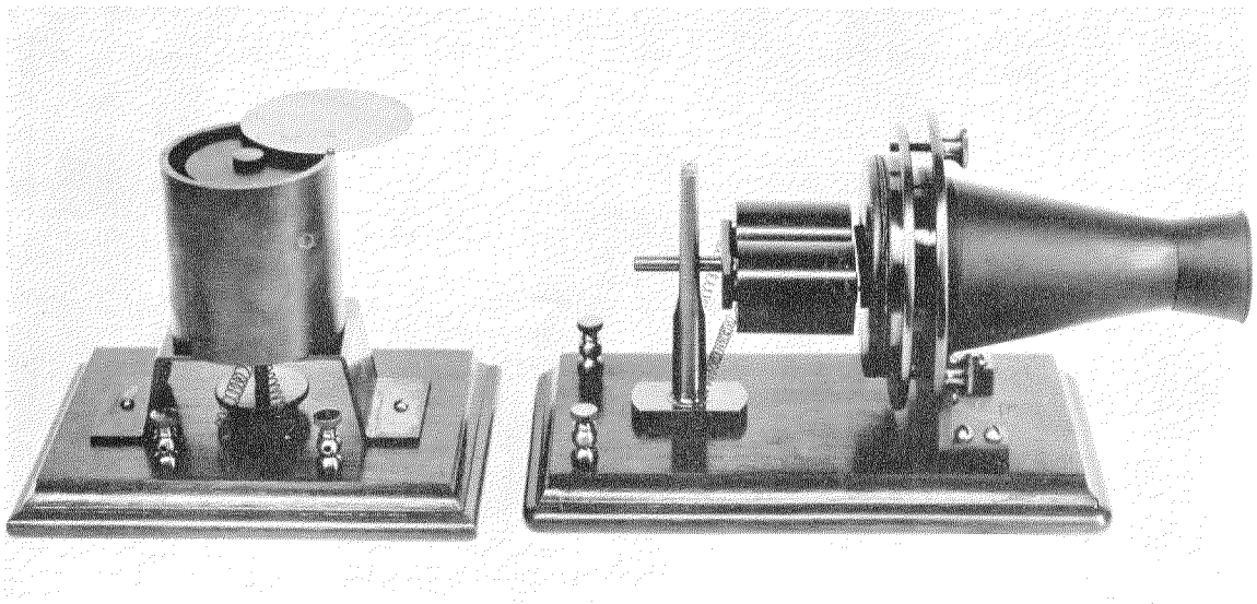
Replicas of the "iron-box" receiver and an improved magnetic transmitter. The iron-box receiver was developed by Bell shortly after the first intelligible speech was transmitted over the telephone. It employed a metal diaphragm and permanent magnet in a form comparable to the most modern receivers used in telephones today.
