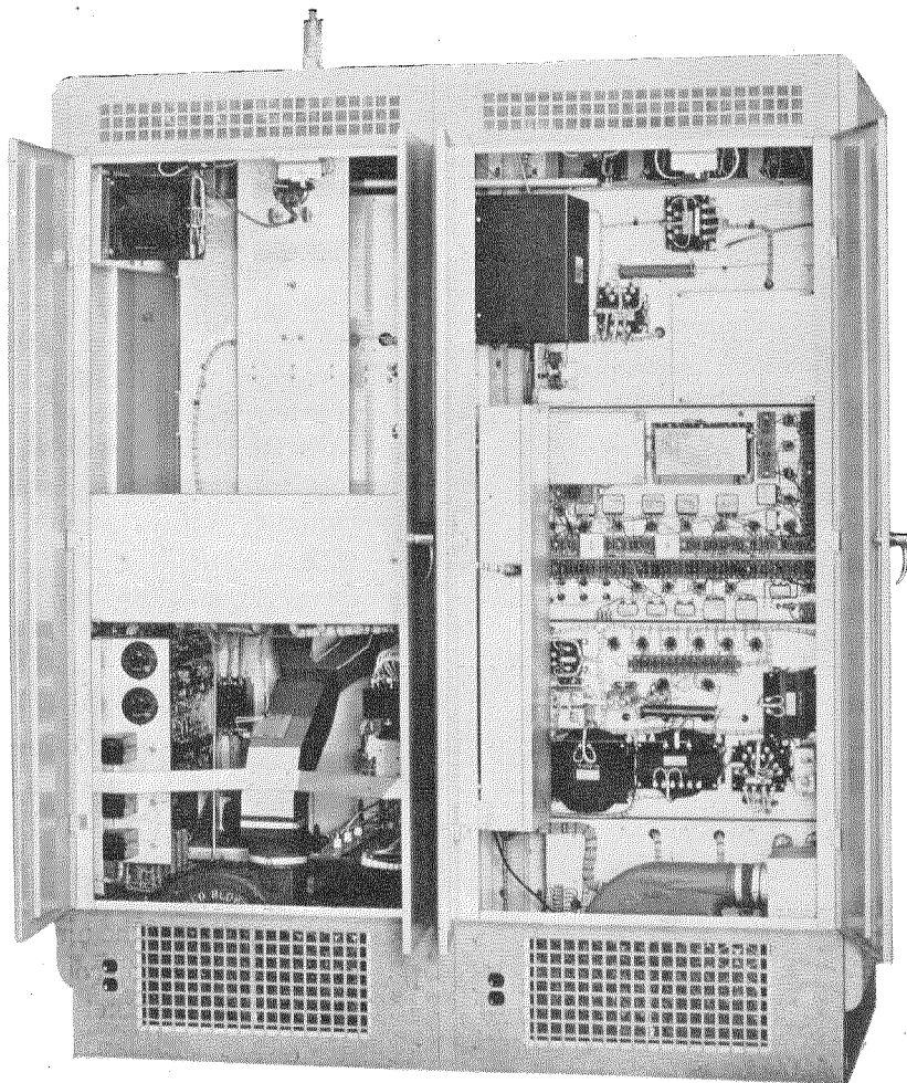
3-kilowatt frequency-modulated transmitter, rear view, doors open.
