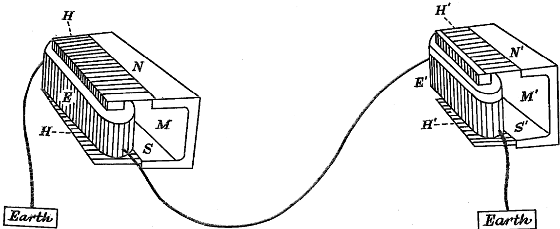
Bell's conception of his "harp" telegraph apparatus. H, H were two series of steel reeds, each reed having a different pitch. A single permanent magnet M was to be employed. An elongated electromagnet E was to be placed between the two series of reeds so that the free end of each reed might be close to the pole of the electromagnet without touching it. Bell never reduced this idea to practice, because it became evident to him that a single diaphragm could function as well as the many reeds.
