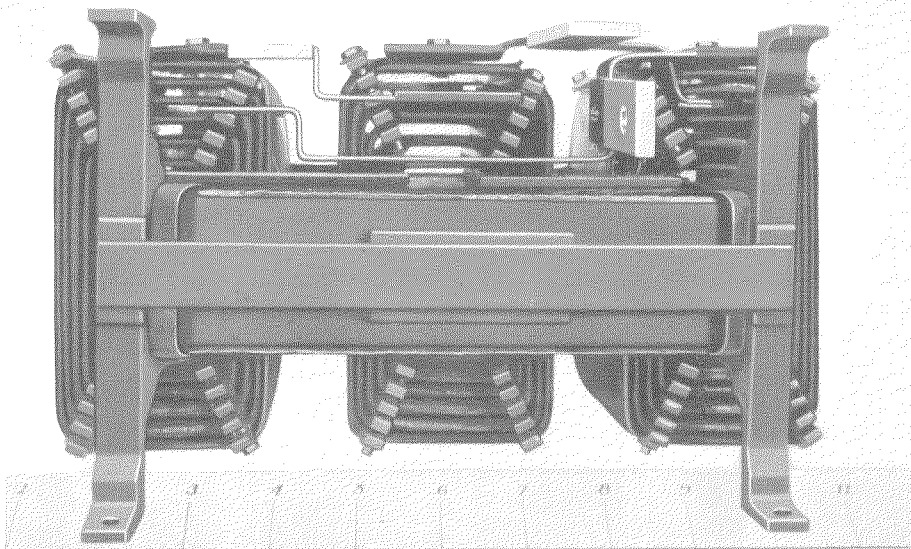
Fig. 6—Aircraft Transformer, Air-Cooled, 33.7-kva, 400-cycle, 3-phase, 250-volt primary, 28-volt secondary. Weight 30 pounds. Front View.
