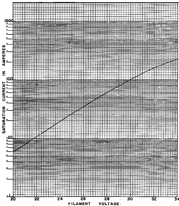
Fig. 10—Tube Type 3067A—Emission Characteristics
