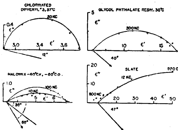
Fig. 16—Complex Dielectric Constants of Solids.
