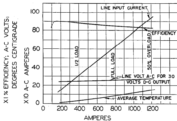
Fig. 9—Performance Characteristics of 800-ampere, 30-volt Rectifier used in Fig. 1 System.
