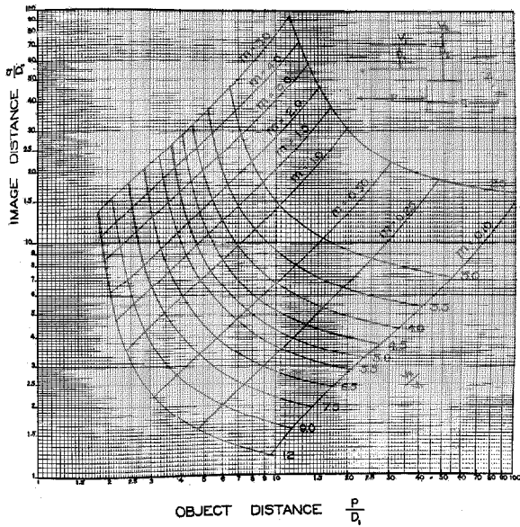
Fig. 3—Two Cylinder Lens D_2/D_1=1.5 .
