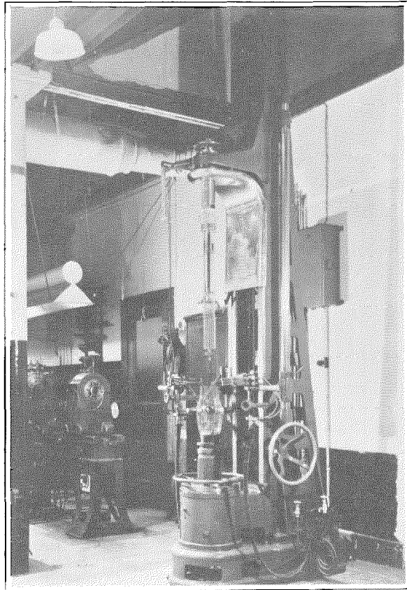
Fig. 8—Vertical Scaling Lathe.
