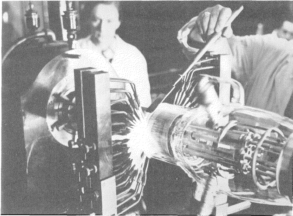
Fig. 7—Sealing of the Tube
