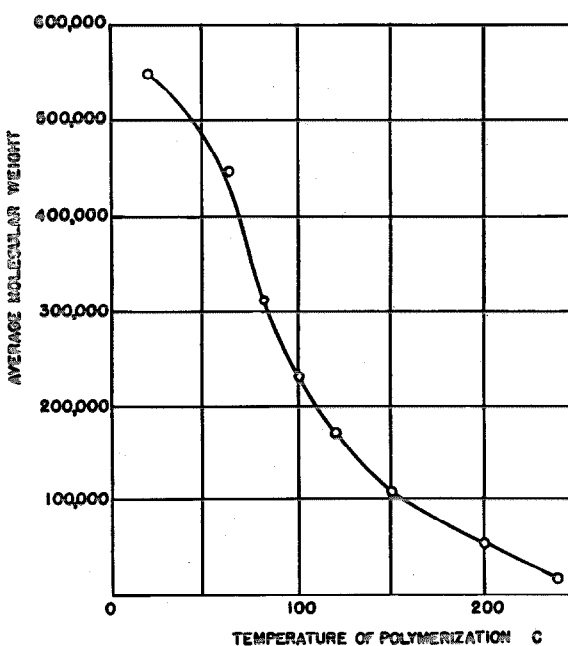
Fig. 3—Molecular Weight Dependence on Temperature for the Polymerization of Styrene.
