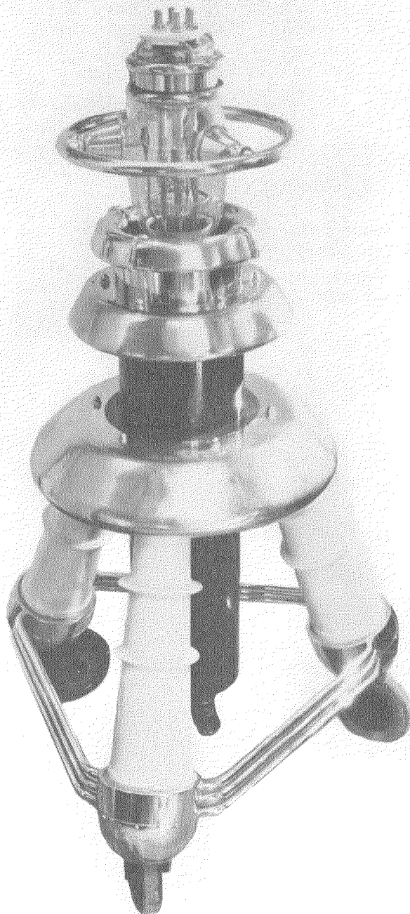
Fig. 9—3067A Vacuum Tube with Water Jacket and Truck.
