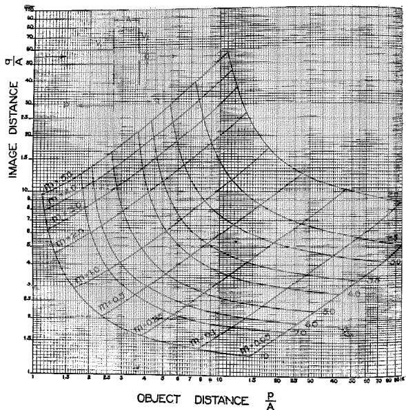
Fig. 6—Aperture Lens A/D=5 .
