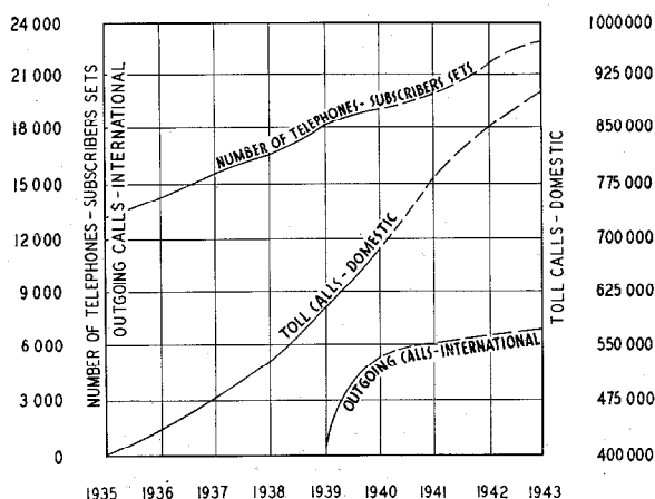
Fig. 4—Cia. Telefonica Rio Grandense (Brazil). Broken lines in above curves represent forecasts. Data for 1940 (as of end of year) are preliminary and partially estimated.
