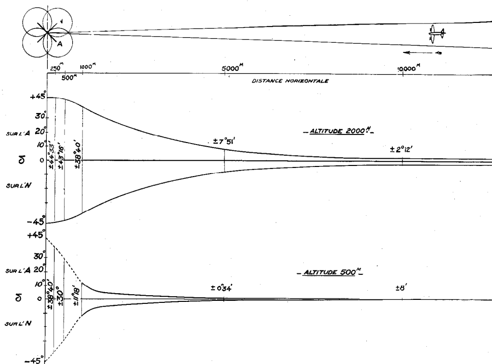
Fig. 9c—Progressive Errors in Alternate Directions of Approach in the Beam of a Loop Radio Beacon.
