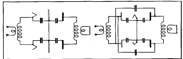
Fig. 2—Simplified Inverted Amplifier (A—left) and Conventional Neutralized Balanced Amplifier (B—right). In the Inverted Amplifier the Output Capacitance is Halved.
