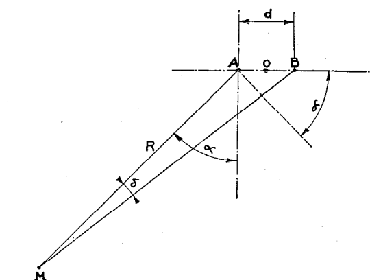
Fig. 12—Representation of the Geometrical Elements: Causes of Error at a Few \lambda Distance from a Spaced Antenna Radio Beacon.
