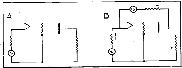
Fig. 1—Actual and Equivalent Circuits of the Inverted Amplifier. The Input and Output Effectively Operate in Series, as Shown in (B).
