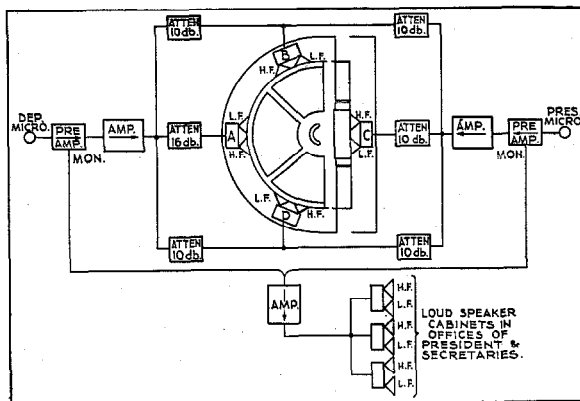
Fig. 2—Block Schematic Showing Arrangement of Microphones, Amplifiers, Attenuators and Loud Speakers.
