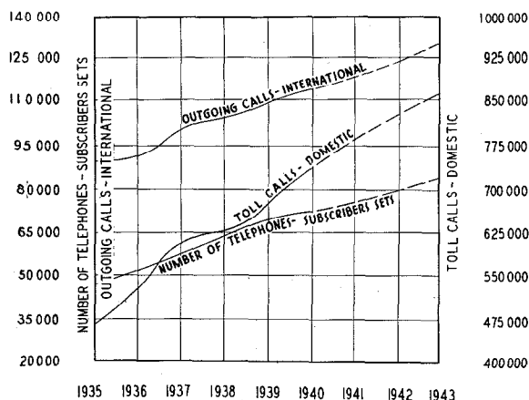
Fig. 7—Mexican Telephone Company. Broken lines in above curves represent forecasts. Data for 1940 (as of end of year) are preliminary and partially estimated.
