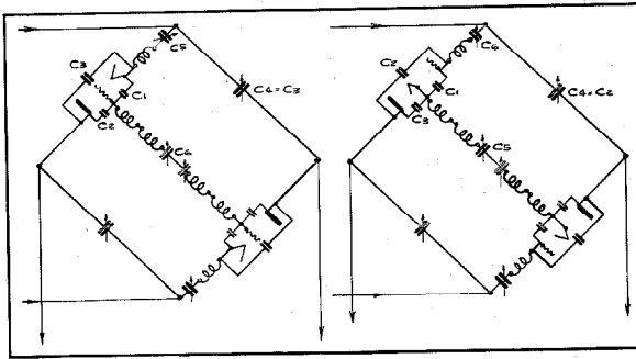
Fig. 3—Neutralization of Inverted Amplifier (A—left) and Conventional Amplifier (B—right). Similar Methods are Used, but the Inverted Amplifier Requires Smaller Balancing Capacitances.
