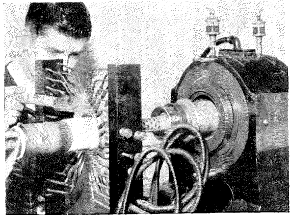
Sealing-in grid end of the 4030-C valve.
