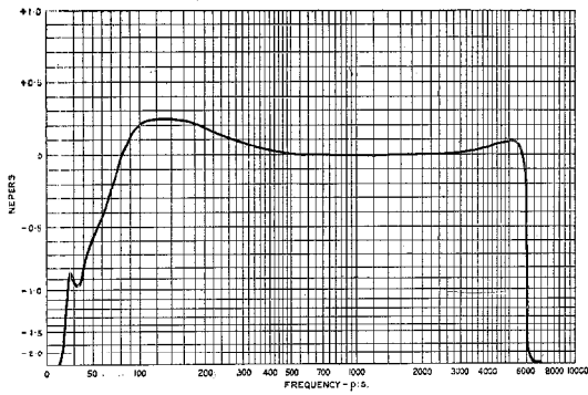
Fig. 6—Bâle-Zürich, H-20 Phantom Circuit No. 1 : Loss-Frequency Curve Measured at Zürich.
