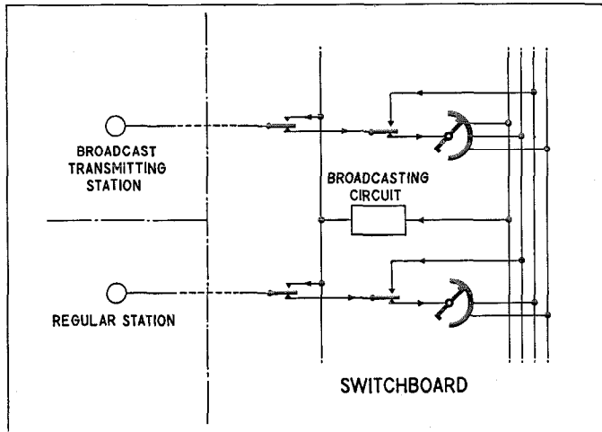
Fig. 3—Routing Diagram.
