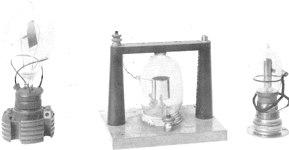
Fig. 3—Fleming Valves, 1904-1908.
