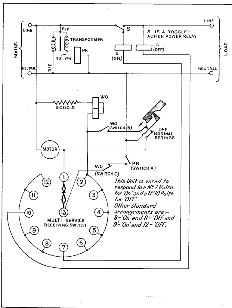
Fig. 9—Schematic Circuit of Multi-service Control Receiving Unit.
