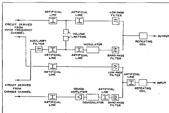
Fig. 1—Block Schematic of Single Channel Carrier System.
