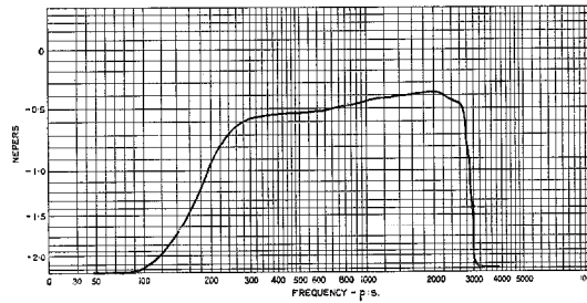
Fig. 9—Zürich-Bâle, Voice-Frequency Channel No. 1 : Loss-Frequency Curve Measured at Bâle (Including Terminating Set at Zürich).
