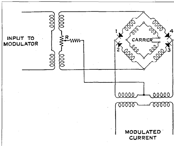
Fig. 3—Modulator Schematic.
