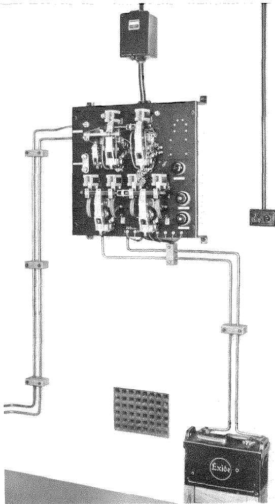
Fig. 1—Substation Biasing Panel and Battery.
