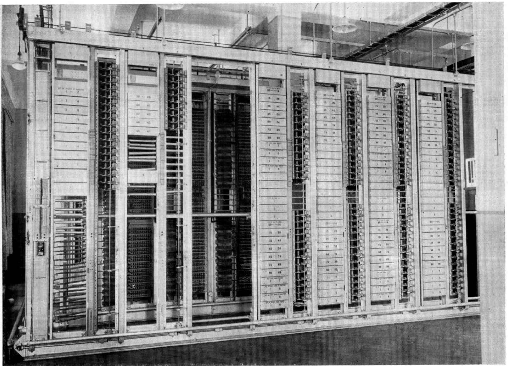
Fig. 5—Galati 7-D Exchange—1st Line Finders, Final Selectors and Penultimate Group Selectors.
