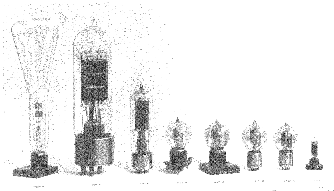
Fig. 7—A Range of Oxide-coated Alloy Filament Valves made by Standard Telephones and Cables, Limited.
