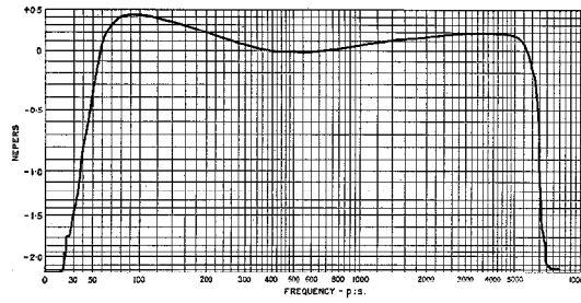
Fig. 7—Zürich-Bâle, H-20 Phantom Circuit No. 1 : Loss-Frequency Curve Measured at Bâle.
