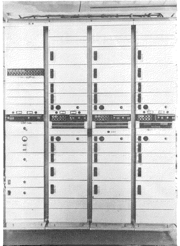
Fig. 13—Bay Containing Equipment for Six Carrier Channels.
