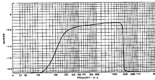
Fig. 11—Zürich-Bâle, Carrier Channel No. 1 : Loss-Frequency Curve Measured at Bâle (Including Terminating Set at Zürich).
