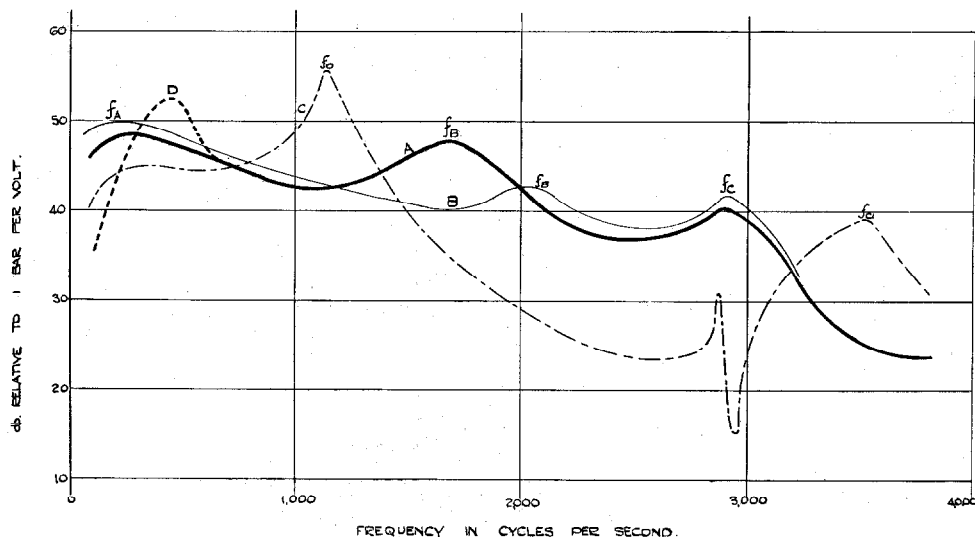
A - RECEIVER INSET 2-P. B - HEAD RECEIVER 10A/2. C - RECEIVER INSET 1-L. D - SHOWING EFFECT OF A LEAK BETWEEN EARCAP AND EAR.
