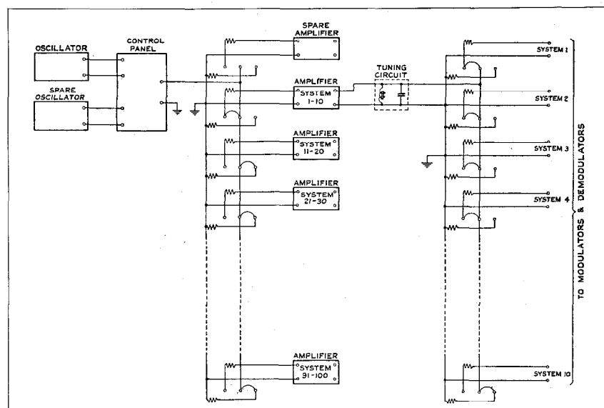
Fig. 4—Block Schematic of Carrier Current Supply.
