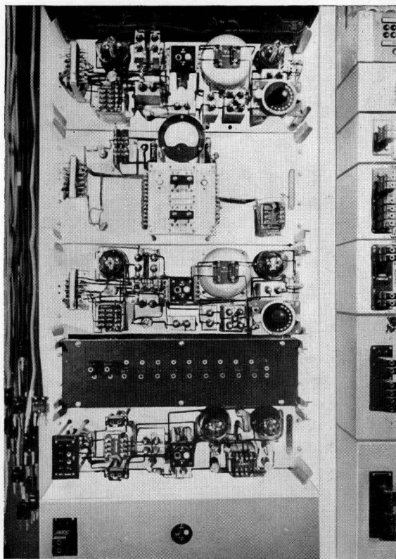
Fig. 5—Carrier Supply.
