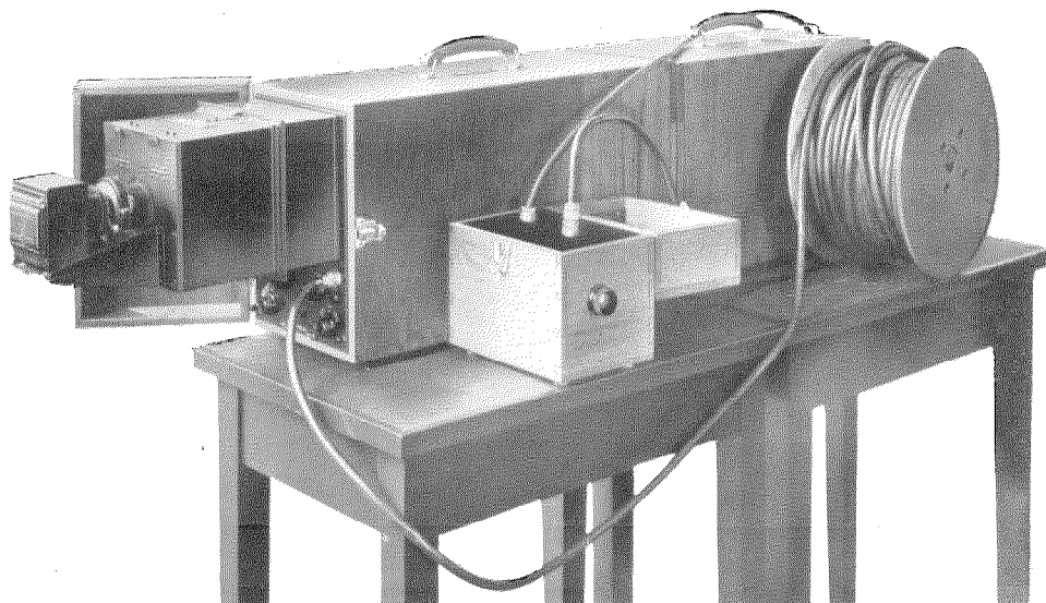
Transient Recorder Equipment, with Delay Cable in Circuit, connected up for recording Surge Generator Wave.
