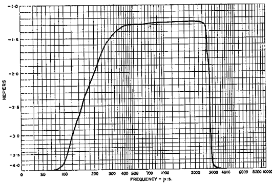
Fig. 10—Bâle-Zürich, Carrier Channel No. 1 : Loss-Frequency Curve Measured at Zürich Terminating Set.
