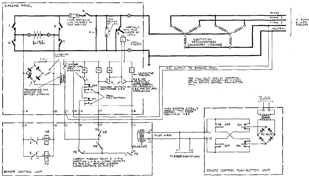
Fig. 8—Schematic Circuit of Substation Biasing Panel with Remote Control.
