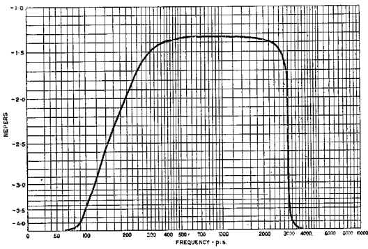
Fig. 8—Bâle-Zürich, Voice-Frequency Channel No. 1 : Loss-Frequency Curve Measured at Zürich Terminating Set.
