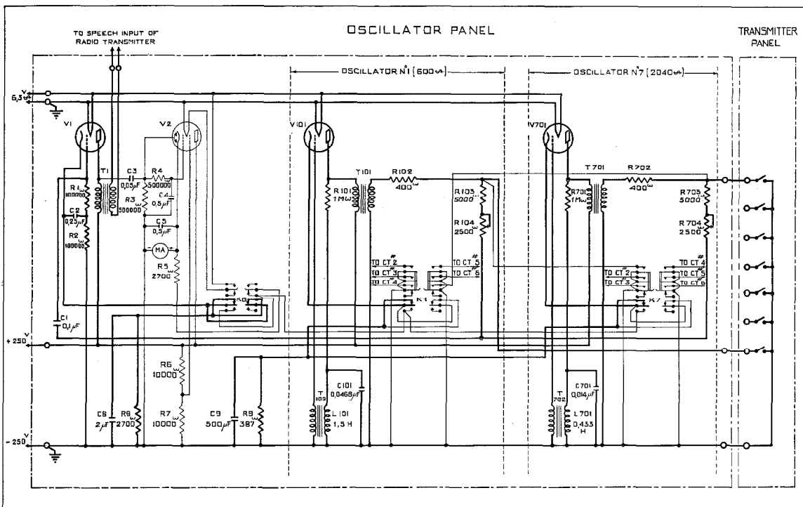
Fig. 7—Schematic Diagram of Oscillator Panel.
