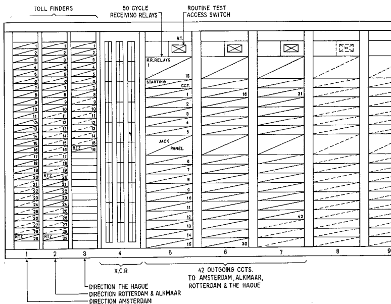
Fig. 3—Equipment Layout of Switchboard with Outgoing Toll Line Circuits (Front of Rack).
