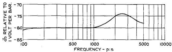
Fig. 3—Typical Transmitter Frequency Characteristic.
