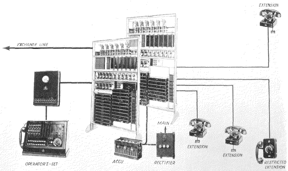
Fig. 3—System for Maximum of 10 Exchange Lines and 97 Extensions.
