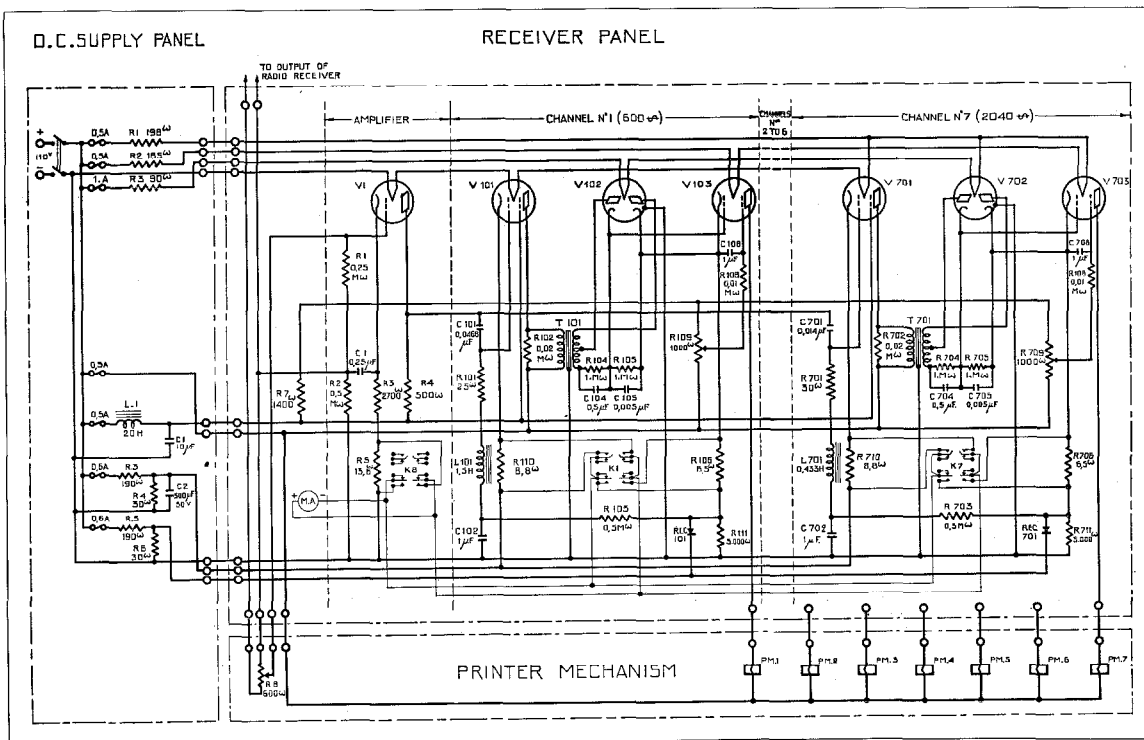
Fig. 8—Schematic Diagram of Receiver Panel.
