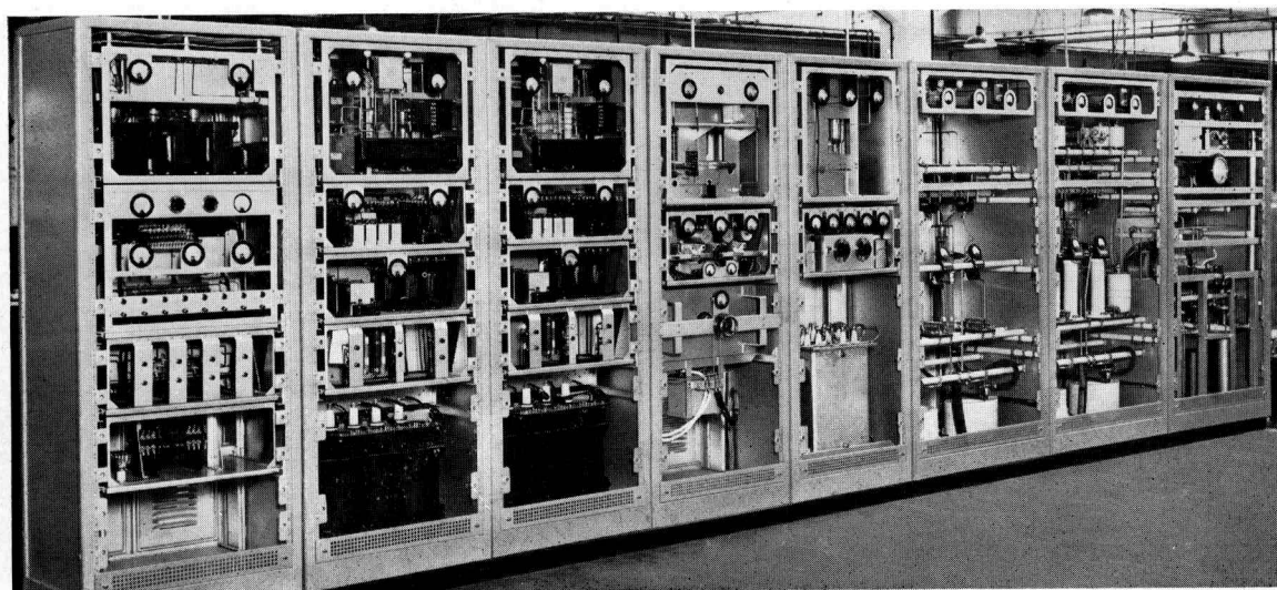
New "Standard" 10 kW Broadcasting Transmitter—Front view with panels removed. These panels are detachable without interference with the controls and meters.
