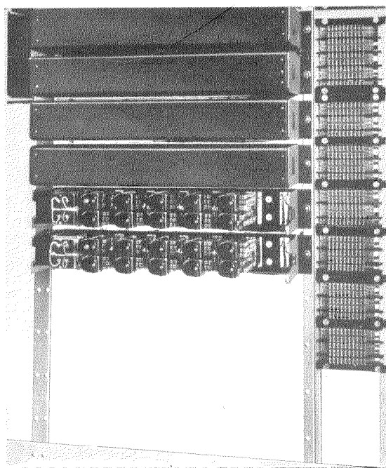
Fig. 10—Rack Showing Space for Mounting Relay Sets and Method of Connection to Soldering Strips.
