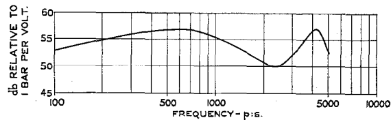
Fig. 4—Receiver Frequency Characteristic Measured on an Artificial Ear.
