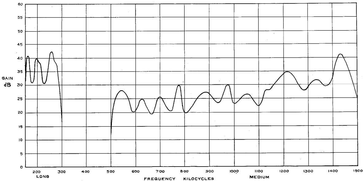
Fig. 4—Amplifier Characteristics.
