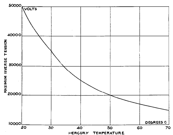
Fig. 7—Variation of the Maximum Inverse Voltage Supported by One of the Tubes Shown in Fig. 3 Versus the Temperature of the Condensed Mercury.
