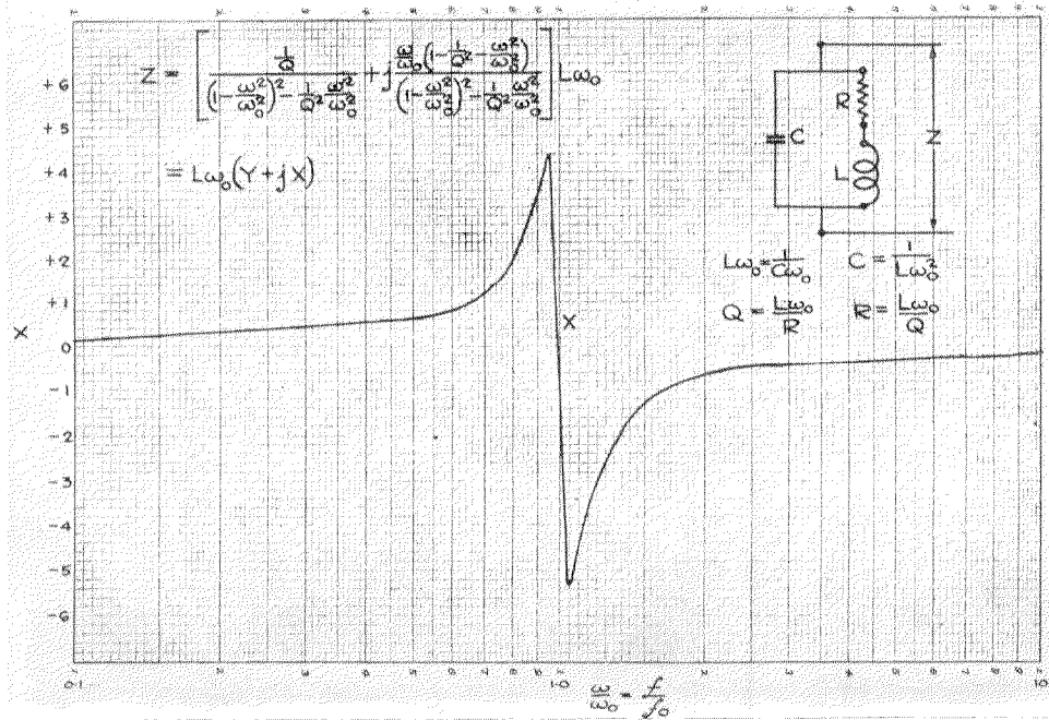
Fig. 4—Generalised Reactance Curve for Network Shown with Q=10 .
