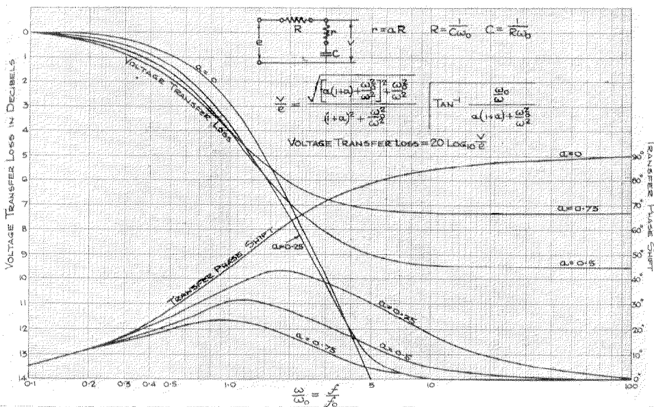
Fig. 15—Transfer Loss and Phase Shift for Network Shown.
