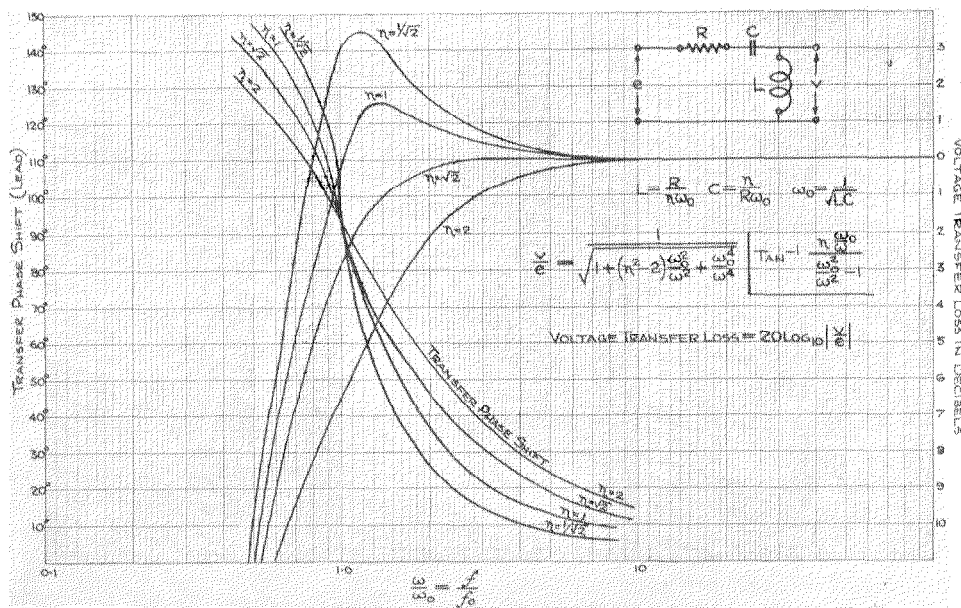
Fig. 14—Transfer Loss and Phase Shift for Network Shown.
