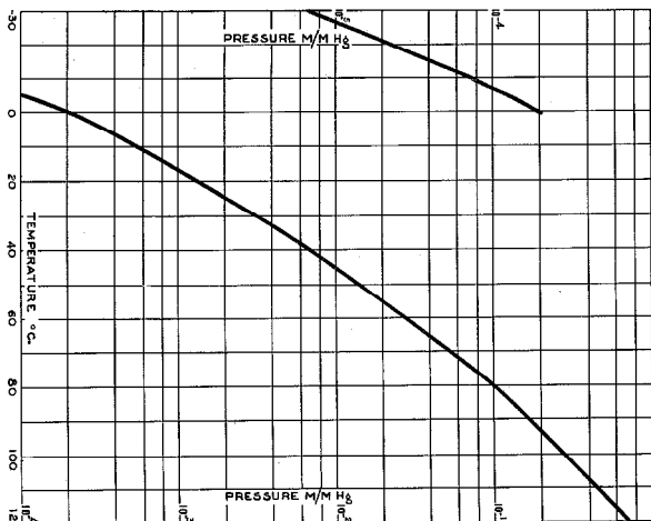
Fig. 5—Pressure Versus Temperature of Saturated Mercury Vapour.
