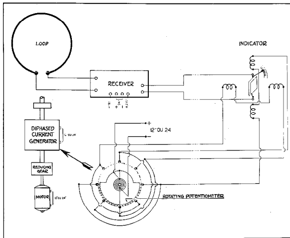
Fig. 1—Schematic Layout of Equipment.
