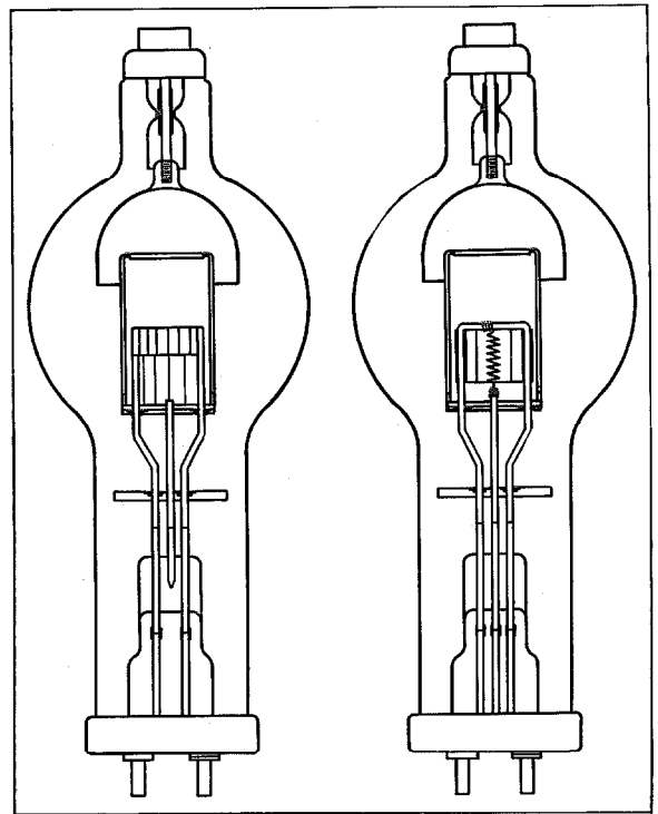
Fig. 1—Cross Section of Two Typical Hot Cathode Mercury Vapour Tubes. The Tube on the Left-Side is Directly Heated; the Other is Arranged for Indirect Heating.
