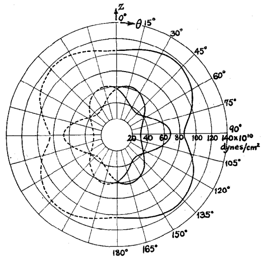
Figure 5—Values of c 's in the Frequency Equation (1) when the Normal to a Plate is in the Plane \phi = 0^\circ, 60^\circ, \text{ or } 120^\circ .
