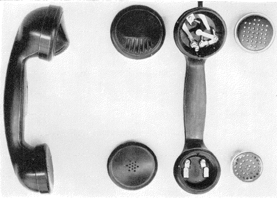
Figure 5—Moulded Microtelephone.
