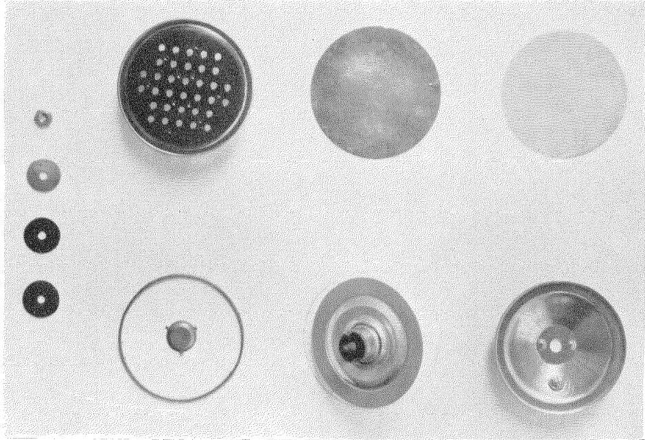
Figure 7—Microphone Capsule Parts.
