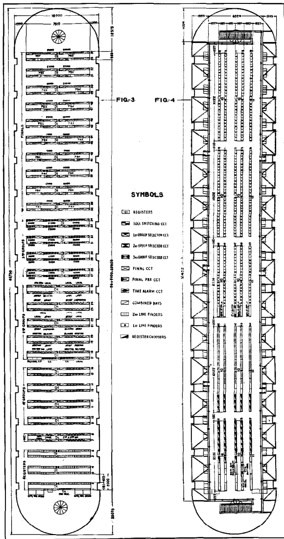
Figure 3—Layout of Lower Level of Switchcracks.
