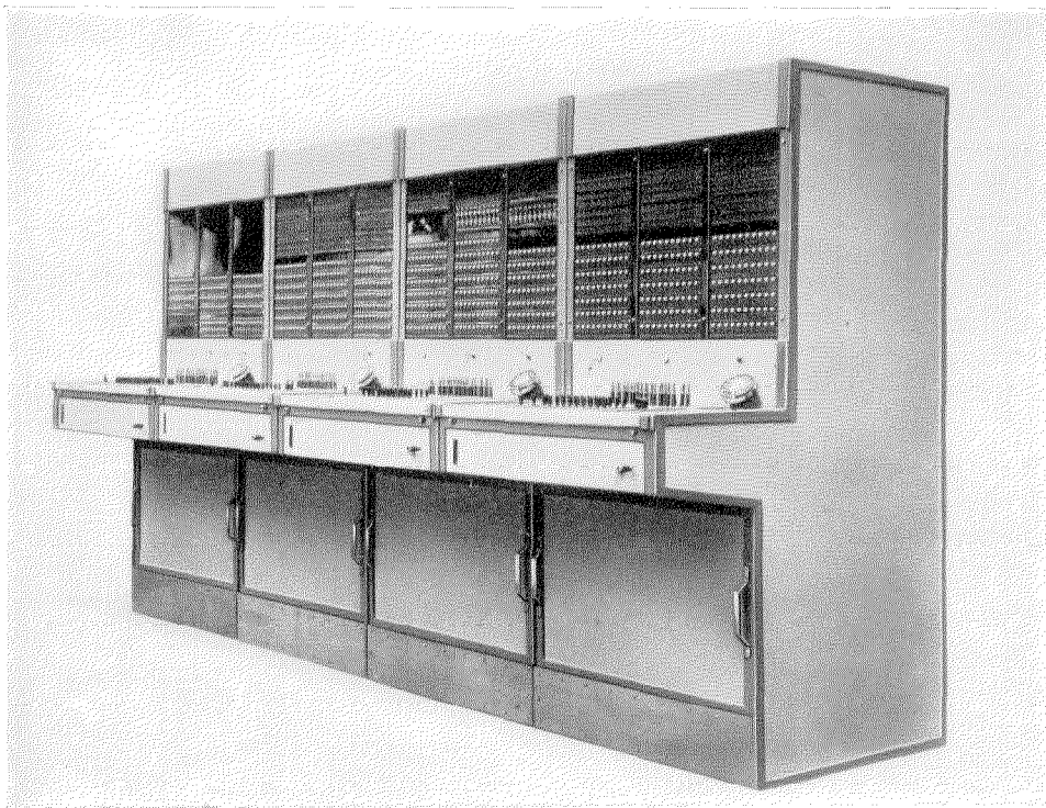
Figure 1—Officers' and Passengers' Telephone Switchboards—Front View.
