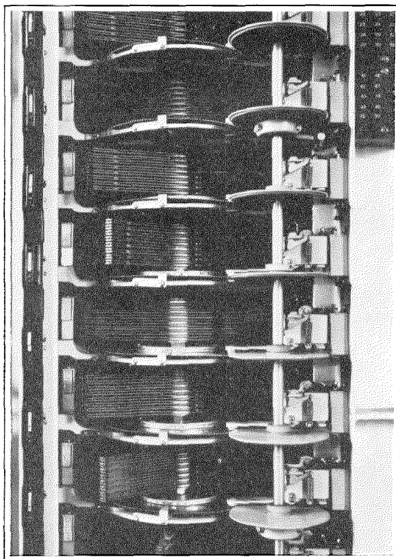
First and Second Line Finders.
