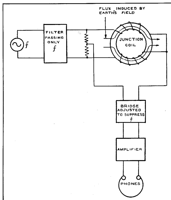
Figure 2—Even Harmonic Production in Loading Coils.
