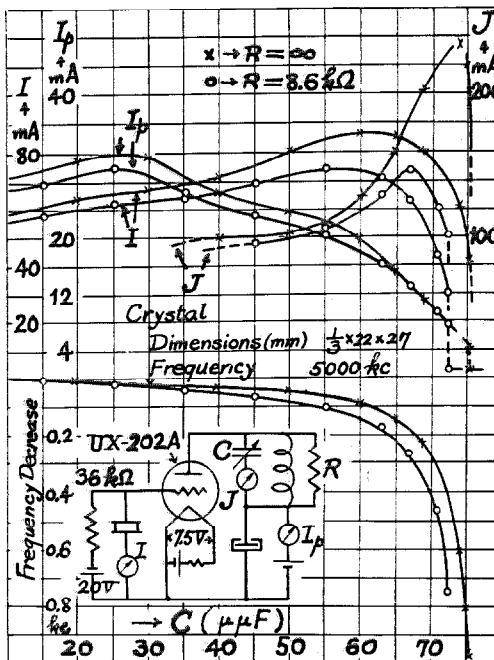
Figure 13—Characteristics of Triode Crystal Oscillator.
