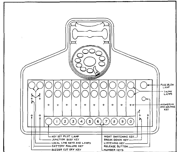
Attendant's Set.
