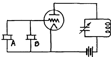
Figure 19—Two Crystals of Nearly the Same Frequency Connected in Parallel.
