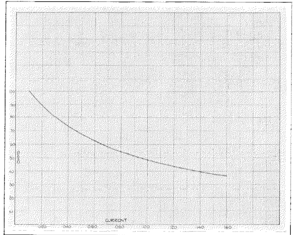
Figure 12—Talking Resistance of Microphone (Type A).
