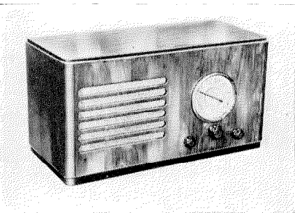
Figure 10—Standard Vienna 5-Tube (4 + 1) a-c. Receiver with Protection Scale and Neon Tuning Beacon.
