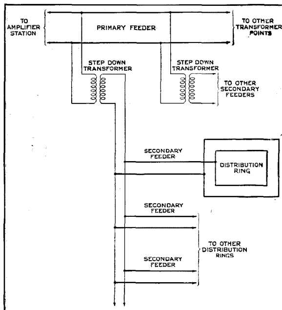
Figure 1—Rediffusion Feeder System—General Layout.
