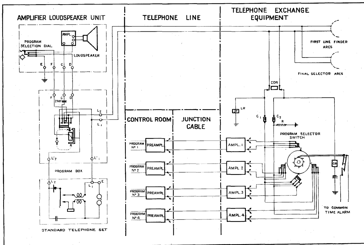
Figure 7—Teleprogramme System.
