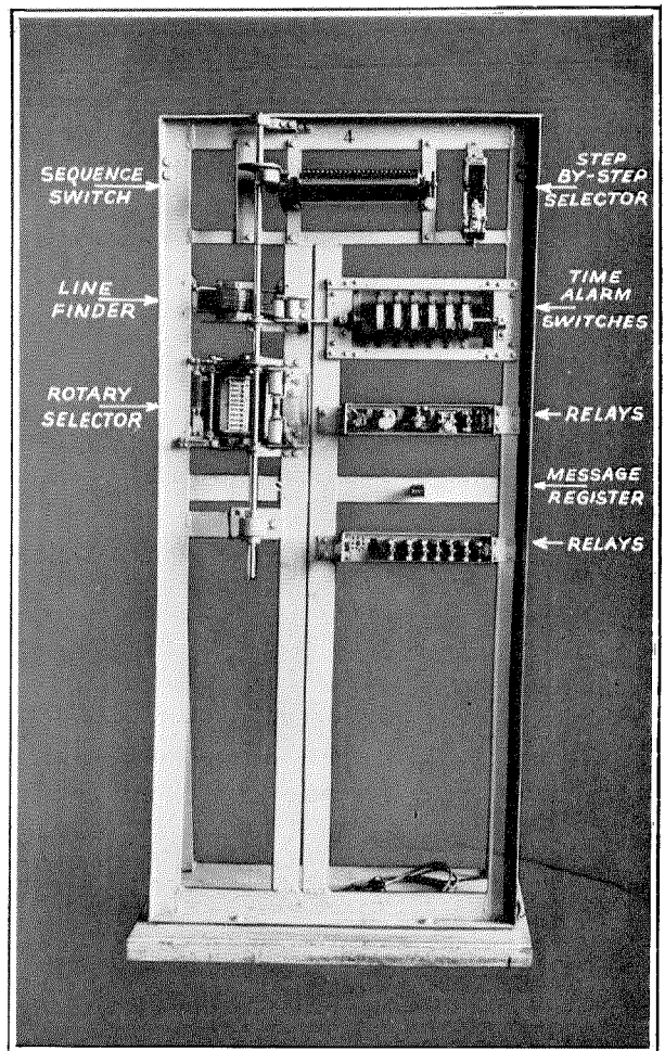
Figure 7—Apparatus Frame Used in Machine Adjustments Training.
