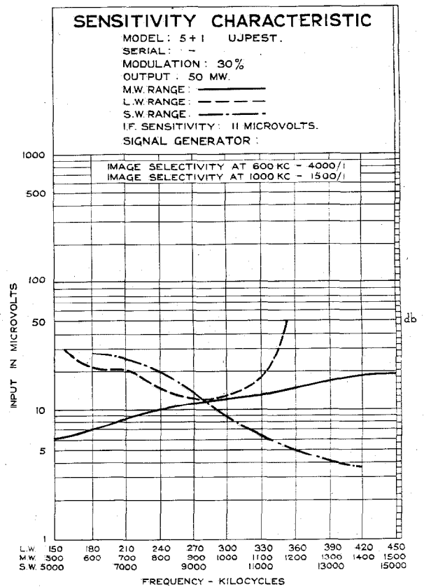
Figure 20—Sensitivity Characteristic of Standard Budapest 35 6-Tube (5+1) Radio Receiver.
