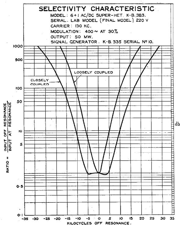
Figure 1—Selectivity Characteristic of Variable Selectivity Receivers. Curves Show Effect on Selectivity and Band Width of Operating the Selectivity Control Knob from Most Selective to Highest Fidelity Positions.
