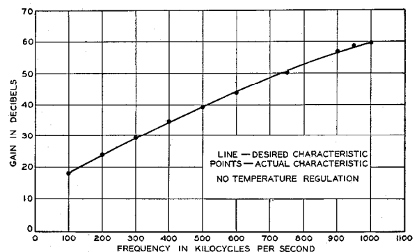
Figure 11—Gain of 1,000-kc. Repeater.
