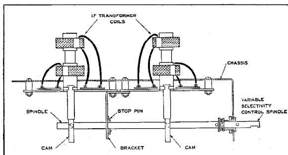
Figure 2—Sketch Showing Mechanics of Variable Selectivity
