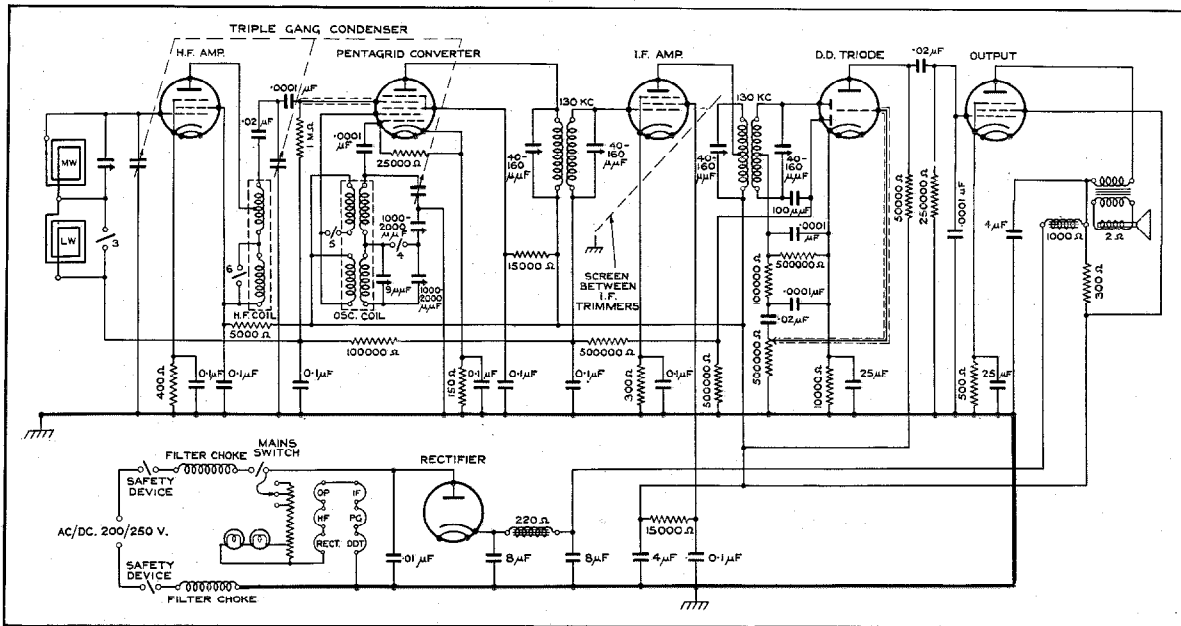
Figure 6—Schematic Diagram of K.B. 405 Transportable Receiver.
