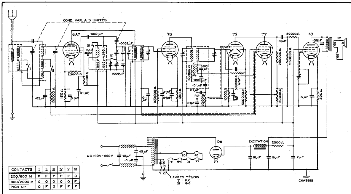
Figure 7—Schematic of Bell Tel. Mfg. Co. "Bell 6" 6-Tube (5+1) a-c. Receiver.
