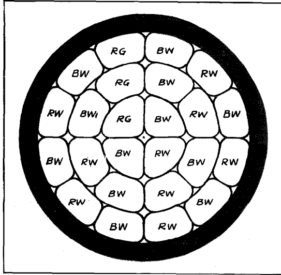
Figure 1—Lay-up of 101 Pair Units in 2424 Pair Telephone Cable
