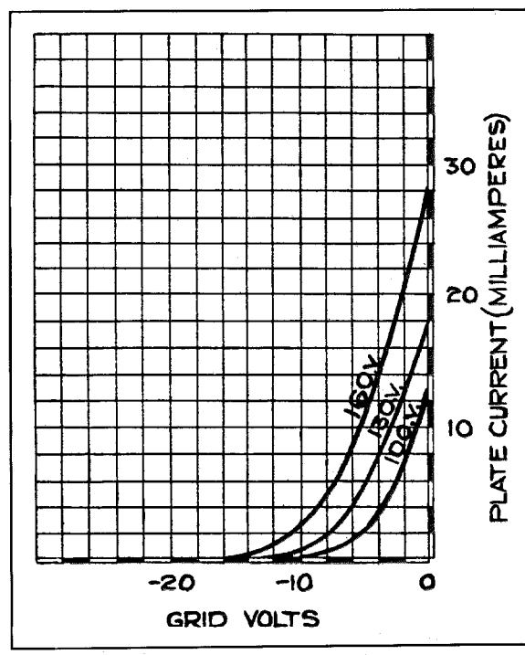
Figure 6—Characteristic Curves of the 4022-A Type Tube
