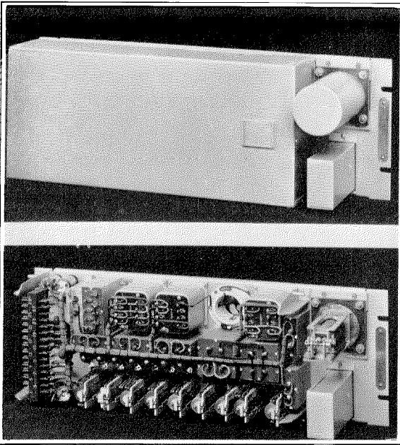
Figure 5—500 Cycle Ringer Panel
