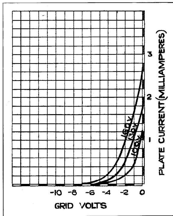
Figure 4—Characteristic Curves of the 4020-A Type Tube
