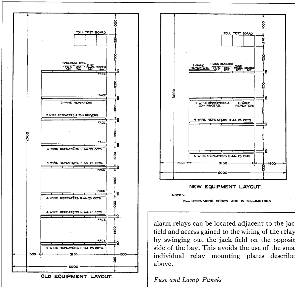
Figure 9—Specimen Floor Plans Comparing Old and New Equipments
