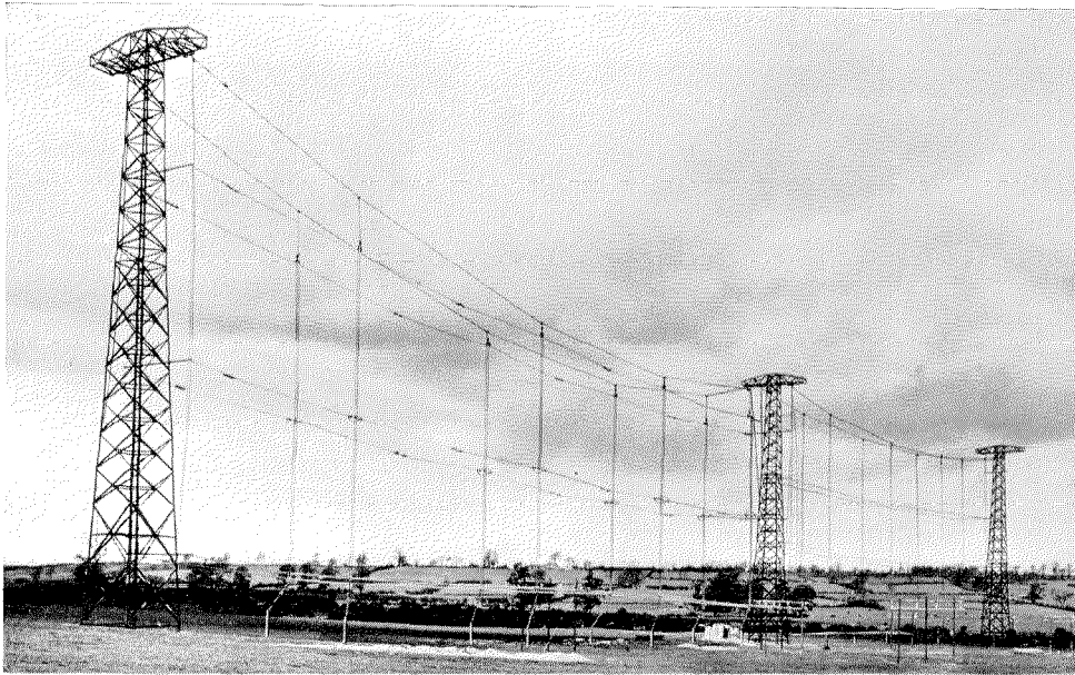
Figure 1—Typical Antenna Array at Rugby, England.
