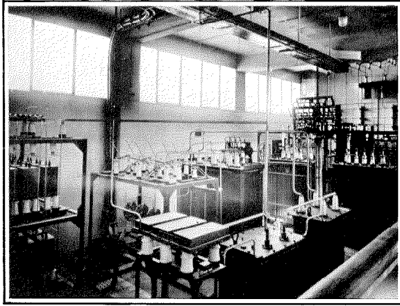
Figure 6—High Tension Enclosure in Basement
