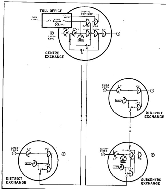
Figure 2—Typical Junction Diagram for Small Town and Environs (Uniform 4-Digit Closed Numbering)
