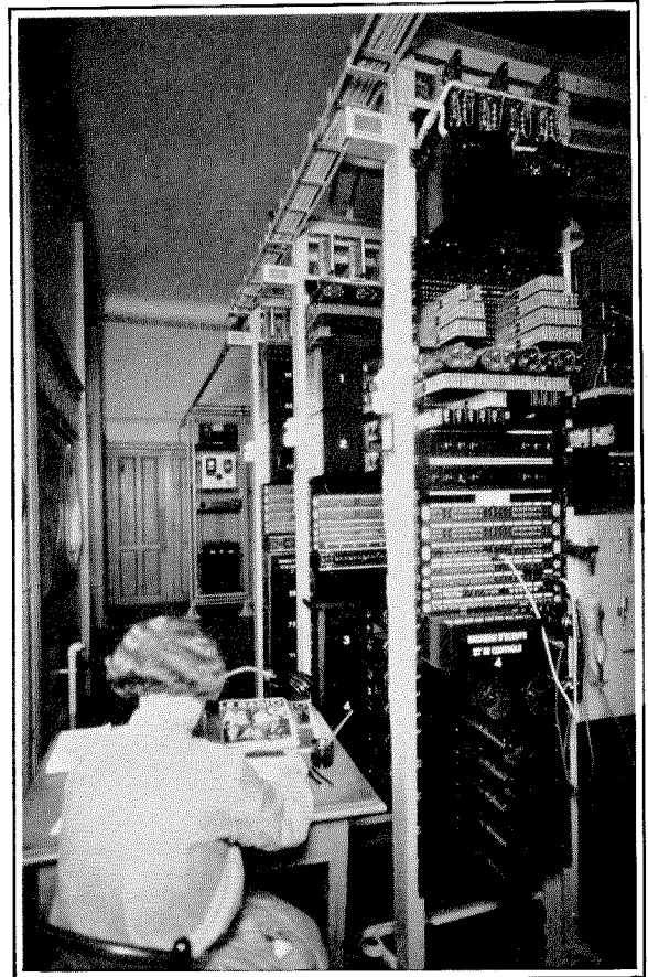
Broadcast Repeater at Lausanne Repeater Station
