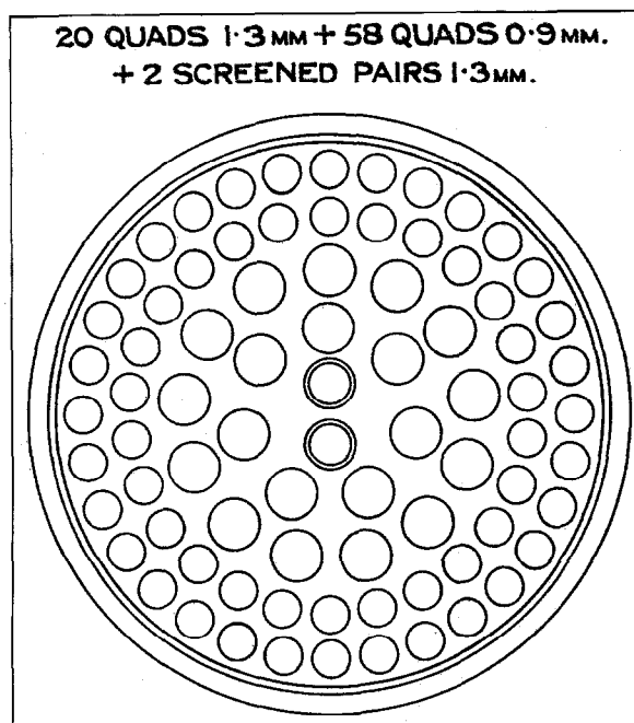
Figure 2—Typical Cable Lay-up Showing Location of Broadcasting Pairs
