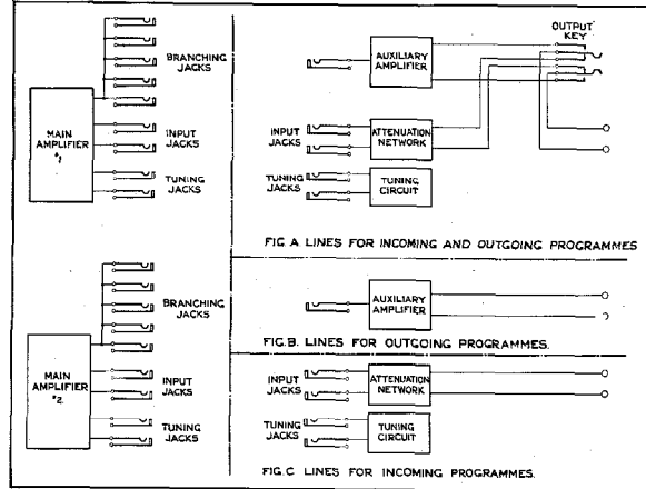
Figure 15—Switching Arrangements for Branching at a Station with a Large Number of Lines
