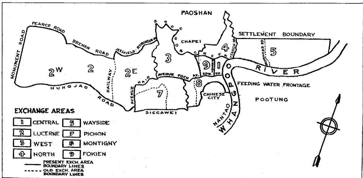
Plate No. 1—Conversion Programme 1930-32. Rearrangement of Exchange Areas
