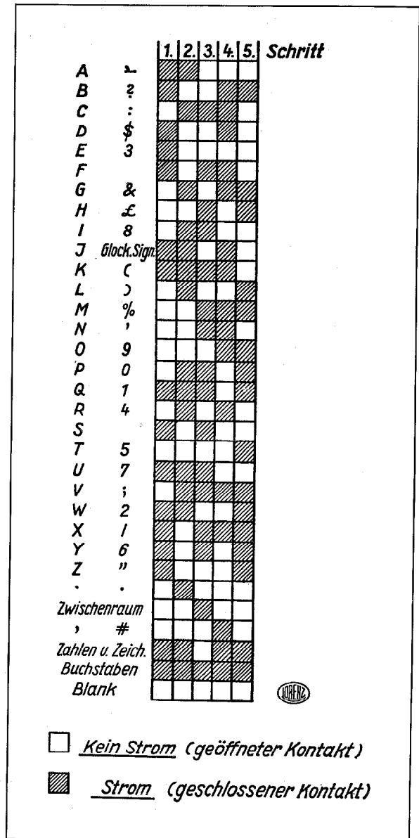
Figure 6—Five-Unit Murray Code
