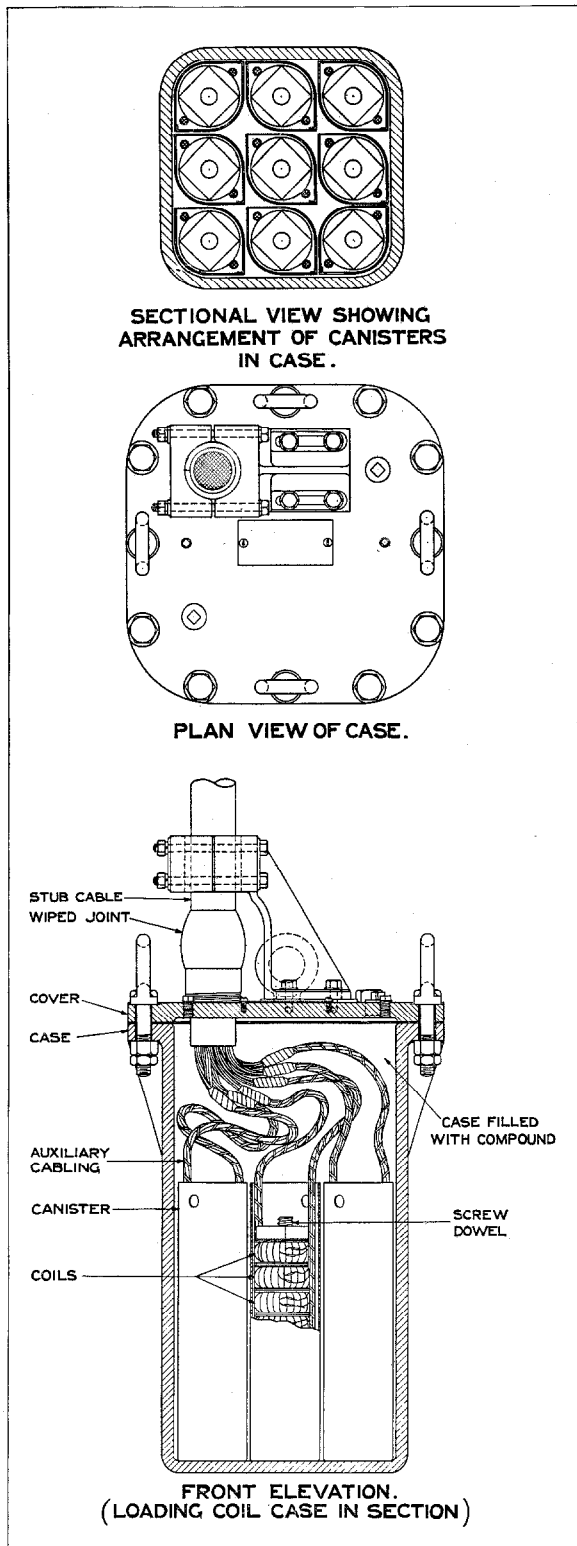
Figure 27—Stub Cable Type Loading Coil Case.
