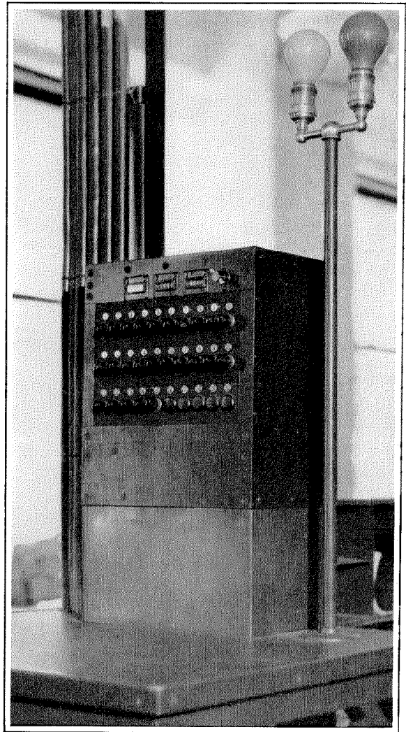
Figure 4—Supervisor's Control Cabinet.
