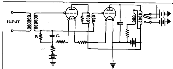
Figure 16—Schematic of Detector of Type 4.
