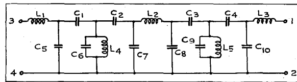
Figure 23—Receiving Filter Schematic.
