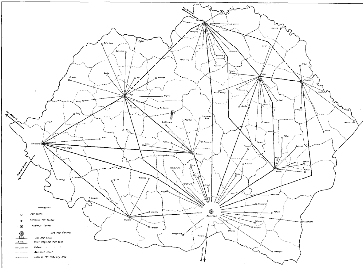
Figure 7—Final Toll Centering Plan for Rumania.
