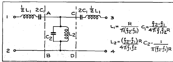
Figure 19—Prototype Band Pass Filter Section.
