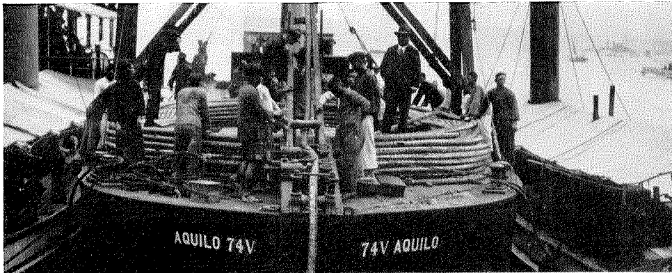
Figure 5—Submarine Cable on Lighter Ready to Start.
