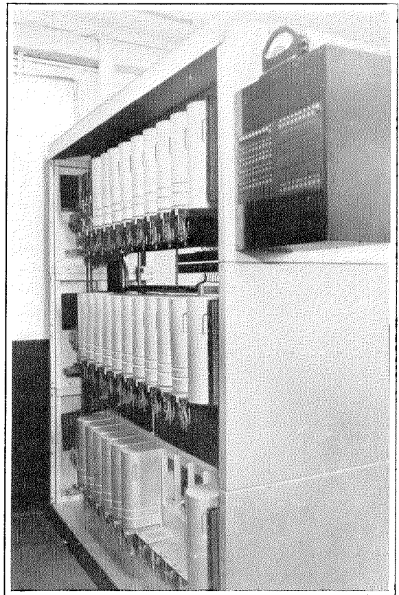
Figure 2—Switch Rack with Covers Removed and Line Jack Panel.
