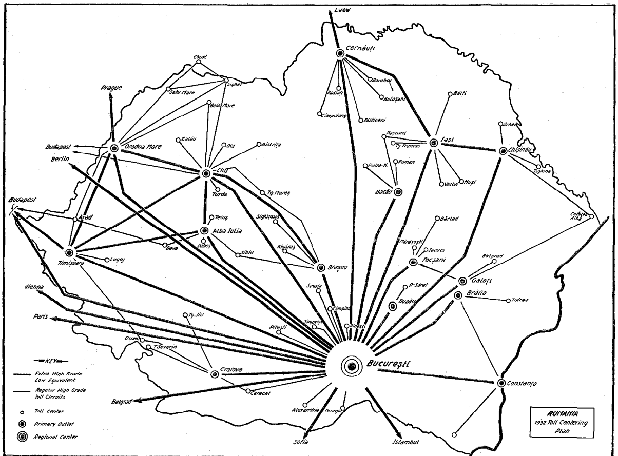
Figure 6—Provisional Toll Centering Plan for 1932.
