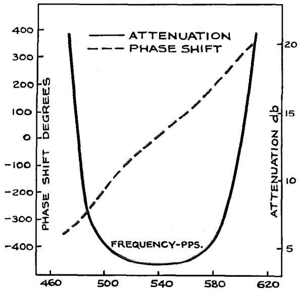
Figure 29—Attenuation and Phase Shift of Receiving Filter Flanked on Both Sides.
