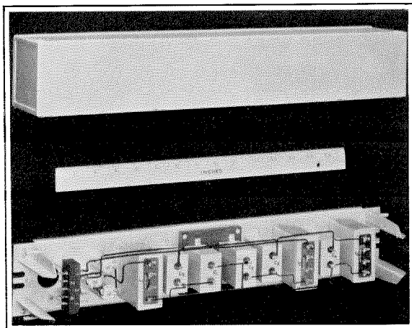
Figure 24—View of Sending Filter.
