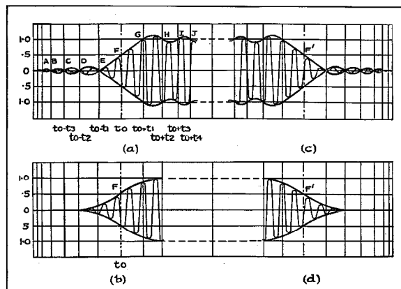
Figure 10-a, b, c, d—Oscillations Resulting From Positive and Negative Signals.
