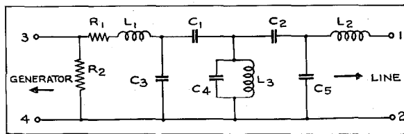
Figure 22—Sending Filter Schematic.
