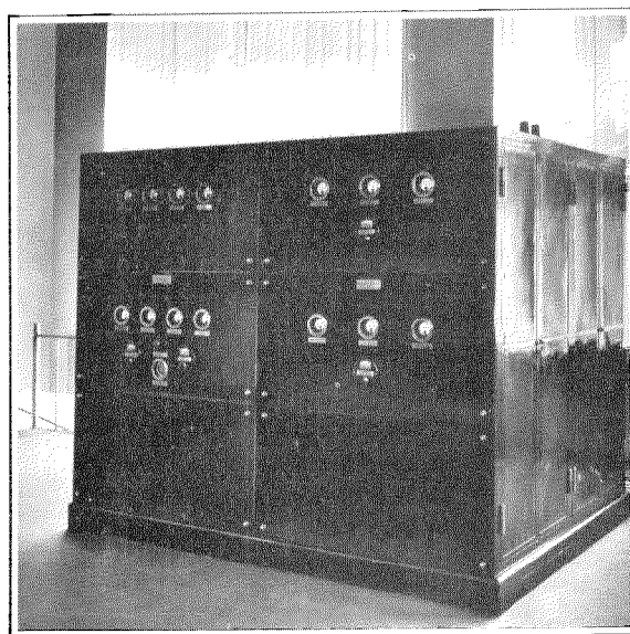
Figure 6—Oscillator-Modulator Unit.
