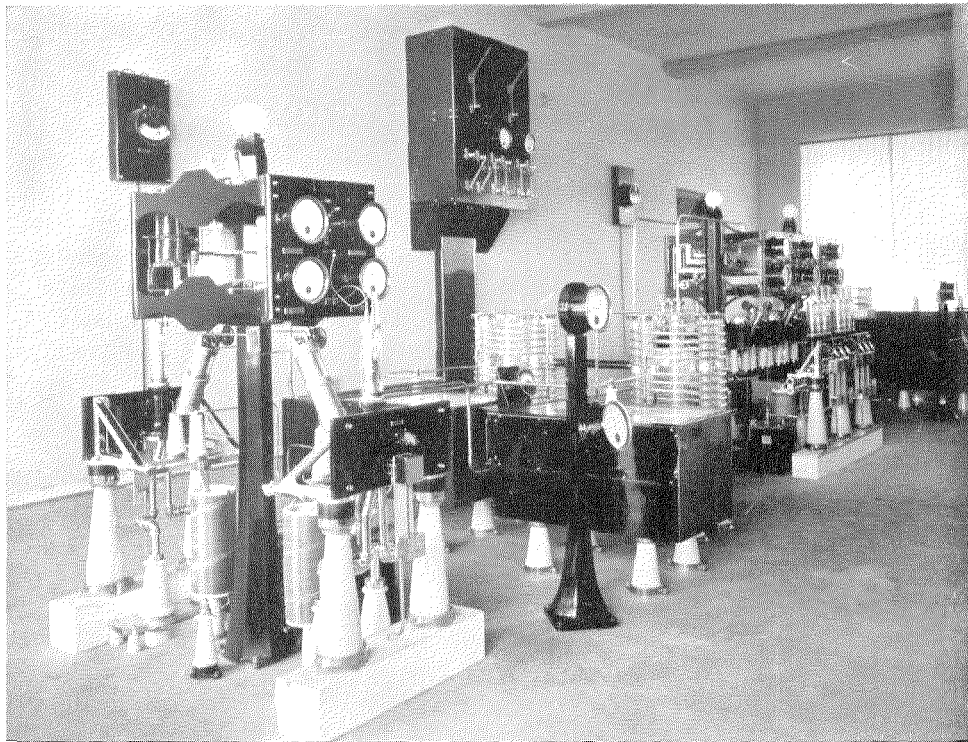
Figure 4—Power Amplifier from the Front, Looking Right.
