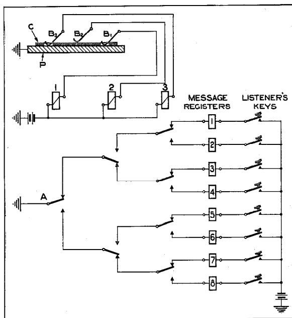
Figure 2—Simplified Schematic of Automatic Device for Recording, Correcting, and Analysing Articulation Results.
