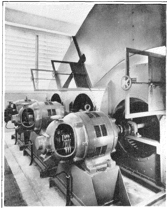
Figure 17—Motor Driven Fans for Air Blast Cooler.
