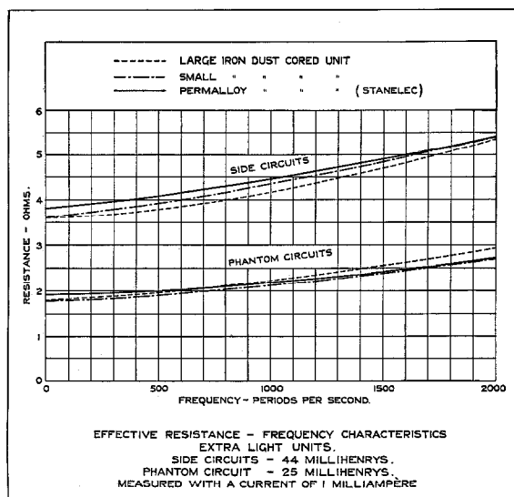
Figure 9—Effective Resistance—Frequency Characteristics Extra Light Units.
