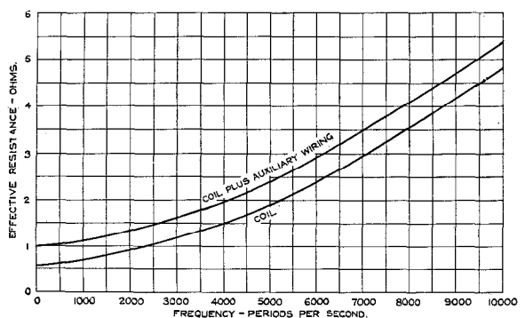
Figure 18—Effective Resistance—Frequency Characteristic of a 15.5 Millihenry Coil for Loading a Music Transmission Circuit. Measured With a Current of 1 Milliampere.
