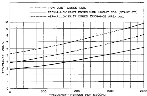
Figure 17—Effective Resistance—Frequency Characteristics of 88 Millihenry Coils as Used for Exchange-area Loading. Measured With a Current of 1 Milliampere.
