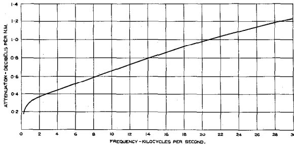
Figure 7—Attenuation-frequency Curve.
