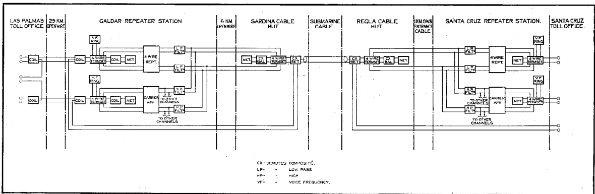
Figure 3—Ultimate Circuit Layout Diagram for the Tenerife-Gran Canaria Cable.
