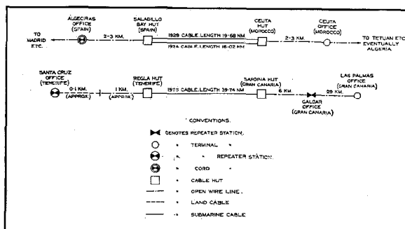
Figure 2—Layout of Cable Systems.
