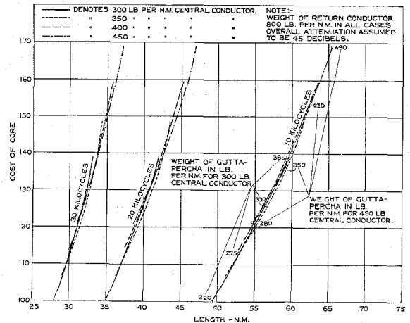
Figure 3—Curves Showing the Effect of Varying the Weight of Gutta-percha While Keeping the Weights of the Central and Return Conductors Fixed.
