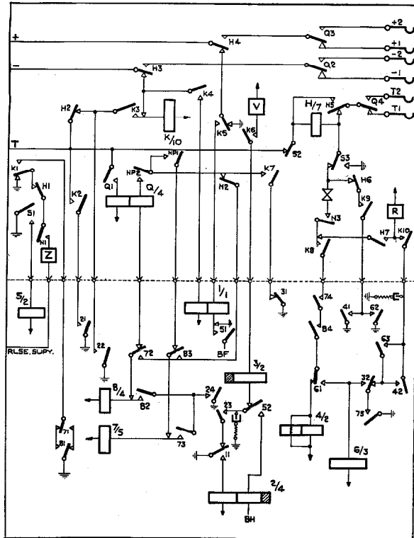
Figure 2. Switching and Absorbing Selector
