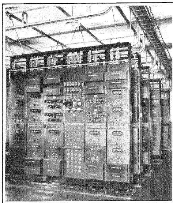
Carrier Terminal Equipment.
