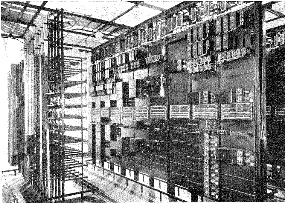
Figure 7—Combined Distributing Frame and Repeater Rack, Florence.
