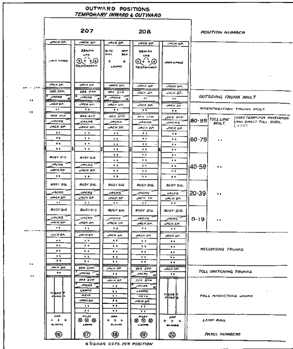
Figure 14—Typical Face Equipment, Outward.
