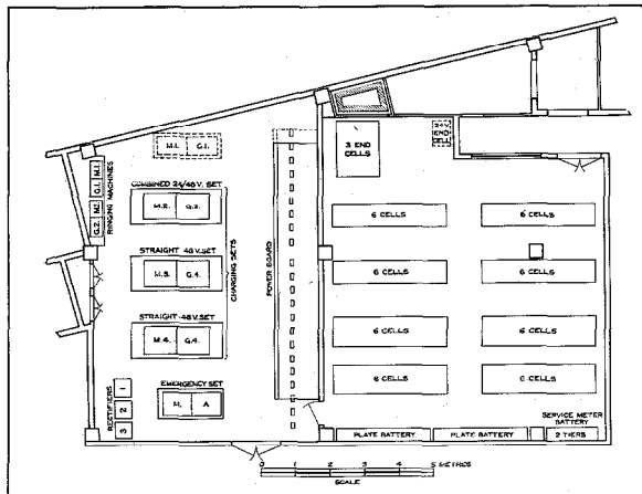
Figure 7—Floor Plan of Battery and Machine Rooms for Cataluna.
