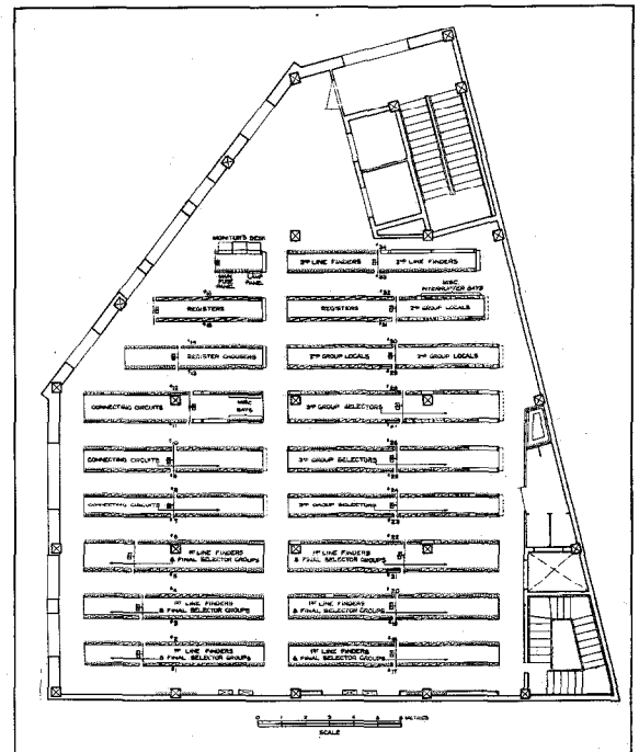
Figure 8—Layout of Automatic Equipment, Fourth Floor.
