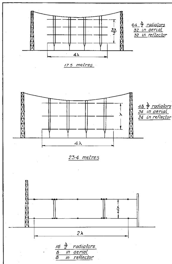
Figure 2—Ship-and-Shore Arrays—Rugby.
