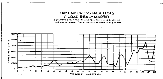
Figure 9—Far End Crosstalk Tests, Ciudad Real-Madrid Disturbing Circuit No. 64 at Ciudad Real Terminated by 620 Ohms. Listening on Circuit No. 60 at Madrid Terminated by 620 Ohms.
