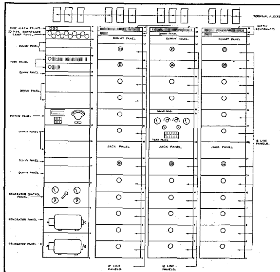
Figure 6—Typical Installation for 34 Lines—Rack Layout.
