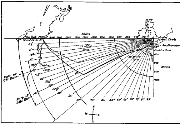
Figure 1—Southampton-New York Sea Route. -----Most Northern Route. ———Most Southern Route. Divergence of Sea Routes from Rugby-New York Great Circle.
