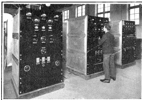
Figure 5—The Transmitter, Rugby Station.
