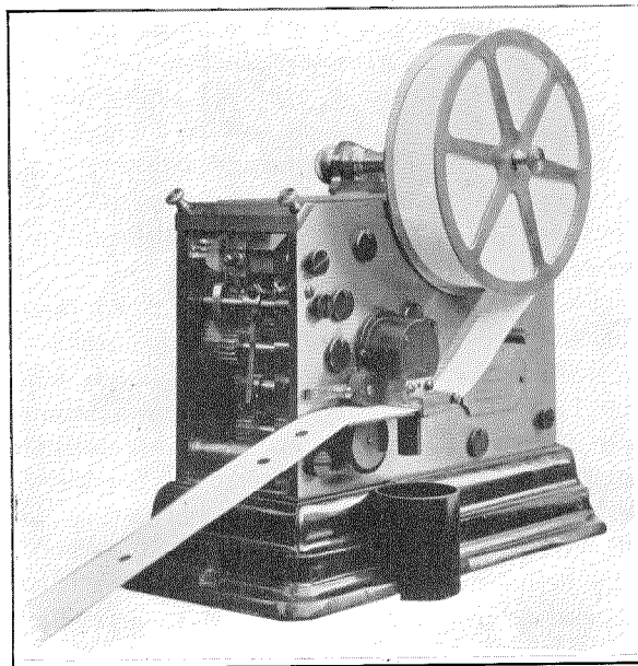
Figure 10—Single Circuit Register.
