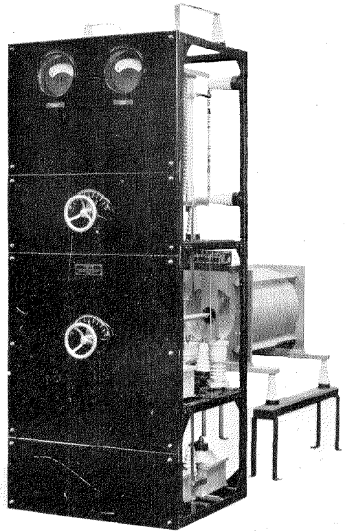
Figure 11—Tuning Unit.
