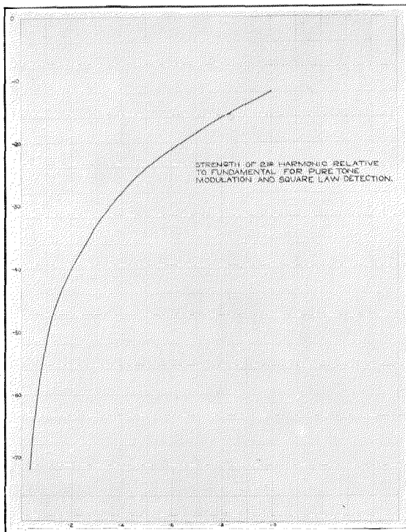
Figure 1—Strength of Second Harmonic.
