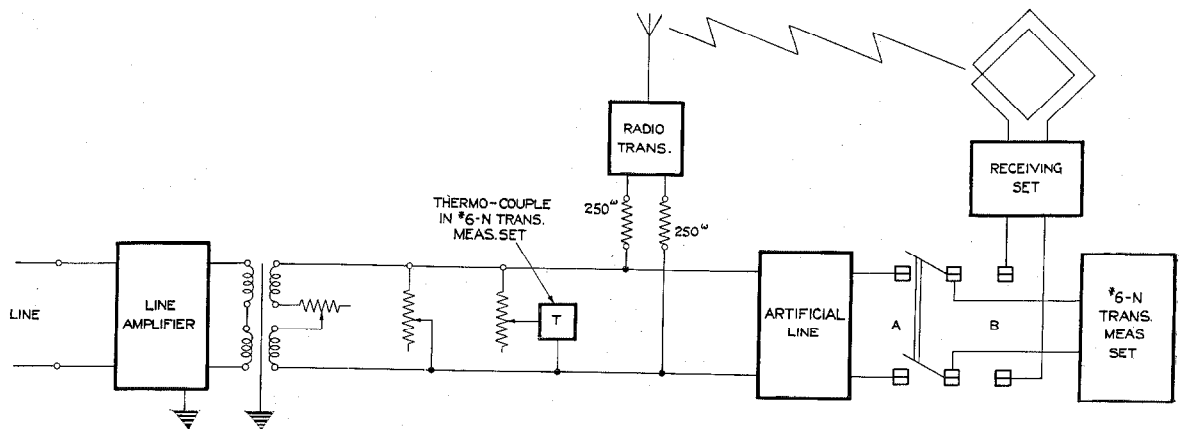
Figure 7—Circuit for Response Measurements on Radio Transmitter.
