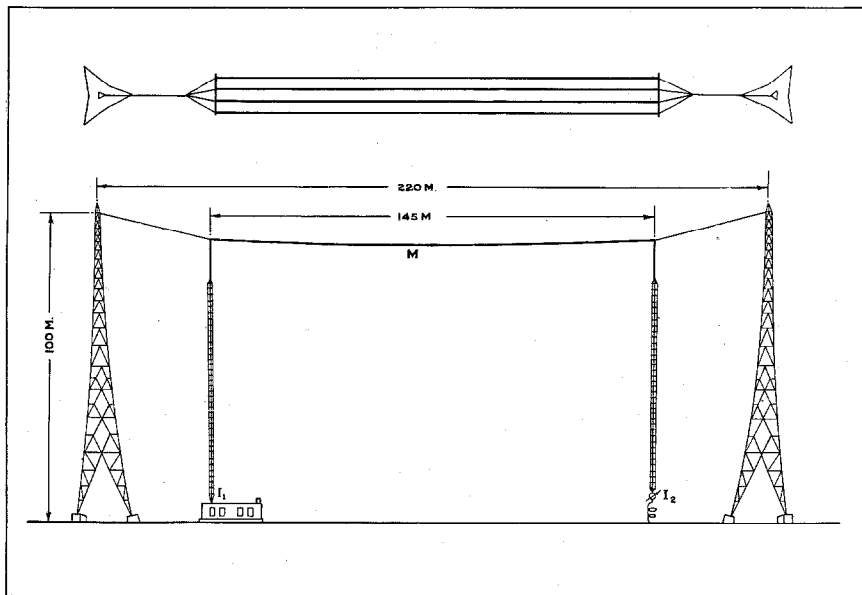
Figure 6—Antenna System.
