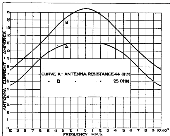
Figure 7—Overall Band-width Curves of Kalundborg Transmitter.
