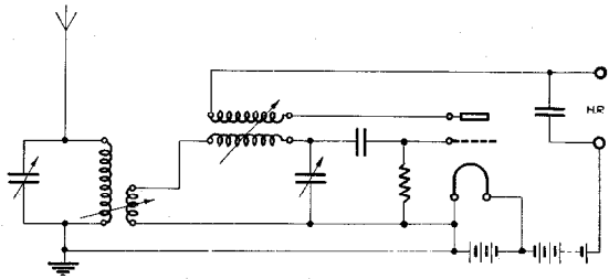
Figure 6—Simple Reaction Amplifying Circuit.
