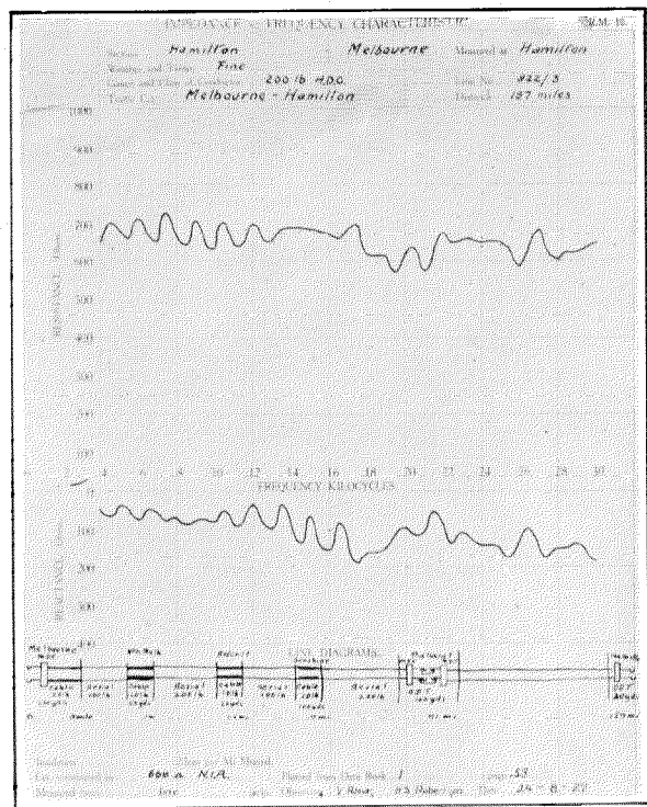
Figure 6—Impedance-Frequency Characteristics of the Melbourne-Hamilton Circuit Measured from the Hamilton Terminal.
