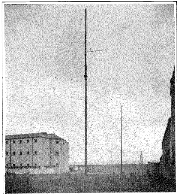
L-type Aerial at Cork Broadcasting Station.
