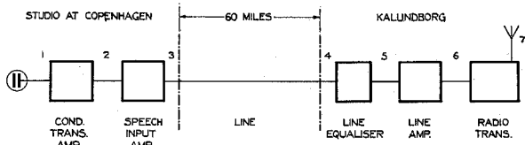
Figure 1—Component Parts of Transmission Path.
