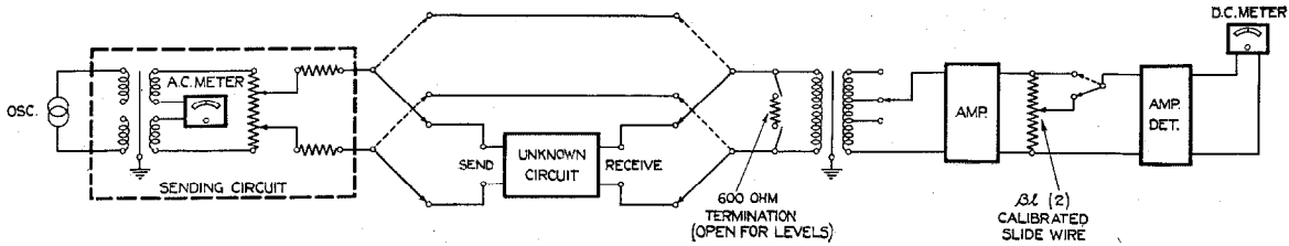
Figure 9—Schematic of No. 74006-G Transmission Measuring Set.
