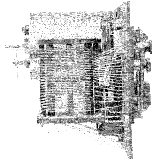
Figure 3B—Master Oscillator (Interior view).
