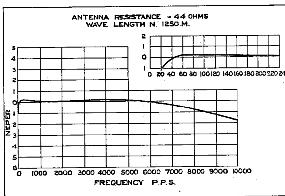
Figure 8—Frequency Characteristic Curve of Kalundborg Transmitter.
