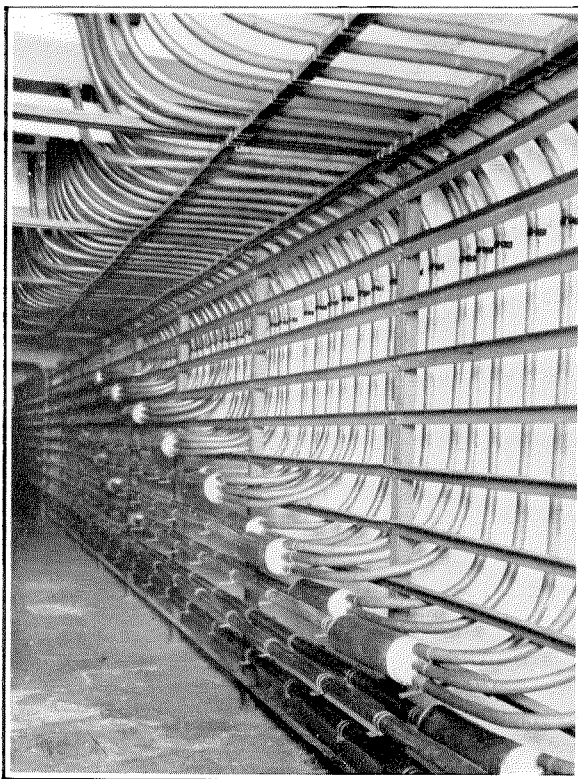
Figure 7—Cable Vault in Jordan Automatic Exchange, Madrid.
