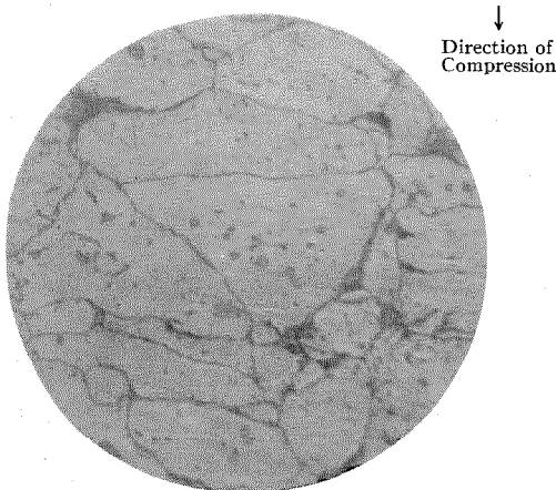
Figure 6B—Photomicrograph of the Cross Section Shown in Figure 6A but Enlarged 400 Times Instead of 100
