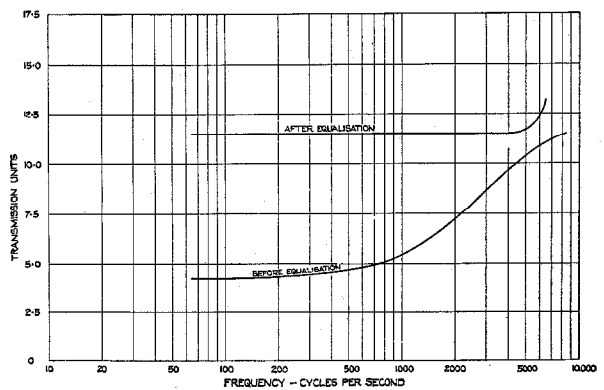
Figure 3—Attenuation of Line between National Theatre (Prague) and Studio (Prague), before and after Equalisation
