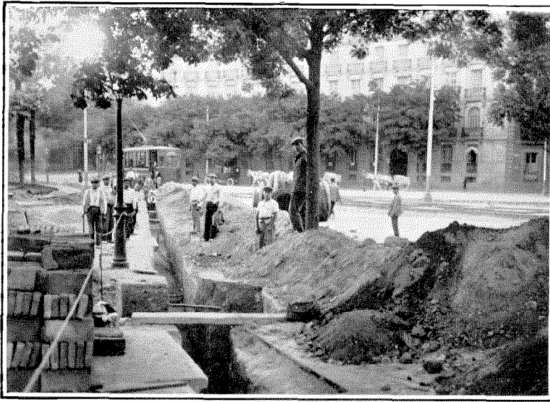
Figure 5—Running a Trench of the Underground Telephone Cable System across the Plaza Colon, Madrid. The variety of pipes and bare cables of other subterranean systems crossing at various levels may be noted.
