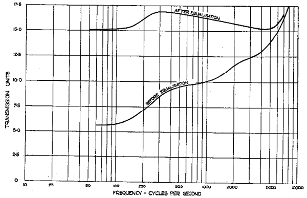
Figure 2—Attenuation of Pair No. 2524 of the Telephone Line between Brno and Prague, before and after Equalisation
