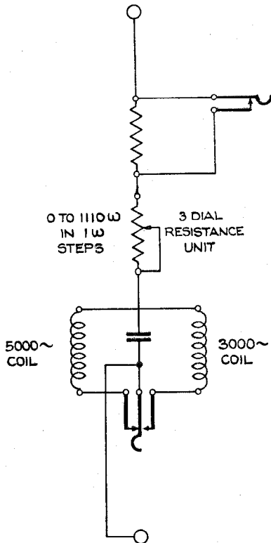
Figure 5—Circuit of Standard No. 1-A Equaliser
