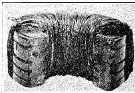
Figure 3—Loading Coil with Ring Form of Winding in Which Part of the Core and Winding Has Been Removed
