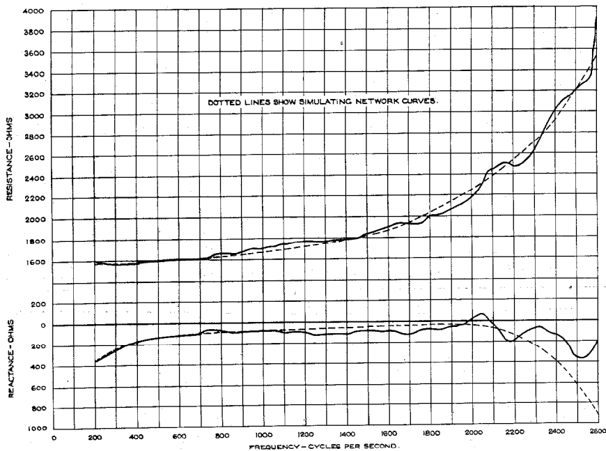
Figure 18—Impedance Curves—0.9 mm. H-177-107 Side Circuit
