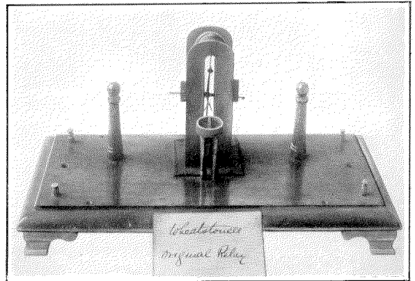
Figure 14—Original Relay
