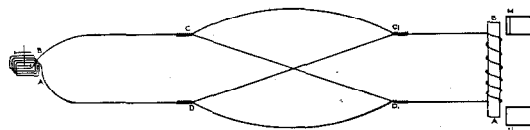
Figure 10—Christie's Single Helix Four-wire Resistance Balance
