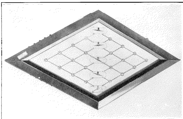
Figure 16—Five-needle Telegraph
