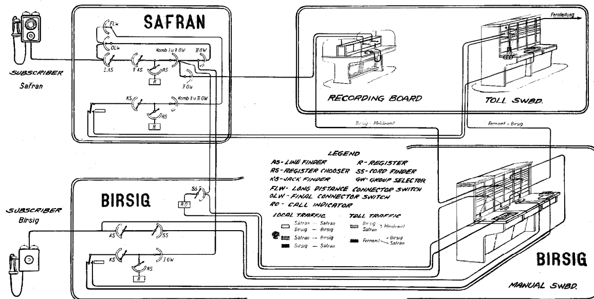
Figure 4—Diagram of Connections of Demonstration Model for Basle Area
