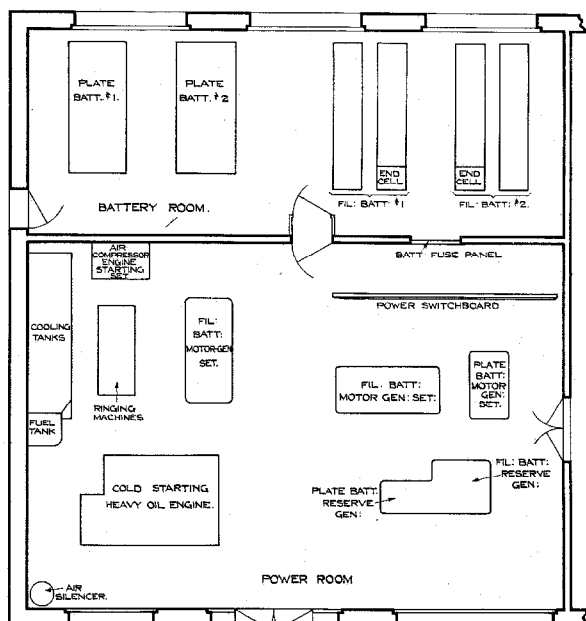
Figure 15—Floor Plan of Power and Battery Rooms
