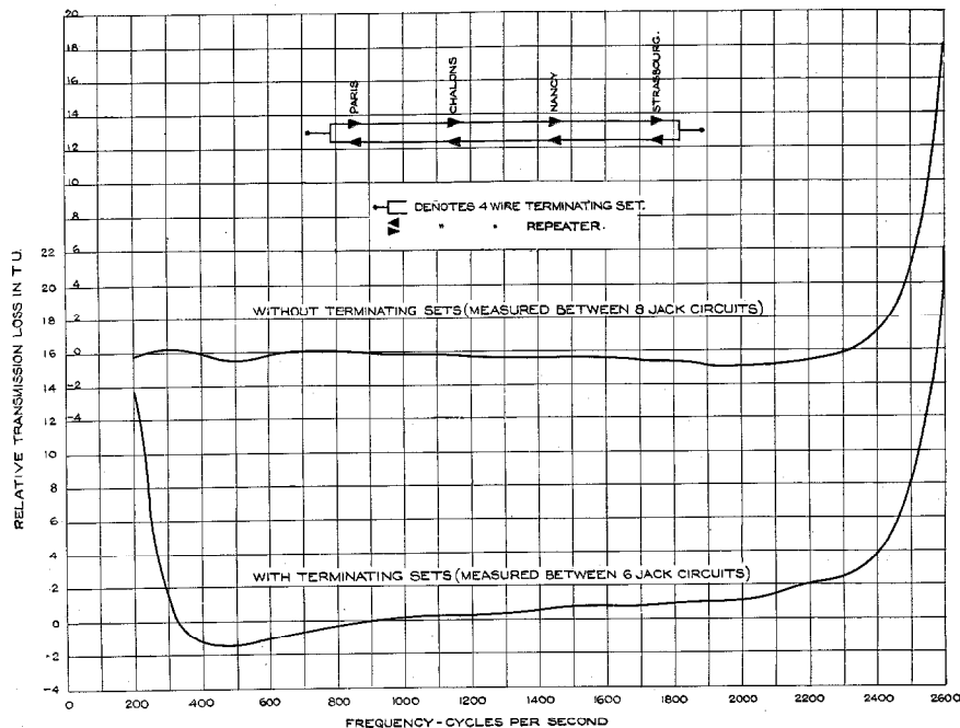
Figure 27—Overall Transmission Frequency Characteristics—0.9 mm. 4-wire H-177-107 Side Circuit
