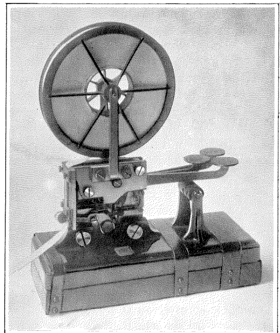
Figure 15—Tape Puncher
