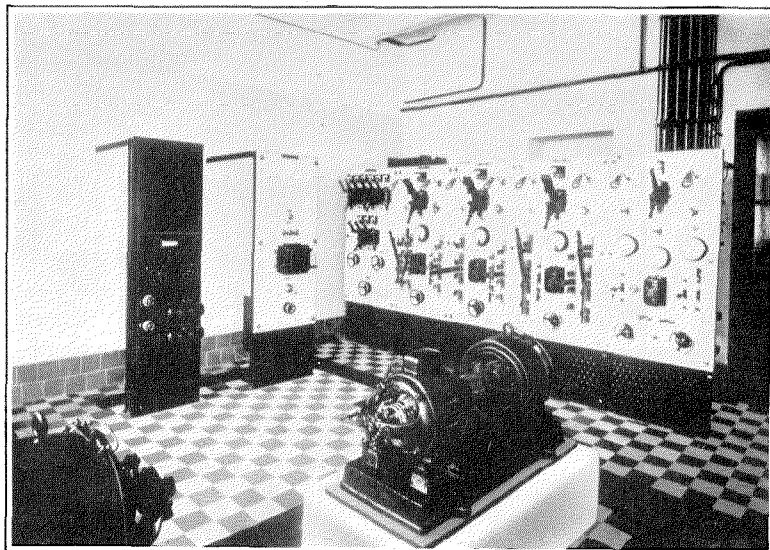
Figure 14—Power Board
