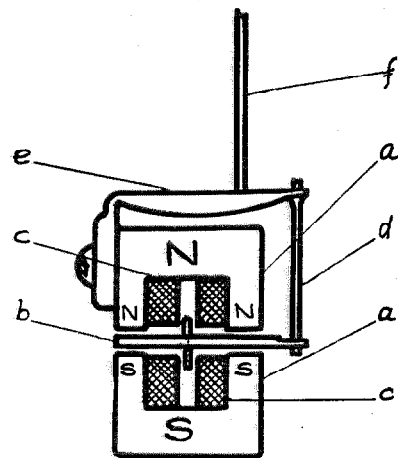
Figure 1—Balanced Armature Mechanism
