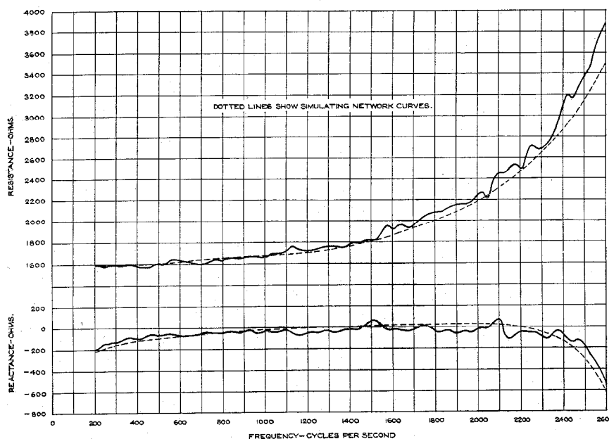
Figure 16—Impedance Curves—1.3 mm. H-177-107 Side Circuit
