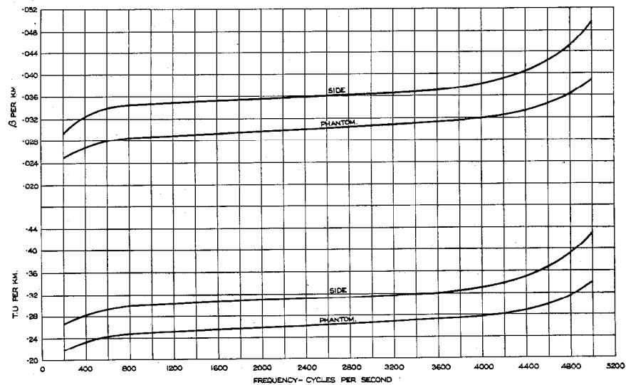
Figure 24—Attenuation—Frequency Curves—0.9 mm. H-44-25 Side and Phantom Circuits
