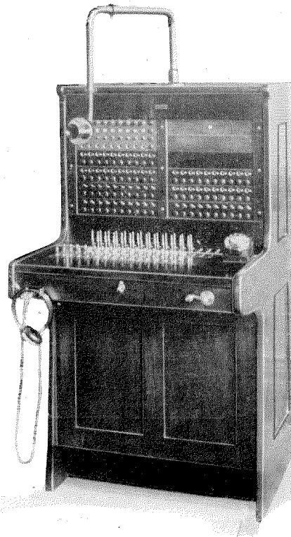
Figure 8—Attendant's Cabinet
