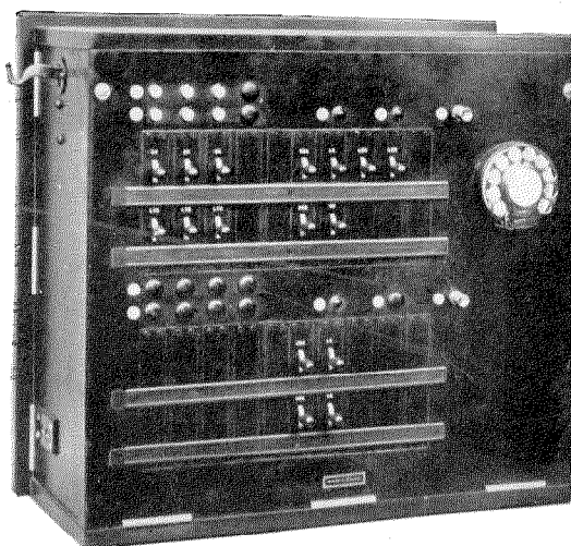
Figure 12—Attendant's Box with Dial
