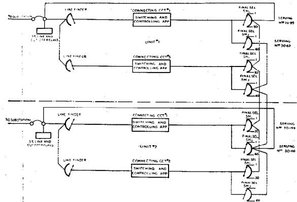
Figure 5—Junction Diagram 70-Line PBX Arranged for Local Calls Only
