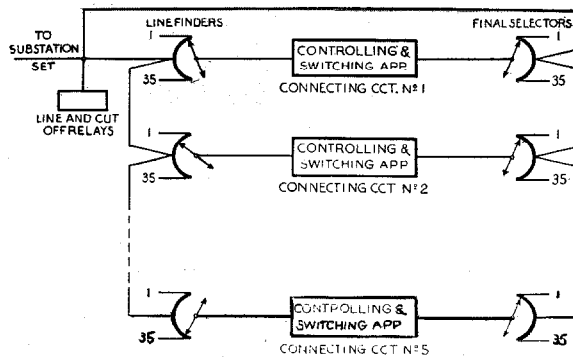
Figure 4—Junction Diagram 35-Line PBX Arranged for Local Calls Only
