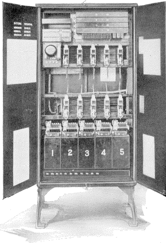
Figure 2—35-Line Unit—Front View
