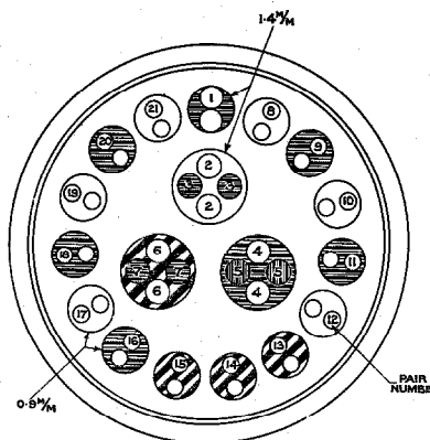
Figure 3c—Cross Section of Cable, Falköping-Göteborg Section
