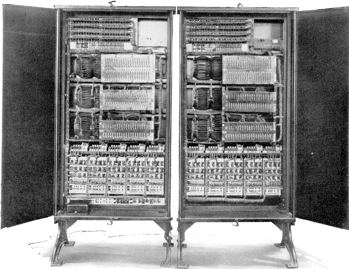
Figure 3—70-Line Unit—Rear View
