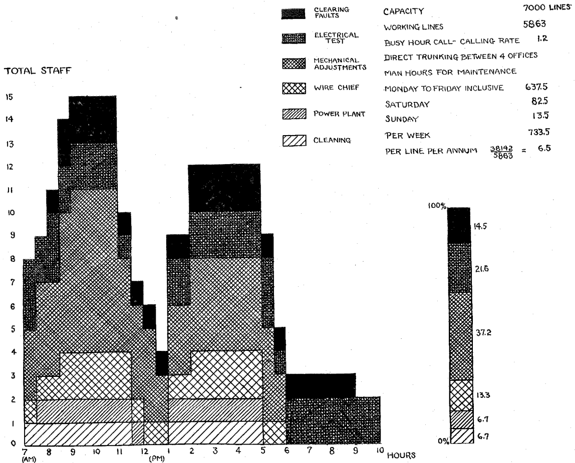
Figure 19—Maintenance Chart—Marnix
