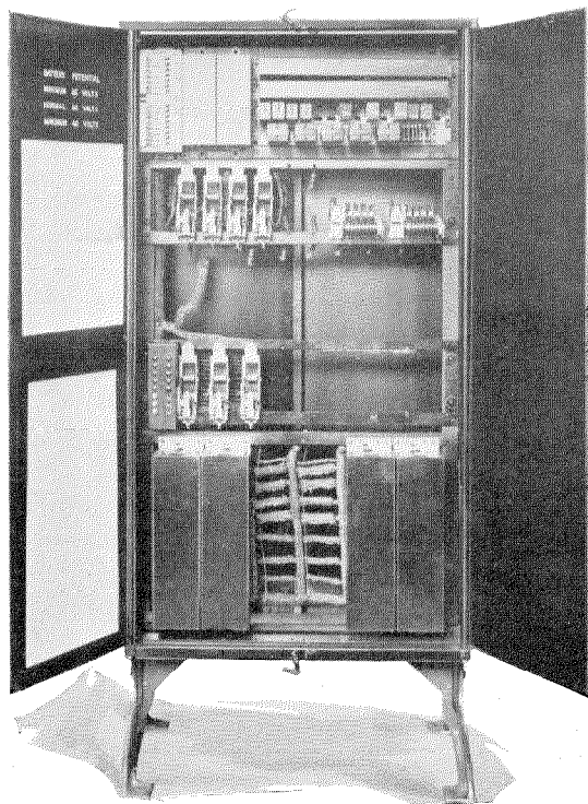
Figure 13—Junction Unit Associated with Attendant Box
