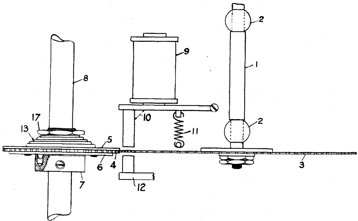
Figure 3—Gear Drive—Elevation
