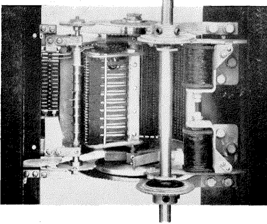
Figure 11—No. 7009 Selector Mounted on Bay
