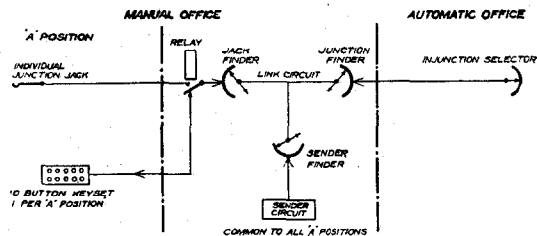
Figure 37—Direct Trunking
