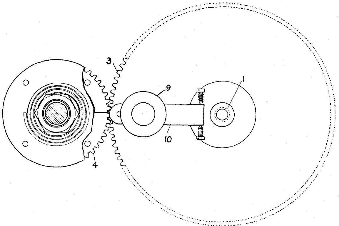
Figure 4—Gear Drive—Plan
