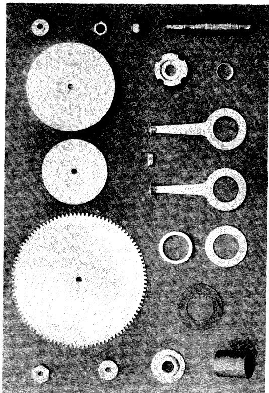
Figure 7—No. 7002 Finder—Brush Carriage Details
