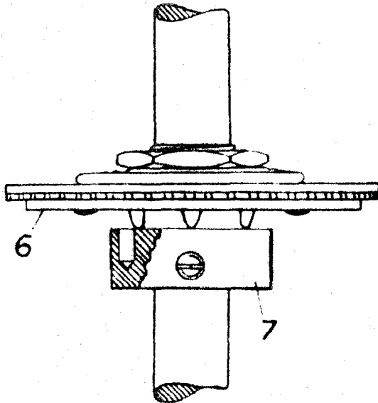
Figure 5—Gear Drive—Driving Gear Raised
