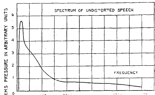
Figure 3—Pressure-Frequency Spectrum of Undistorted Connected Speech
