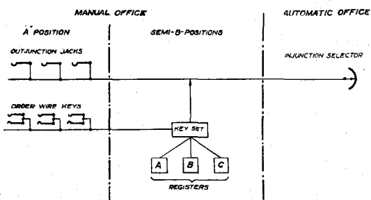
Figure 36—Order Wire Trunking
