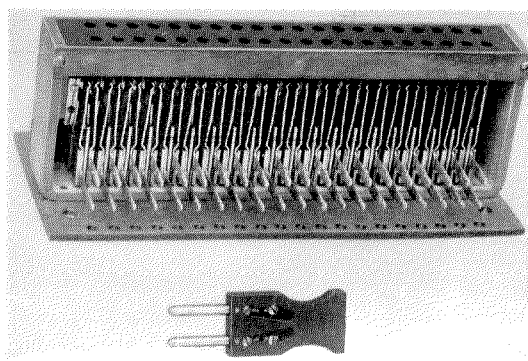
Figure 23—MDF Test Jack—Bottom or Cable Side
