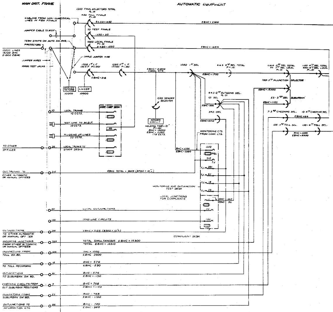
Figure 21—Junction Diagram—Typical 10,000 Line Office
