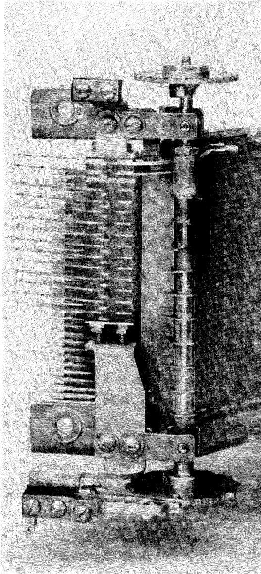
Figure 14—No. 7009 Selector Trip spindle and Terminal Block
