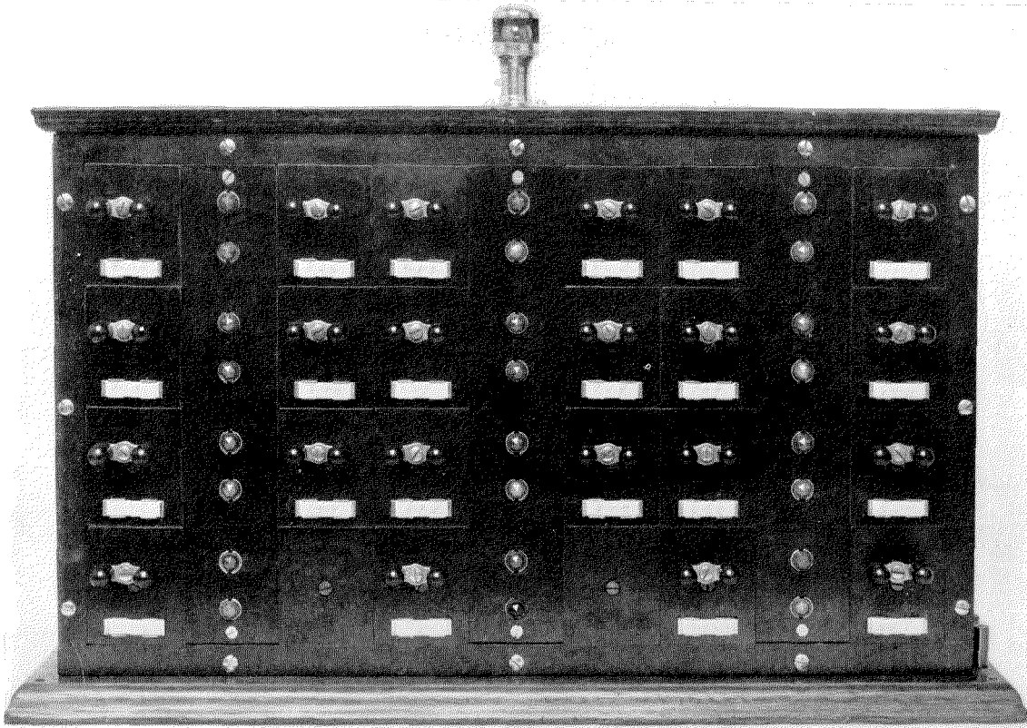
Figure 2E—Selector System, Dispatcher's Station Equipment—Key and Lamp Cabinet Located on Dispatcher's Desk. Contains Two Keys and Two Lamps for Each Unit Supervised. One of These Keys Will Open While the Other Will Close a Circuit Breaker. One Lamp (Green) Indicates the Open Position, the Other Lamp (Red) Indicates the Closed Position of the Unit Supervised
