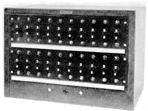
Figure 1G—Distributor and Cable Systems—For Control and Indication—Dispatcher's Control Cabinet. Contains One Key and Two Lamps for Each Switch to be Supervised
