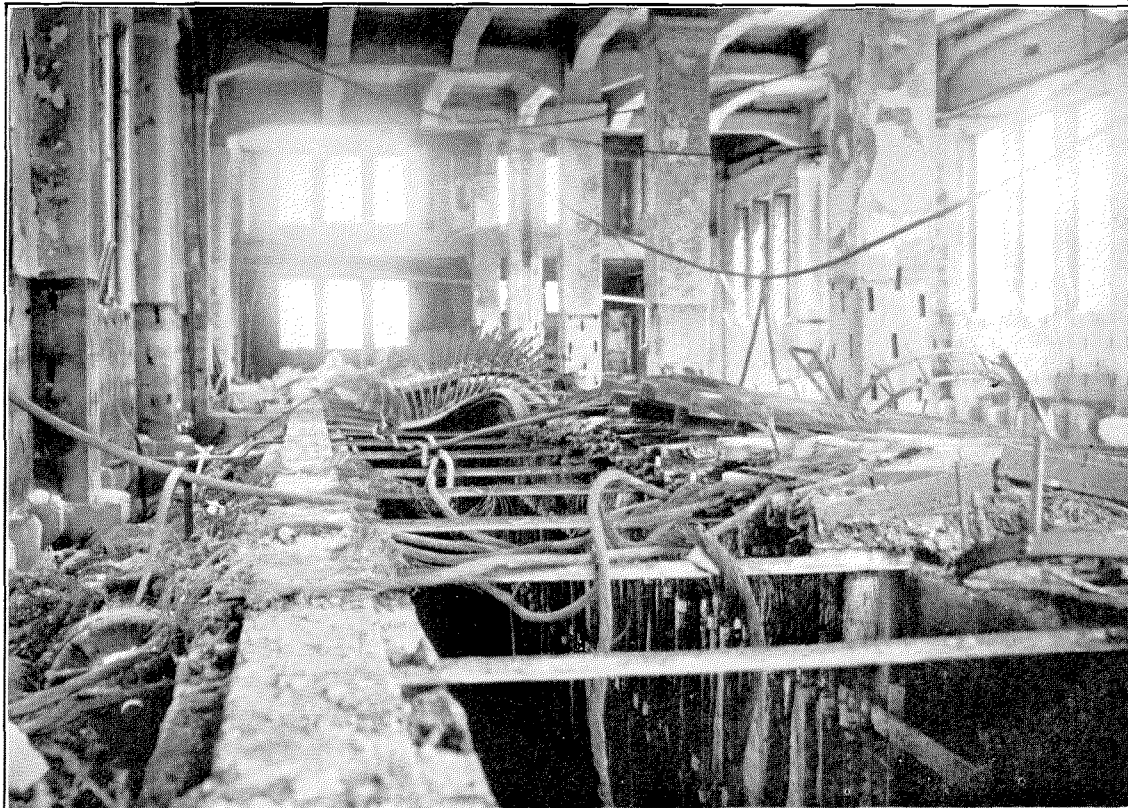
Figure 16—Ruins of M. D. F. and Office Manhole After Fire in Telephone Central Ginza, Tokio
