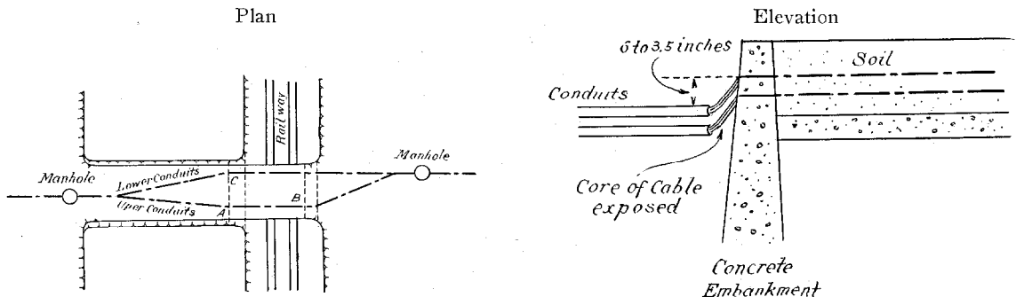
Figures 14 and 15—Damages to Cables on Public Bridges, Tokio
