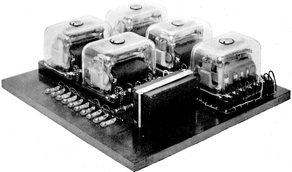
Figure 2B—Selector System, Dispatcher's Station Equipment—Indication Shelf—Contains the Receiving Apparatus Required for the Indication of Four Switches
