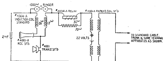
Figure 2—British Post Office Reference Circuit
