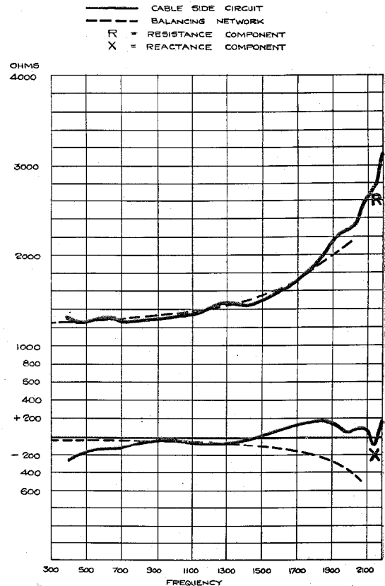
Figure 17—Impedance Curve for Cable Side Circuit
