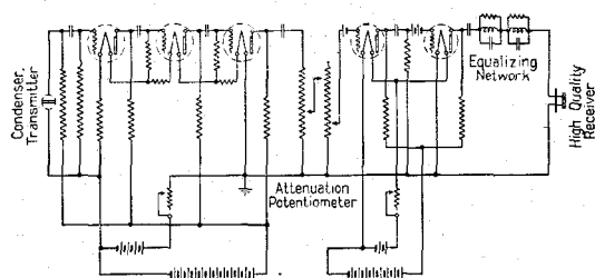
Figure 1—Circuit of High Quality Telephone Reference System
