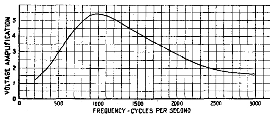
Figure 20—Amplification Characteristic, 201-A Input Transformer
