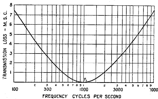
Figure 10—Transformer Connecting a Resistance to a Negative Reactance Ideal transformer of impedance ratio R/X at frequency " F_1 " = 1000 cycles
