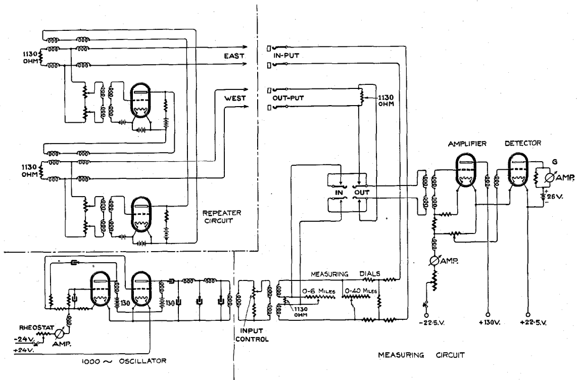
Figure 25—Measurement of Repeater Gain
