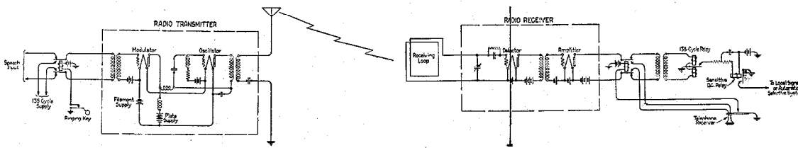
Figure 1—Simplified Diagram of Basic System for 135-Cycle Signaling
