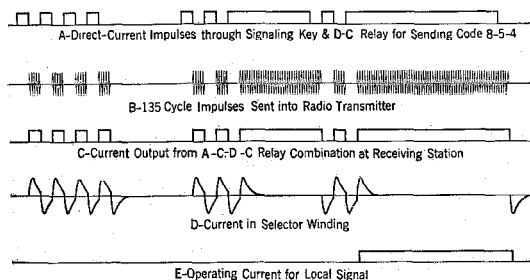
Figure 13—Form of Transmitted and Received Currents in Operation of Selective Signaling System
