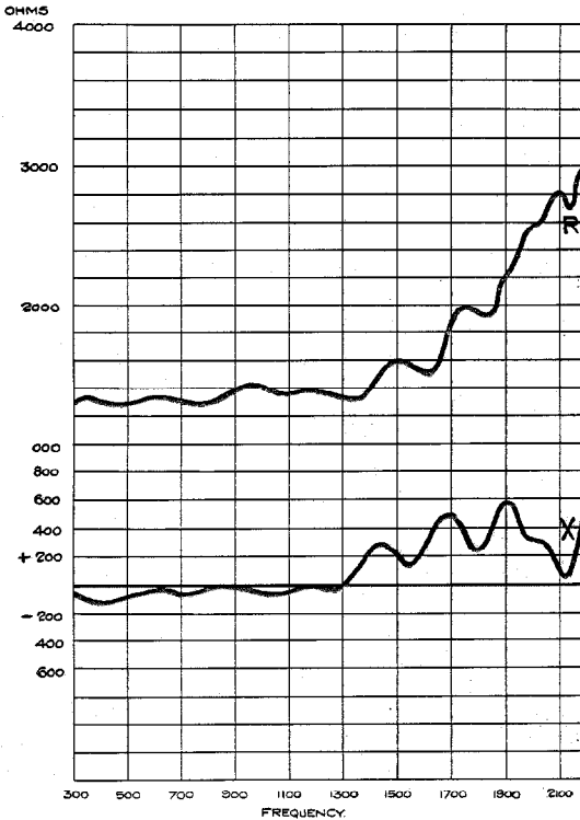
Figure 15—Impedance Curve for Cable Side Circuit
