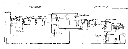
Figure 12—135-Cycle Selective Signaling System—Circuit Arrangement of Receiving Apparatus
