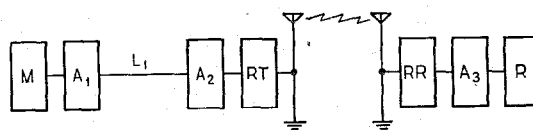
Figure 3—Schematic Diagram of Radio Broadcasting System
