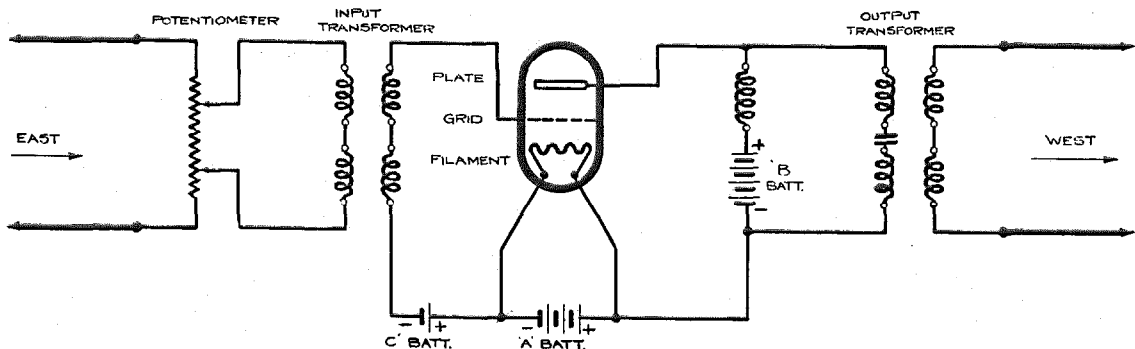
Figure 3—The Principle of Amplification
