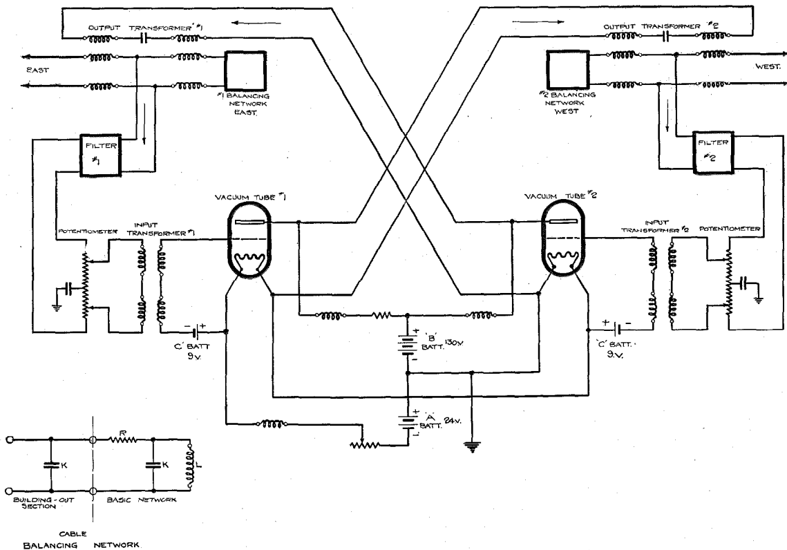
Figure 4—22-Type Repeater
