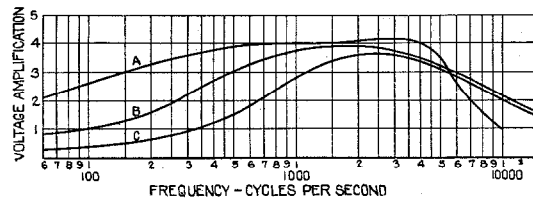
Figure 14—Voltage Amplification of Input Transformers of Different Mutual Impedances
