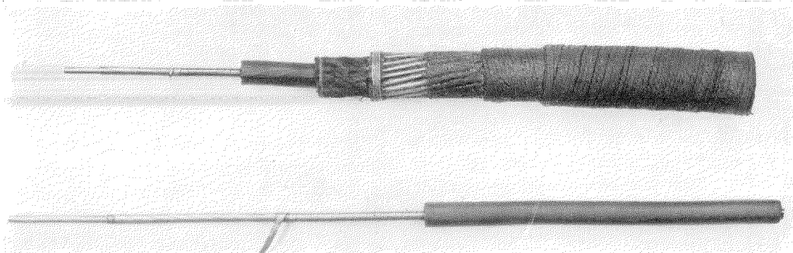
Permalloy Loaded Type Cable
