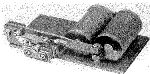
Figure 8—Structure of Vibrator for Interrupter
