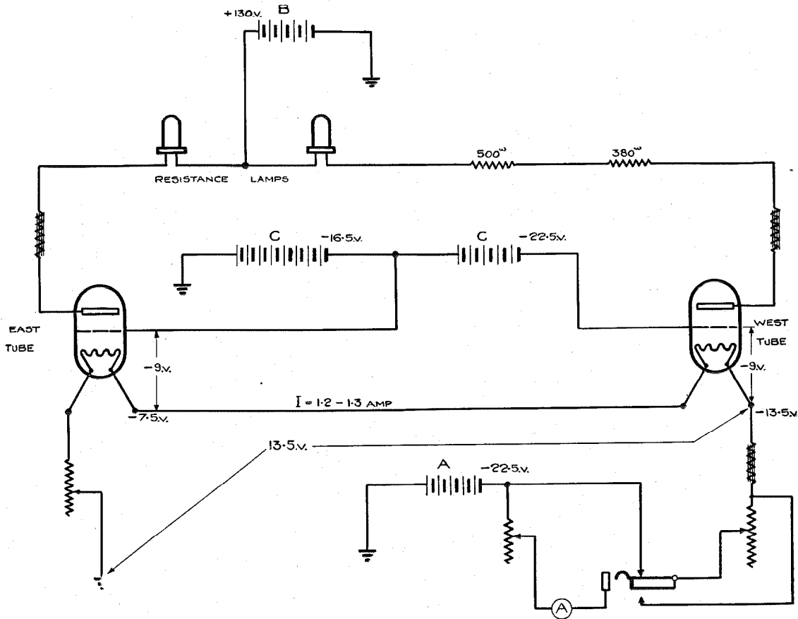
Figure 24—Battery Connections
