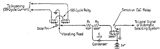
Figure 3—Secondary Circuit of 135-Cycle Relay
