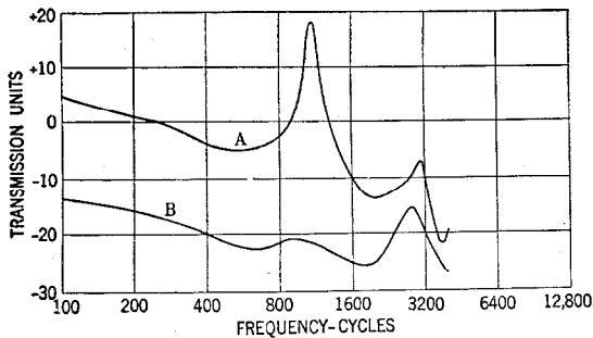
Figure 9—Frequency Response Characteristics of Telephone Receivers
