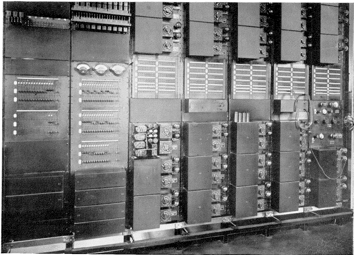
Figure 20—Repeater Rack
