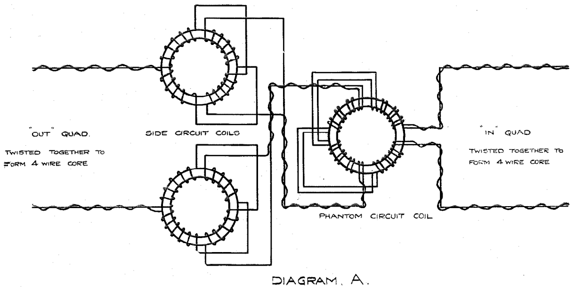
Figure 9—Splicing Plan
