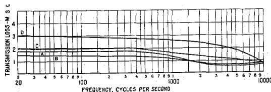
Figure 9—Transformers Operating Between a Resistance and a Positive Reactance
