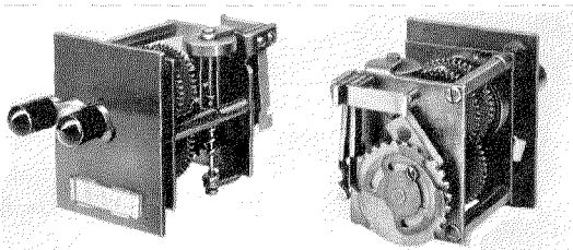
Figure 14—Code Sending Key for Particular Station
