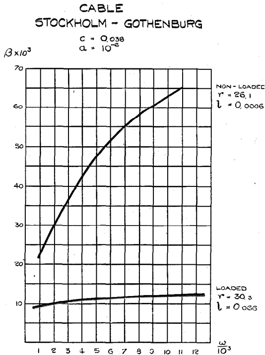
Figure 1b—Attenuation Curves
