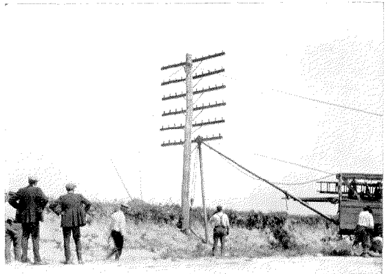
Figure 3—Derrick in Position to Pull Pole Out of Ground
