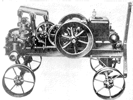
Figure 17—Enclosed Discharge Diaphragm Pump. Capacity One Barrel per Minute
