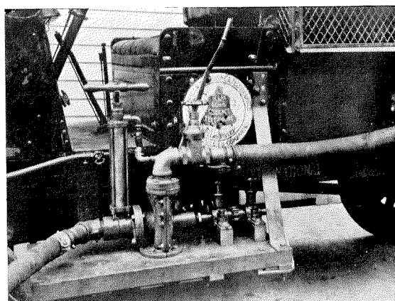
Figure 19—Centrifugal Pump Mounted on Underground Cable Placing Truck
