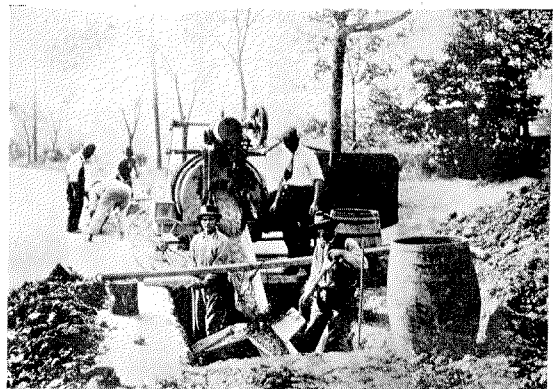
Figure 14—Pouring Concrete Manhole. Note 4-way Chute for Uniform Distribution
