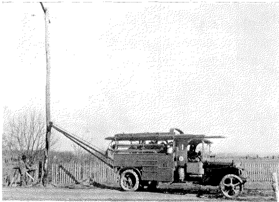
Figure 2—Erecting Pole at Distance from Truck, One Derrick Member on Ground
