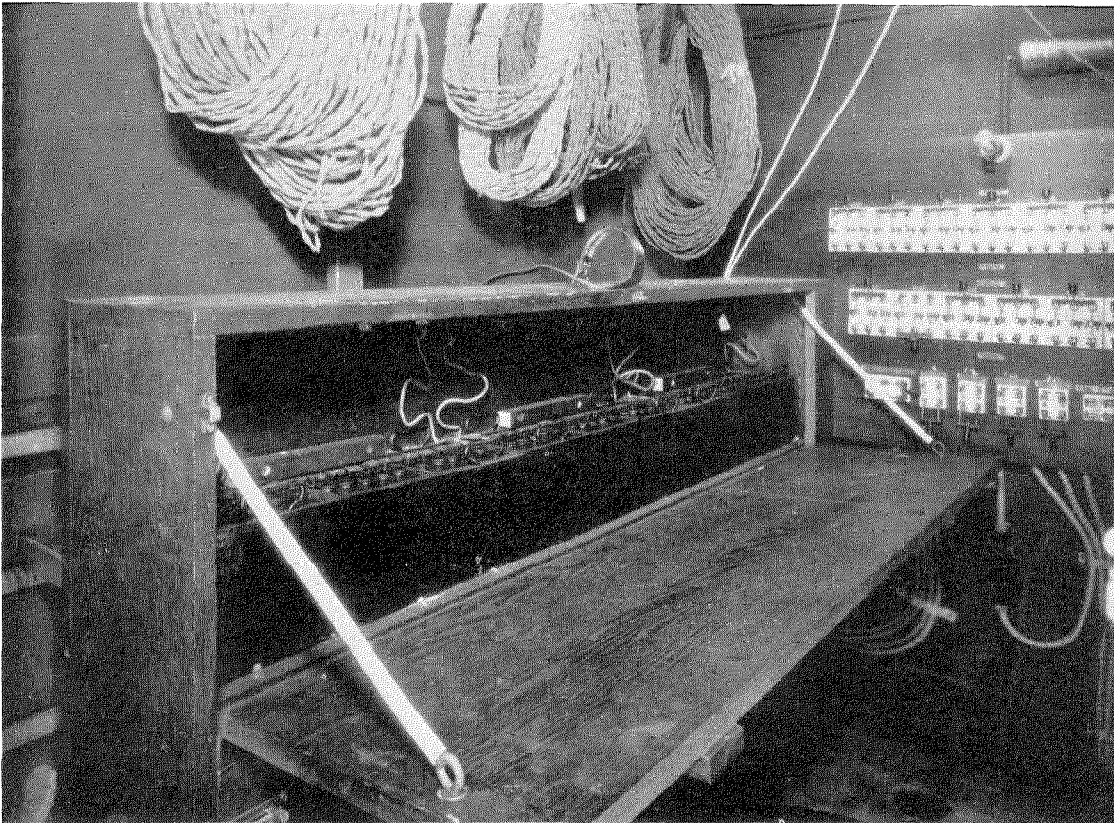
Fig. 3. Mobile Public Address System—Storage Battery Equipment
