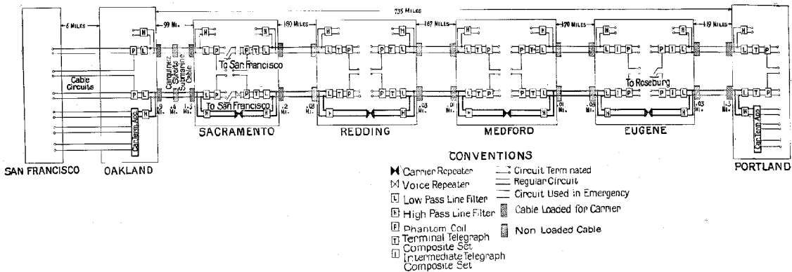
Fig. 6—Oakland-Portland Carrier Telephone System
